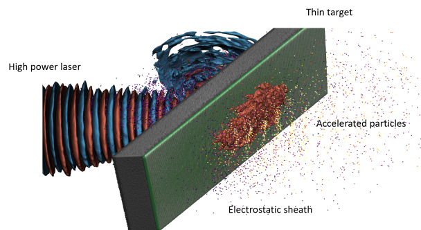
Figure 2: Illustration of 3D particle-in-cell simulation of TNSA mechanism following high-power laser impact on a thin, dense, target.
