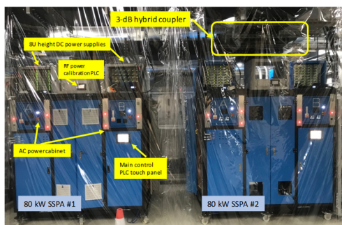
Figure 4: Two SSPA towers are practically RF power combined within the plastic shielding room for better temperature isolation and control by the air conditioner.
