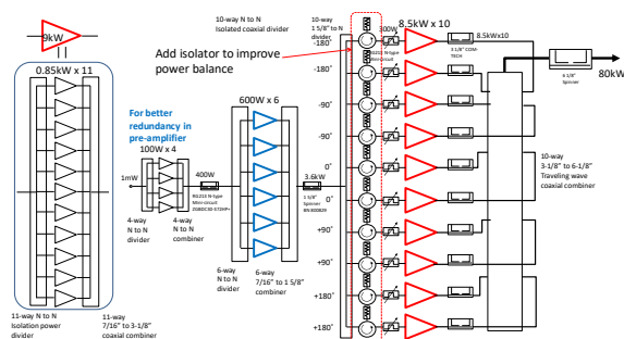
Figure 2: The schematic of redundancy improved 80 kW SSPA tower.
