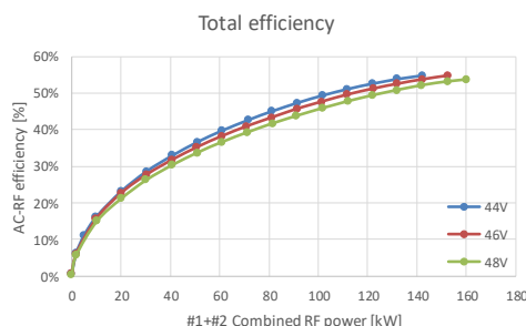
Figure 5: the AC-RF conversion efficiency as a function of output RF power in different DC voltage settings for 2-way combination of 80 kW SSPAs.
