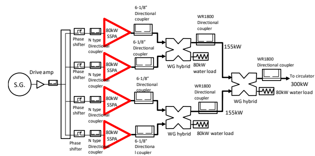
Figure 1: The topology of 300 kW fully solid-state transmitter.
