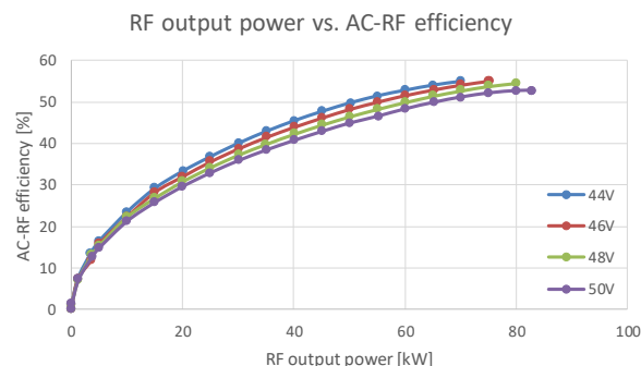
Figure 3: The AC-RF efficiency of 80kW SSPA tower as a function of RF output power by different Drain voltage settings.
