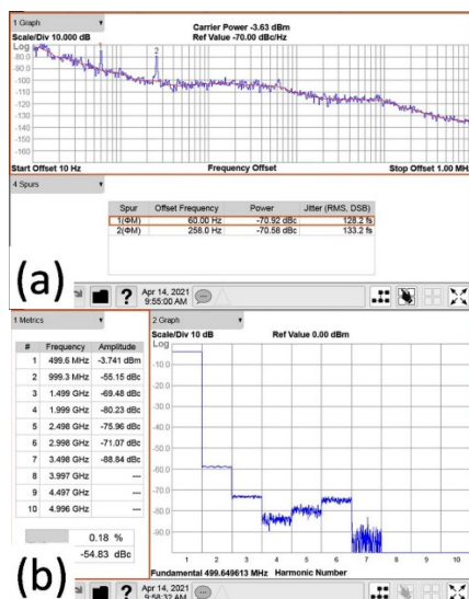
Figure 6: The quality of the combined RF of 2 80kW SSPA towers: (a) phase noise: -70.92 dBc@60Hz, -70.58 dBc@260Hz (b) harmonics: -55.15 dBc@2 nd and -69.48 dBc@3 rd harmonic.
