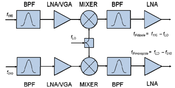
Fig. 5: Analog downconversion of symmetric dipole- and monopole mode signals
