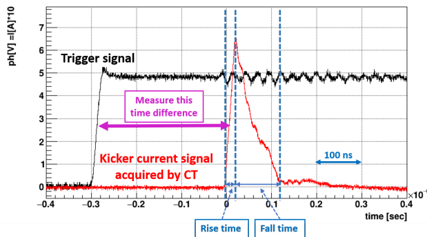
Figure 5: Kicker current signal as seen on the oscilloscope (Supply voltage : 1 kV).
