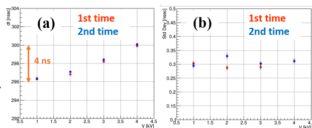
Figure 6: Measurement results average (a) and standard deviation (b) of the time difference between the trigger signal and the rise of the kicker current signal.
