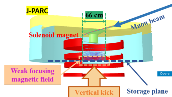
Figure 1: Image of the beam injected by the three-dimensional spiral injection scheme.
