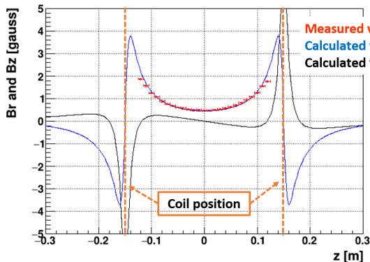
Figure 3: Calculation results of the magnetic field distribution created by the kicker coil and the radial magnetic field distribution measured by the pickup coil.
