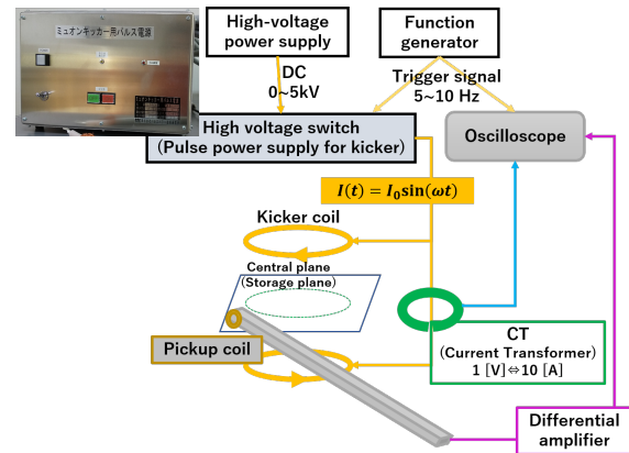
Figure 4: Experimental setup for stand-alone performance evaluation measurement.
