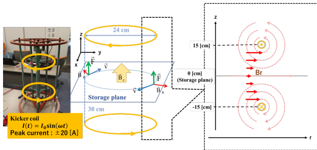
Figure 2: Prototype pulse magnetic field kicker device for our test bench with the electron beam, and the schematic diagram of the coil arrangement and the radial magnetic field generation of this kicker device.
