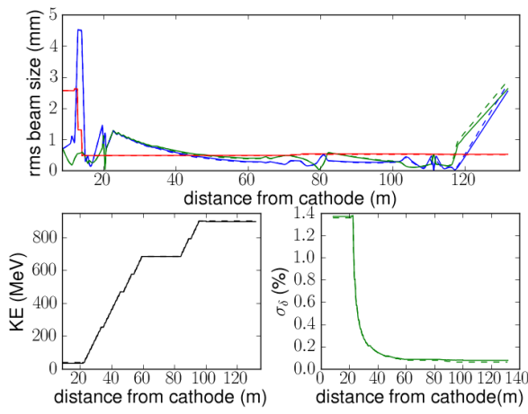
Figure 3: Single-particle-dynamics simulation using ELE-GANT (dashed line) and IMPACT-Z showing the evolution of \sigma_x (blue), \sigma_y (green), and \sigma_z (red) [top plot], the kinetic energy [bottom left] and fractional energy spread \sigma_\delta [bottom right].
