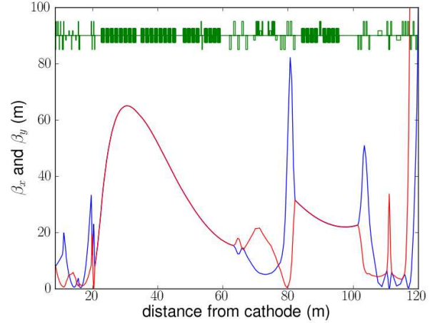
Figure 2: Lattice functions \beta_x (blue) and \beta_y (red) along the STF@NML beamline simulated with ELEGANT.
