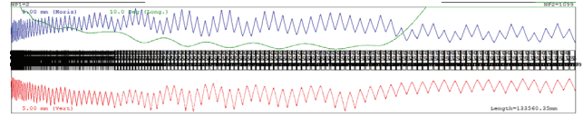
Figure 11: End-to-end simulation of the linac to 200 MeV at 50 mA.
