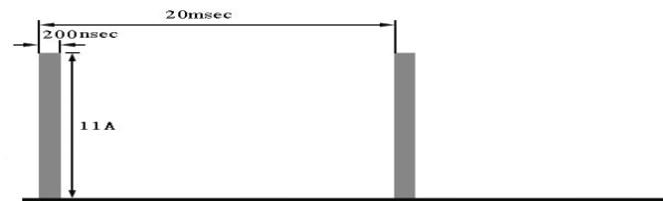
Figure 4: Time structure of short-pulsed mode.
