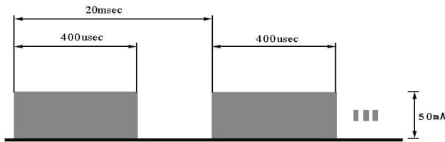
Figure 2: Time structure of the long-pulsed mode.
