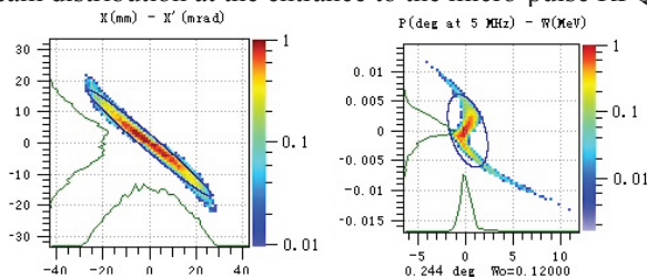
Figure 6: Particle distribution in transverse (left) and longitudinal (right) planes at the end of the LEBT.
