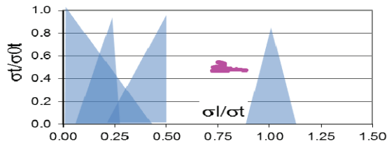
Figure 8: Hofmann coherent resonance diagram for the DTL.
