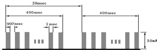
Figure 3: Time structure of micro-pulsed mode.
