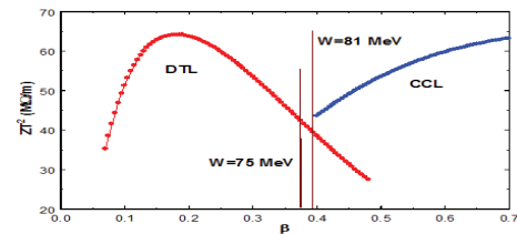
Figure 7: ZT^2 as a function of \beta .
