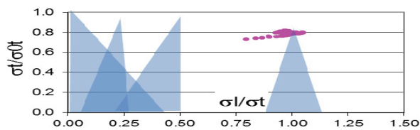
Figure 9 Hofmann coherent resonance diagram for the CCL.
