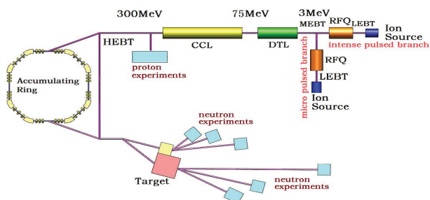
Figure 1: Schematic of the CIAE complex.
