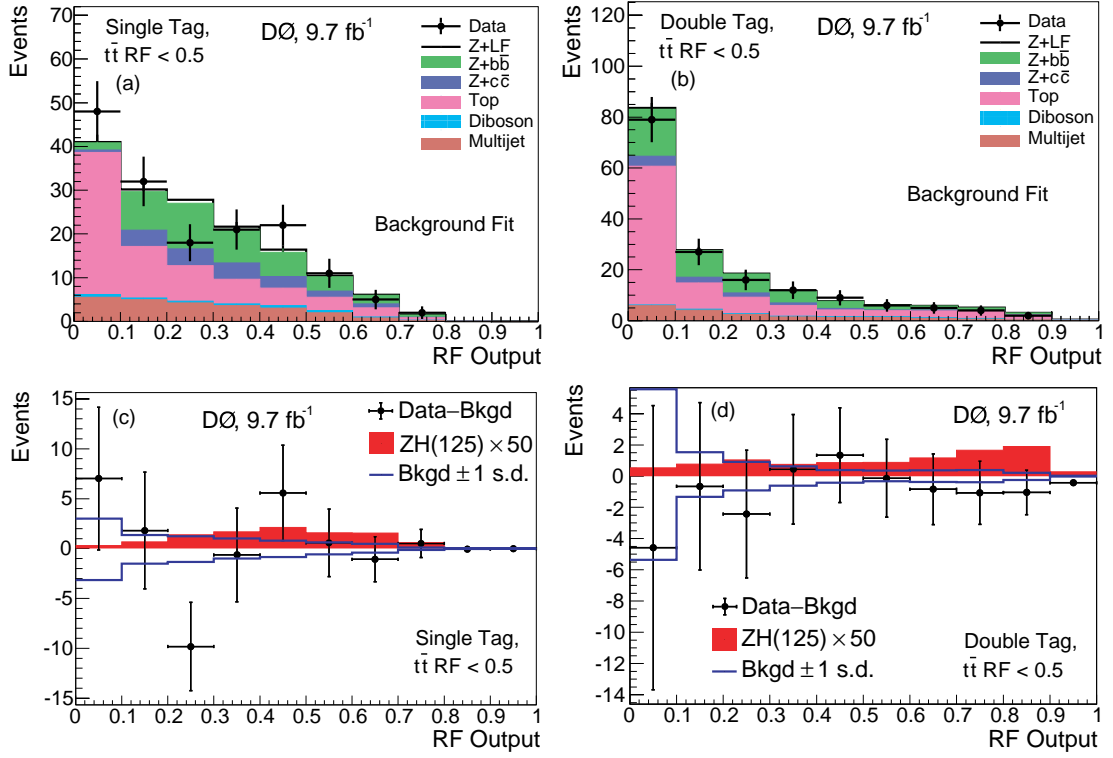
FIG. 7: Post-fit RF output distributions in the t\bar{t} enriched region, assuming M_H = 125 \text{ GeV} , after the fit to the background-only model for (a) ST events and (b) DT events. Background-subtracted distributions for (a) and (b) are shown in (c) and (d), respectively. Signal distributions are shown with the SM cross section scaled to 50 \times \text{SM} prediction in (c) and (d). The blue lines are the total posterior systematic uncertainty following a fit of the background to the data.
