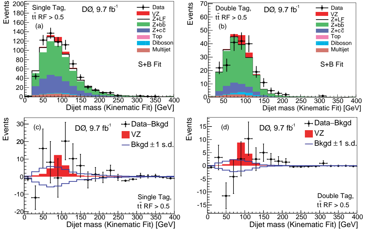
FIG. 10: Post-fit distributions of the dijet invariant mass (from the kinematic fit) in the t\bar{t} depleted region after the fit to the S+B model for (a) ST events and (b) DT events. Background-subtracted distributions for (a) and (b) are shown in (c) and (d), respectively. Signal distributions are scaled to the measured VZ cross section. The blue lines indicate the uncertainty from the fit.
