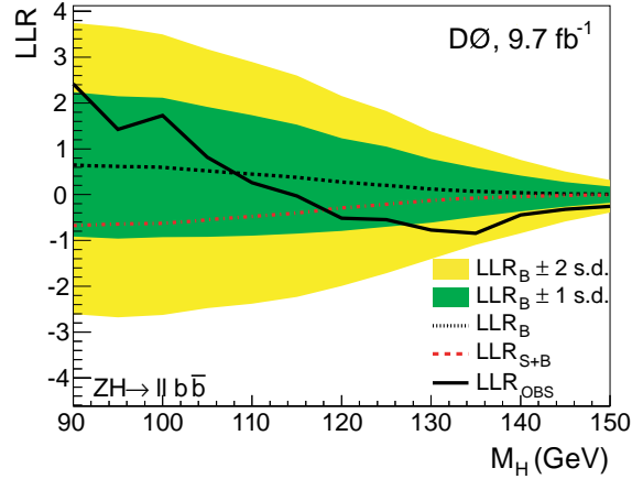
FIG. 8: Observed LLR as a function of Higgs boson mass. Also shown are the expected LLRs for the background-only (B) and signal+background (S+B) hypotheses, together with the one and two standard deviation (s.d.) bands about the background-only expectation.
