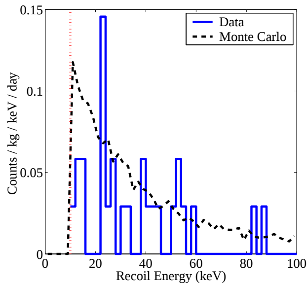
Figure 5.7: Recoil energy spectra from the veto-anticoincident germanium data set and the corresponding external neutron Monte Carlo. (a) inner data set. (b) inner + shared data set.
