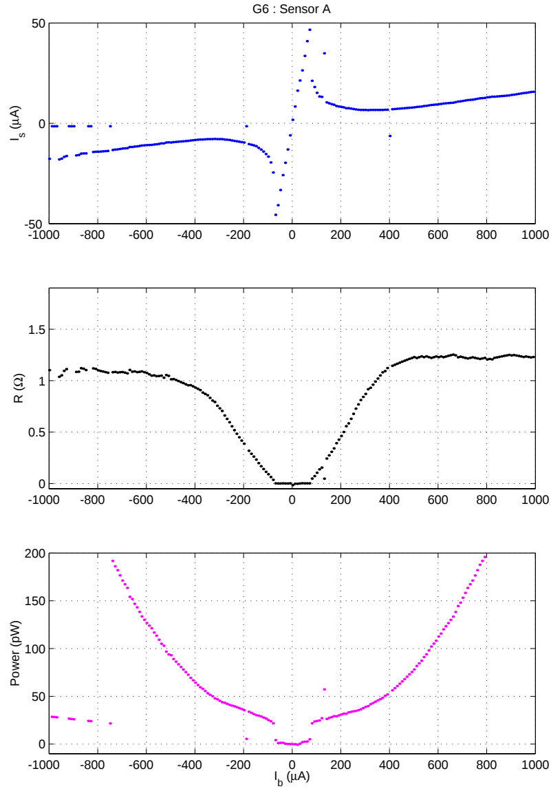
Figure 6.6: IbIs data from sensor A. The three plots correspond to sensor current I_s , sensor resistance, and Joule power dissipation in the sensor as a function of the bias current I_b . See the text for details on the expected shapes of these curves. The few points that deviate from smooth behavior in these curves are artifacts due to “SQUID lock-point jumps”, and therefore are of no significance.
