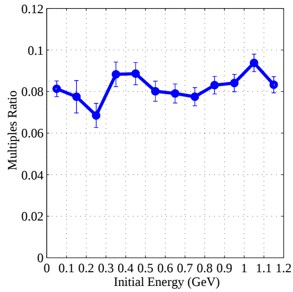
Figure 5.4: The dependence of mean recoil energy and multiples fraction on initial neutron energy.
