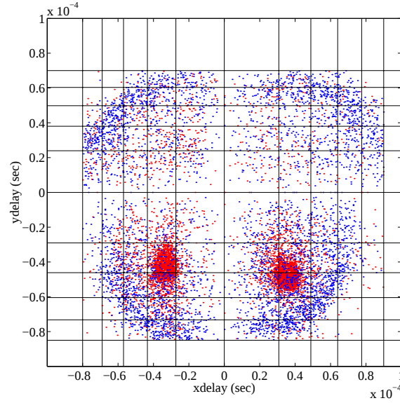
Figure 6.13: X_{delay} vs. y_{delay} for ^{241}\text{Am} and ^{137}\text{Cs} photons in G6 . Note that alphas are not included here because only events to the left of the vertical dashed line in figure 6.11 have been used. However, similar plots for the alpha events show that they are also concentrated at the two dense spots seen here due to photons from ^{241}\text{Am} . The more uniform distribution of events is mostly due to the ^{137}\text{Cs} source.
