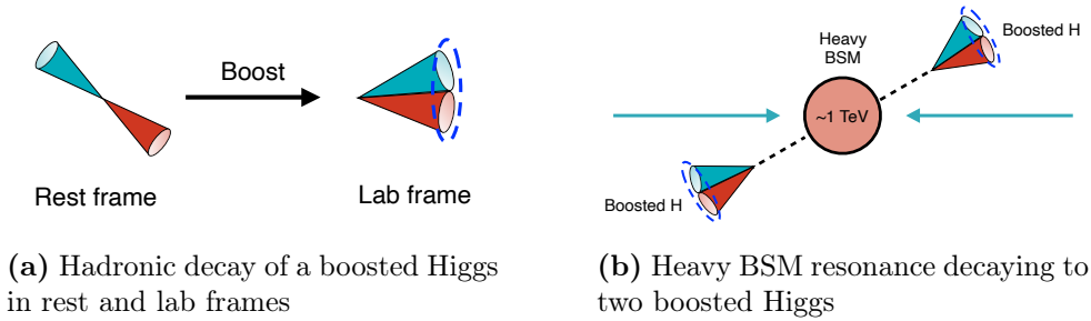
Figure 0.1 Boosted Higgs hadronic decay, and its importance for new physics searches.
