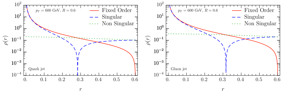
Figure 3.6 The differential jet shape at order \alpha_s for quark jets (left) and gluon jets (right) at p_T = 600 GeV and R = 0.6 . Shown are \rho_{r \lesssim R} (red solid), decomposed in its singular \rho_{r \ll R} (blue dashed) and nonsingular (green dotted) contribution that correspond to the power corrections in eq. (3.17).
