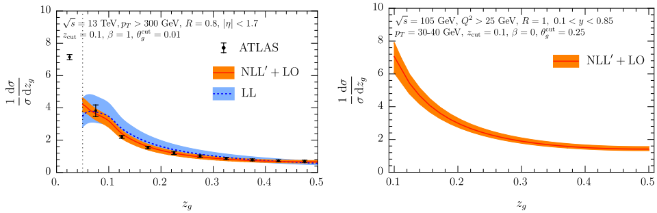
Figure 6.6 Comparison to ATLAS results [159] for \beta = 1 (left). Prediction for the Electron-Ion Collider (right).
