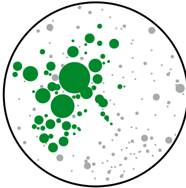
Figure 5.1 Schematic picture of a jet, with circles representing radiation whose size corresponds to its energy. Wide-angle soft radiation (grey) is groomed away, resulting in the groomed jet (green).
