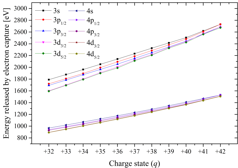
Fig. 2. Dependence of energy released by electron capture into the M and N subshells of the ^{93m}\text{Mo} isomer on the specific charge state q .
