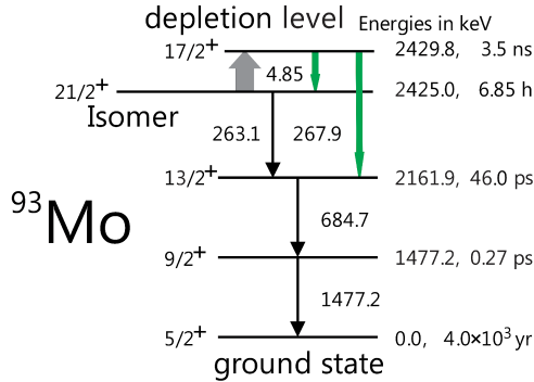
Fig. 1. (Colour on-line) Partial level scheme for the 93 Mo isotope. The thick grey arrow is the transition excited by NEEC and the thin black arrows show the natural decay cascade from the 93m Mo isomer. The thick dark grey/green arrow transitions are only emitted following NEEC [10].
