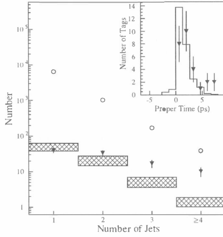
Figure 1: Number of events before SVX tagging (circles), number of tags observed (triangles), and expected number of background tags (hatched) versus jet multiplicity. Based on the excess number of tags in events with \geq 3 jets, we expect an additional 0.5 and 5 tags from t\bar{t} decay in the 1 and 2 jet bins respectively. The inset shows the secondary vertex proper time distribution for the 27 tagged jets in the W + \geq 3 -jet data (triangles) compared to the expectation for b quark jets from t\bar{t} decay.
