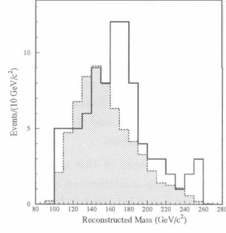
Figure 2: Reconstructed mass distribution for the W + \geq 4 -jet sample prior to b -tagging (solid). Also shown is the background distribution (shaded), with the normalization constrained to the calculated value.
