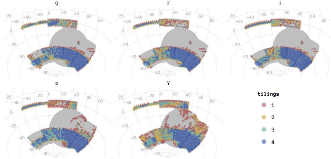
Figure 5 The Y1 survey fields include Stripe 82 (at the Equator), and the boxed-in area at roughly -40 < RA < -60 degrees. We scheduled four tilings in each filter. The colored dots represent the number of “good” exposures (as defined by the t_{\text{effective}} data quality criterion described above) achieved in each filter. Grey-colored fields are unobserved.
