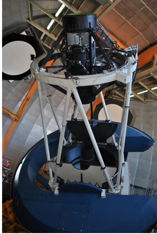
Figure 1 The Dark Energy Camera is mounted at the prime focus of the Blanco 4m telescope at CTIO. The covers for the primary mirror are open. The camera assembly, including the support cage, is approximately 3.6 m long and is secured to the inner telescope ring. The camera, not including the support cage and counterweights, weighs approximately 4350 kg. Subsequent to the date of this photo the cage was retrofitted with aluminum side-covers. The aluminum covers of two of the four readout electronics crates are visible near the top of the camera, just underneath the “Top Cap”.
