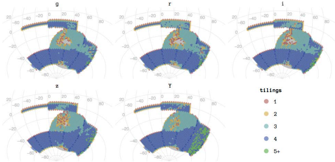
Figure 6 The Y1-Y2 WF survey observations included the fields that were not observed in Y1 with the goal of observing 4 tilings in each filter. The colored dots represent the number of “good” exposures (as defined by the t_{\text{effective}} data quality criterion described above) achieved in each filter. Note that by the end of Y2 we have a region where we haven’t taken any exposures (the center of the fat part of the field), and some areas where we have 5 or more good exposures (particularly in the Y-band, east side).
