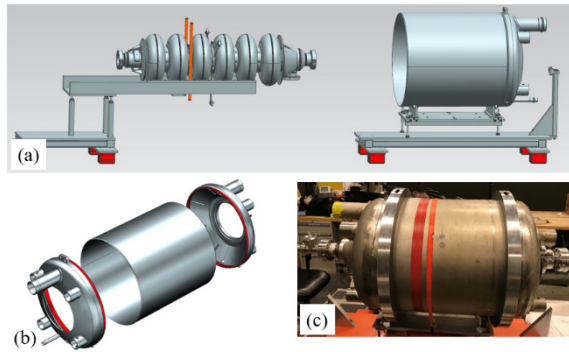
Figure 2: (a) The schematic of the He vessel welding fixture with cavity on rail, (b) schematic of helium vessel and (c) the cavity after completed welding.
