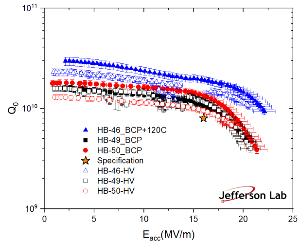
Figure 4: Summary of RF test before and after HV welding at 2.1 K.
