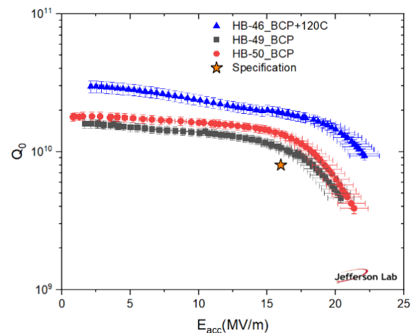
Figure 1: RF test summary of developmental cavities before helium vessel welding at 2.1 K.
