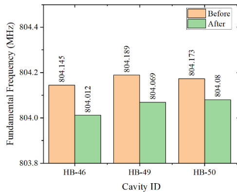
Figure 3: The fundamental frequency before and after the HV welding.
