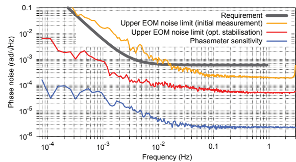
Figure 2. Differential phasenoise measurement.
