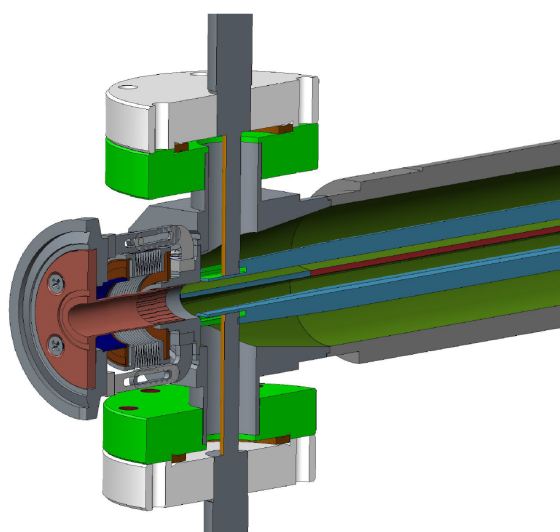
Figure 3: Tapered section of the stripline kicker model.
