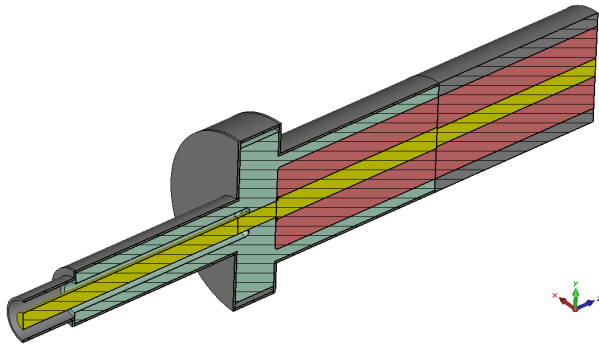
Figure 6: High voltage feedthrough model.
