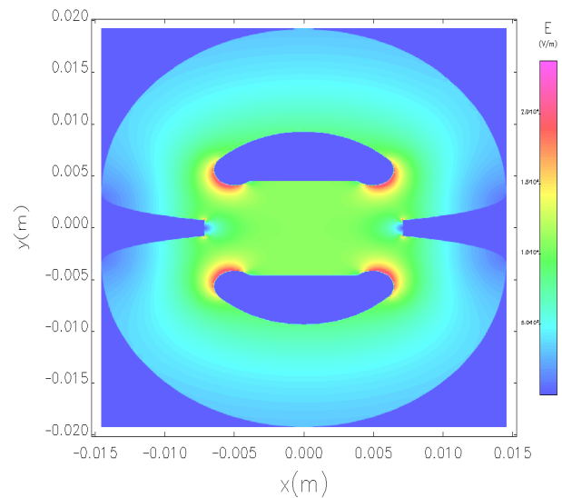
Figure 2: Field distribution of 2-D optimized model.
