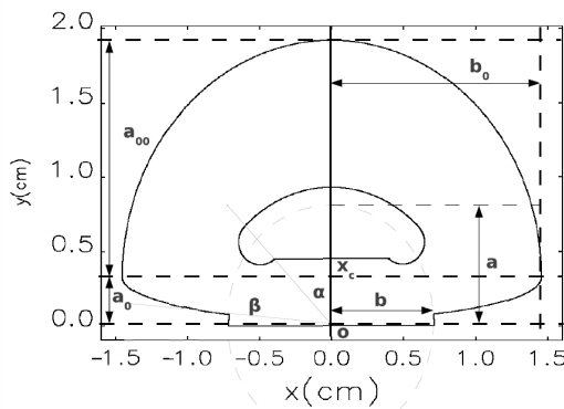
Figure 1: Geometry of the stripline kicker 2-D model.
