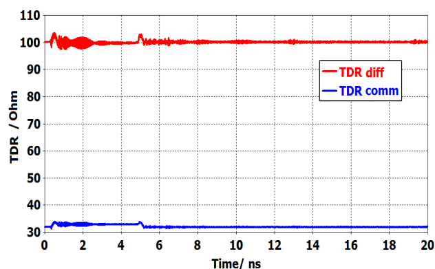
Figure 4: TDR of common and differential modes.
