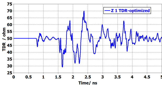
Figure 7: TDR result of the high voltage feedthrough.
