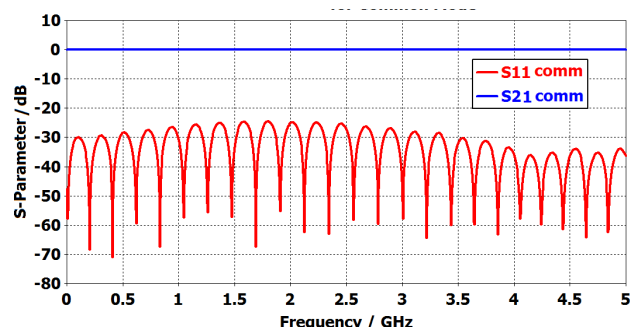
Figure 5: Common-mode S-parameters.
