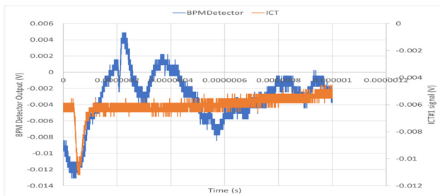
Figure 9: 2SC4083 active-filter output response to button BPM with 150 pC charge beam.
