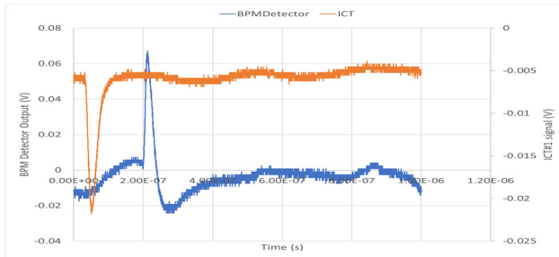
Figure 8: 2SC4083 active-filter output response to button BPM with 500 pC charge.
