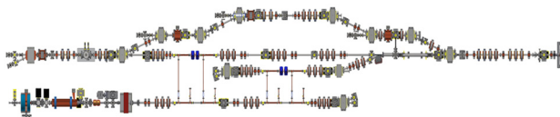
Figure 1: AWA beamline layout.
