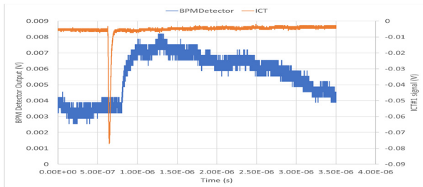
Figure 7: 2N2222 active-filter output response to button BPM with 2 nC charge beam.
