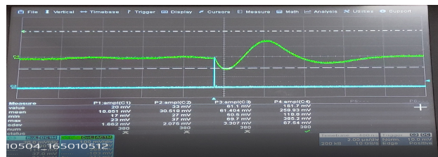
Figure 5: Bench test results of BPM active filter using 2N2222.
