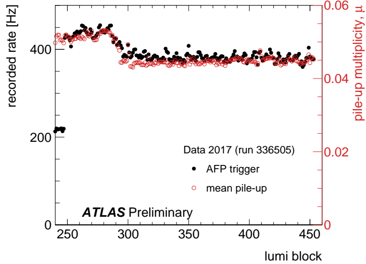
Figure 4.22: AFP trigger rate (black) together with the pile-up rate (red) over the luminosity blocks of a chosen ATLAS run. Taken from Ref. [130].
