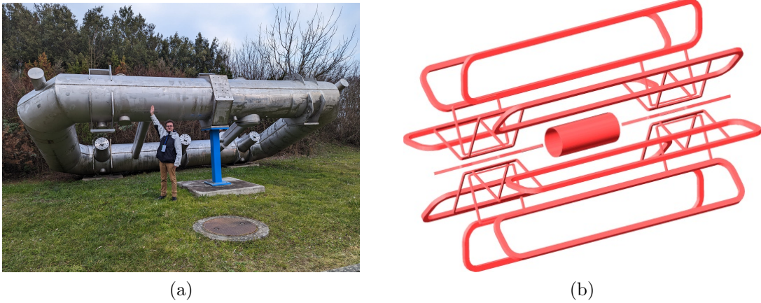
Figure 3.8: (a) Photograph of a final prototype of a toroid magnet at \simeq \frac{1}{3} scale. The prototype is displayed in front of the entrance of the ATLAS control room at CERN. A person is standing in front of the magnet for scale. (b) Schematic of the ATLAS magnet system. Both solenoid and toroidal systems are shown. Taken from Ref. [88].
