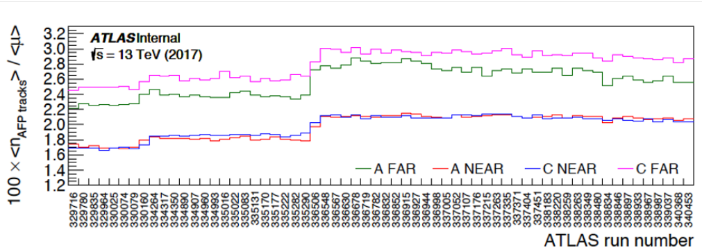
Figure 4.23: Mean number of tracks reconstructed in each station normalized by the average pile-up multiplicity in different ATLAS runs. This quantity is multiplied by 100. The observed step is due to a change of data-taking conditions over the course of 2017.
