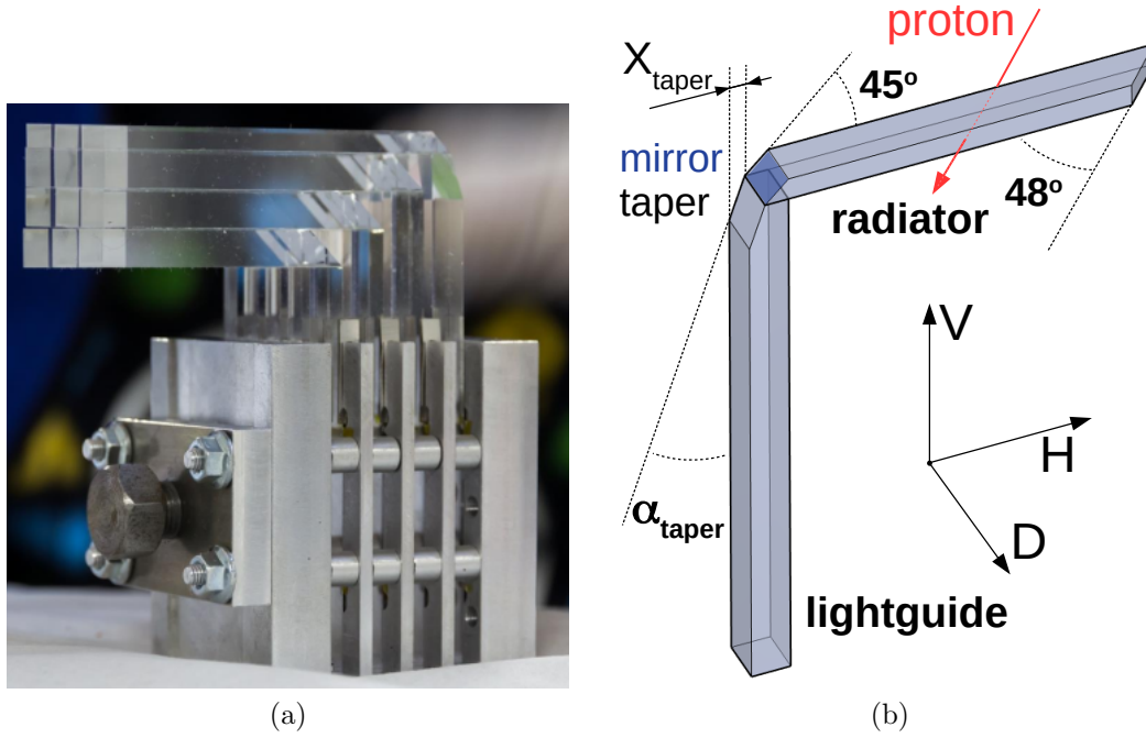
Figure 4.6: (a) Photograph of the ToF detector. (b) Schematic view of a single quartz Cherenkov bar. Taken from Ref. [116].
