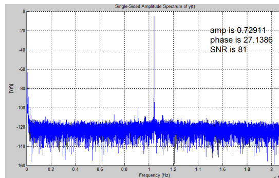
Figure 4: The SNR of one of ADC channel.
