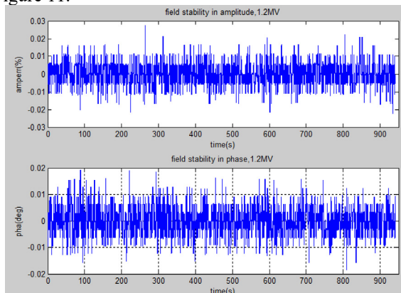
Figure 11: The amplitude and phase stability within 15 minutes when the cavity voltage is 1.2MV.
