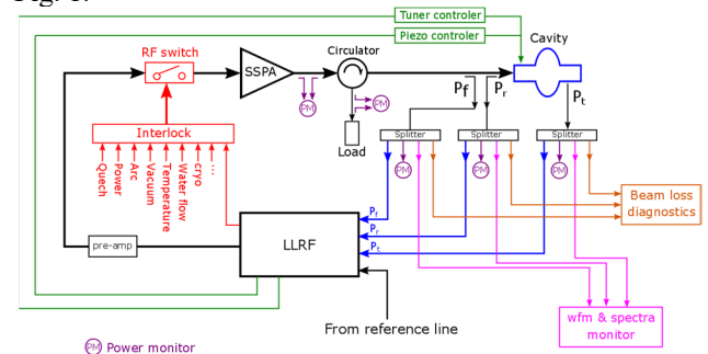
Figure 1: The diagram of RF system.
