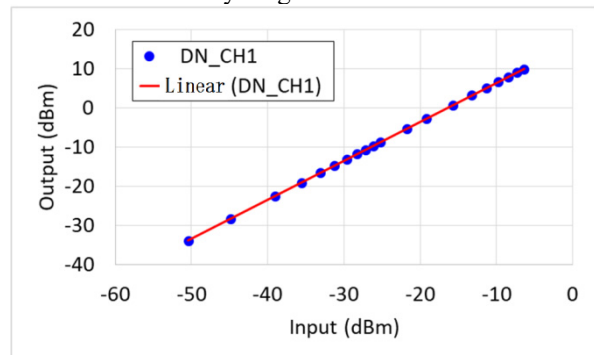
Figure 7: Up-conversion CH1 linearity of RF analog front-end board.
