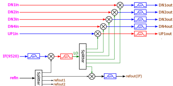
Figure 5: The diagram of RF front-end board.
