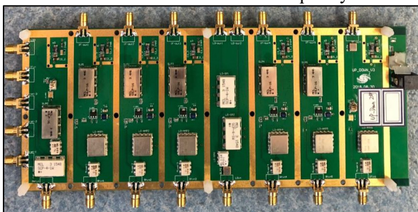
Figure 6: The first prototype of LLRF analog front-end board.
