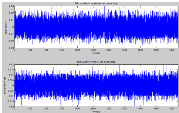
Figure 10: The amplitude and Phase Stability within 90 minutes by self-closed loop of the LLRF system.
