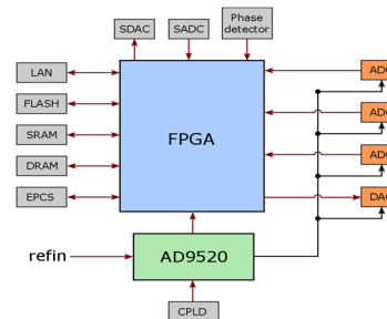
Figure 2: Functional diagram of low-level digital signal processing board (DSP).
