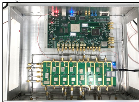
Figure 9: The LLRF control crate integrated with DSP board and analog front-end board.
