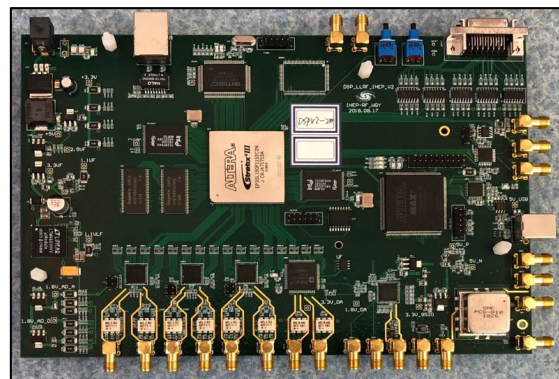
Figure 3: The first prototype DSP board.
