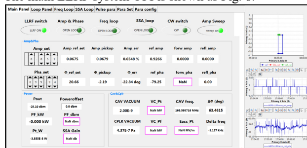
Figure 8: The main LLRF system OPI.
