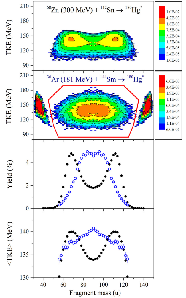
Fig. 2. From top to bottom: the mass-energy distribution of fissionlike fragments formed in the ^{68}\text{Zn} + ^{112}\text{Sn} reaction at E_{\text{lab}} = 300 \text{ MeV} ; the mass-energy distribution of fragments formed in the ^{36}\text{Ar} + ^{144}\text{Sm} reaction at E_{\text{lab}} = 181 \text{ MeV} ; the comparison of mass yields and mean total kinetic energies as a function of mass for the reactions ^{68}\text{Zn} + ^{112}\text{Sn} (solid circles) and ^{36}\text{Ar} + ^{144}\text{Sm} (open circles).
