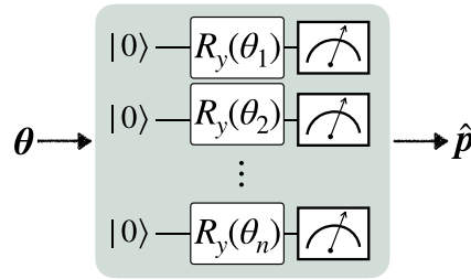
Figure 3. The quantum circuit for generating the noisy probability distribution \hat{\mathbf{p}} used as an input to the NN during training. The training data is generated by applying an arbitrary single-qubit rotation R_y(\theta) to each qubit and measuring qubits in the computational basis. Training of the NN also requires the ideal probability distribution \mathbf{p} , and this is calculated using the set of rotation angles \theta used in the quantum circuit.
