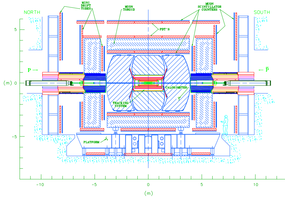
Figure 3.2: Two-dimensional view of the Run II DØ detector, showing the three integral systems outlined in the text.
