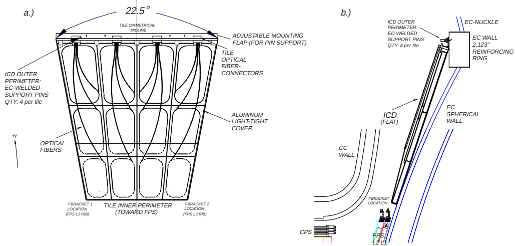
Figure 8.8: One of sixteen flat ICD panels mounted on each end-cryostat head. Shown are: a) r-\phi view and b) r-z view of a tile.
