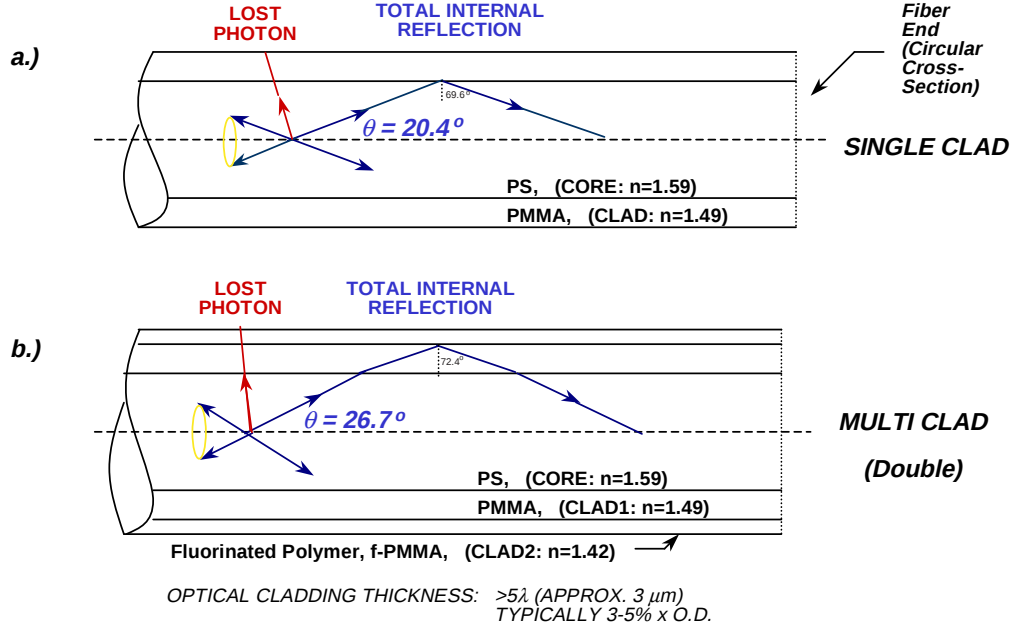
Figure 5.2: Schematic configuration of a typical WLS fiber: a) single clad and b) double clad fibers are shown. Adapted from [62, 32].
