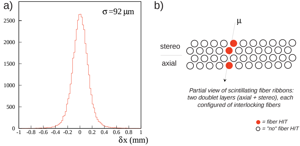
Figure 3.7: a) Distribution for the position resolution measured in the Fiber Tracker for single muons traversing b) an interlocking ribbon doublet configuration.
