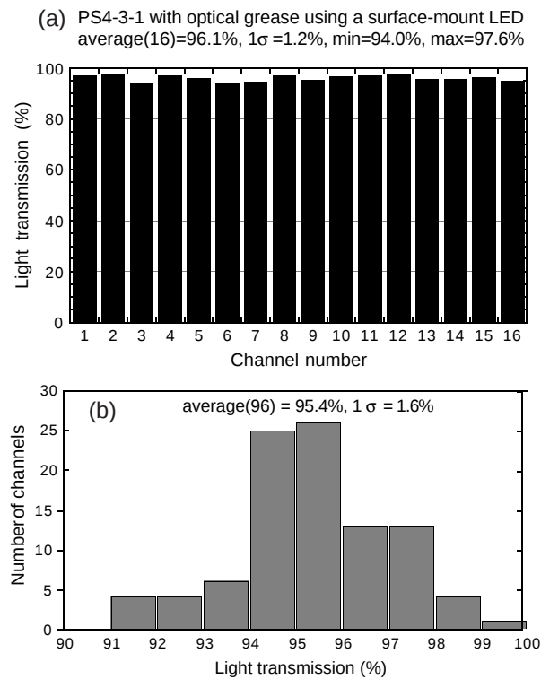
Figure 7.22: Observed light transmission for each channel in a 16-channel one-to-one mated connector assembly (a), and the measured distribution of fiber channel transmissions (b). Both distributions yield, on average, 95% light transmission through the fiber/connector interface.
