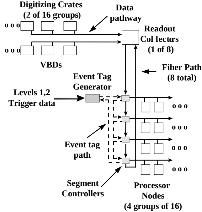
Figure 3.20: L3 trigger framework. Data flow is indicated by the direction of the arrow.
