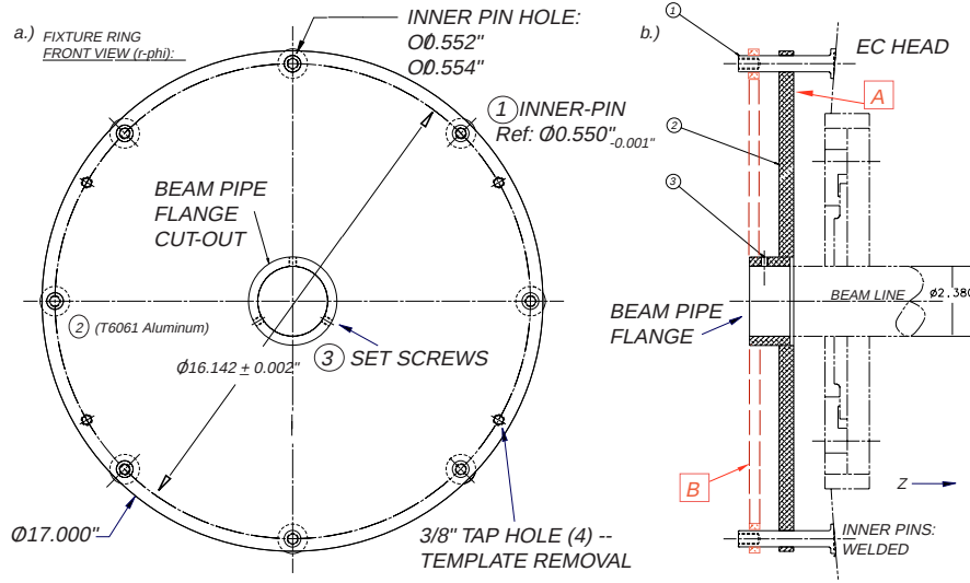
Figure 8.1: a) r - \phi view of template used to align and weld eight stainless-steel inner pins for FPS support on EC heads and b) r - z view of assembly. Also shown is an inner ring (B) mounted in z with the template (A) to guarantee each pin is parallel to one another.
