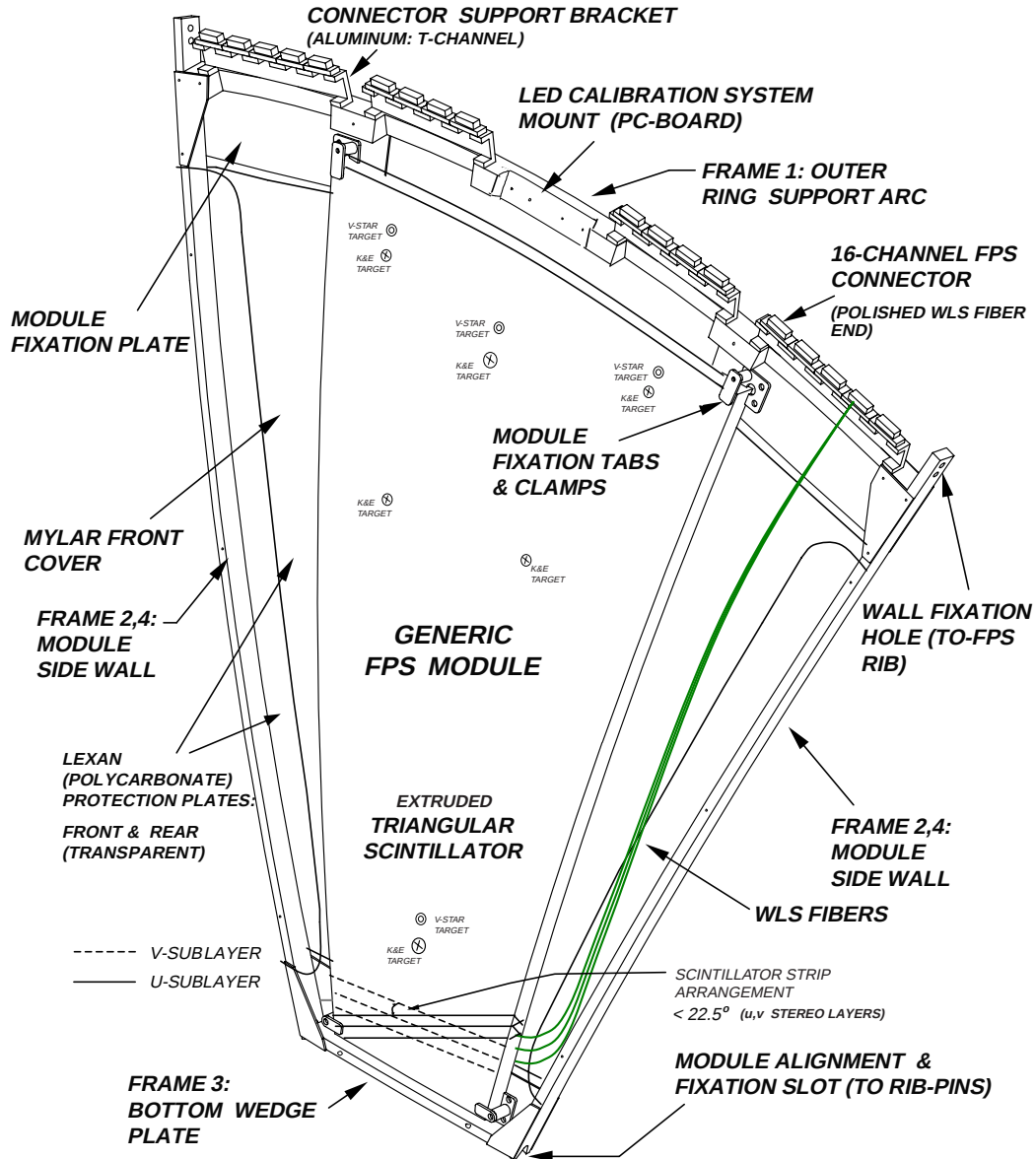
Figure 6.4: Three-dimensional view of a trapezoidal shaped FPS \phi -module in its supporting frame. Shown are the main elements including WLS fibers, optical connectors and brackets, surveying targets, and protective clear frame-covers. See text for complete description.
