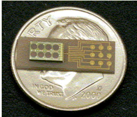
Figure 5.9: Picture of a VLPC chip. The chip has 8 pixels of 1 mm diameter mounted on an aluminum-nitride substrate. The gold-plate conduction pads on the substrate are contacts for the 8 signal outputs and the bias.
