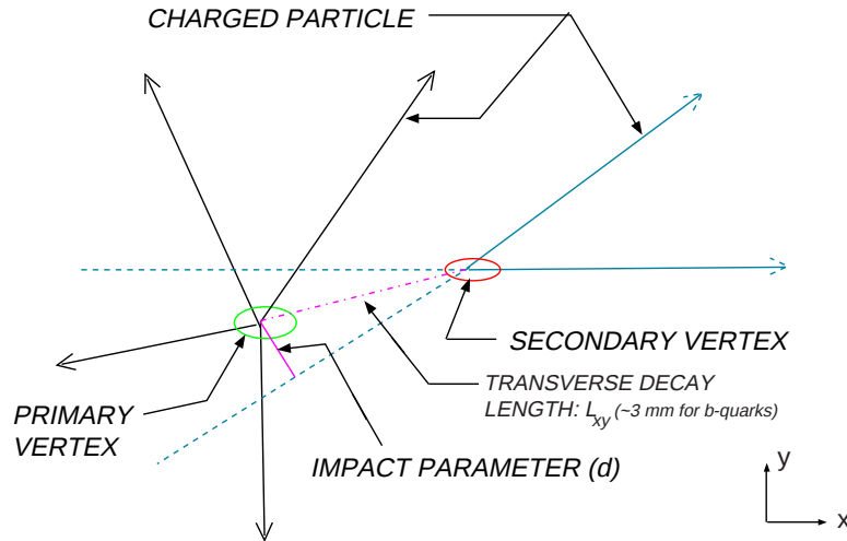
Figure 3.4: Schematic of an observed displaced vertex originating from b or c quarks in a silicon microstrip detector.
