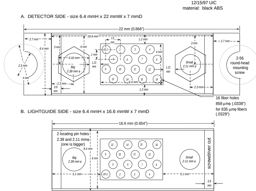
Figure 7.23: Front face of the 4 \times 4 array, sixteen-channel FPS a) WLS-fiber (detector-side) optical connector and its mating b) clear-fiber (light-guide side) connector. All dimensions are given for completeness.
