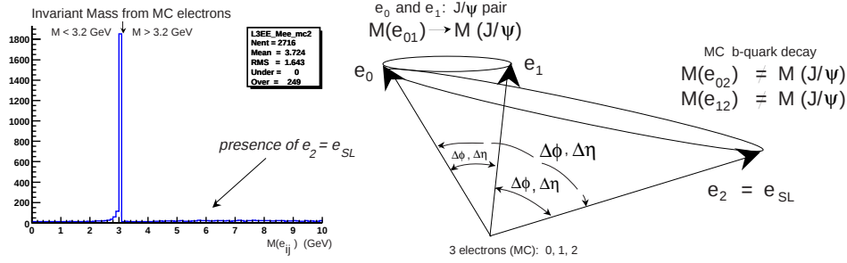
Figure 9.32: Figurative example of three MC-level electrons in the J/\psi sample. Two of these arise from J/\psi decays while the third must be from the semi-leptonic decay of the b -quark.
