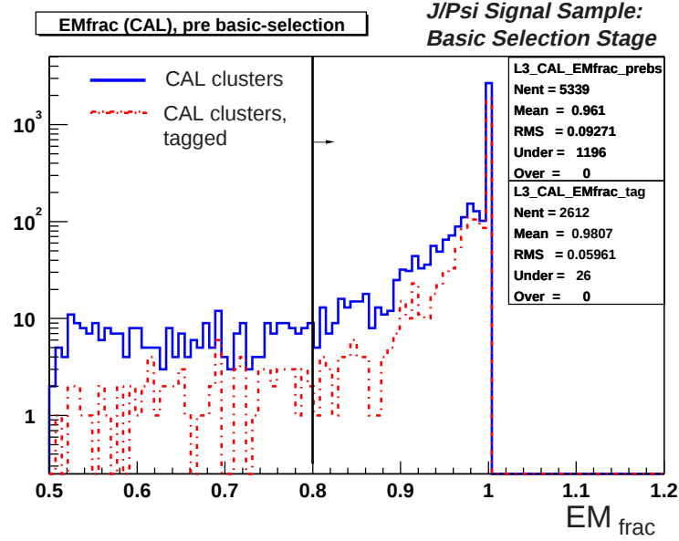
Figure 9.15: EM_{frac} measured within the central calorimeter fiducial. Shown is the distribution for reconstructed clusters (solid-line) and tagged-electron tracks (dashed-line). An initial cut at 0.8 is applied for basic selection of electrons.
