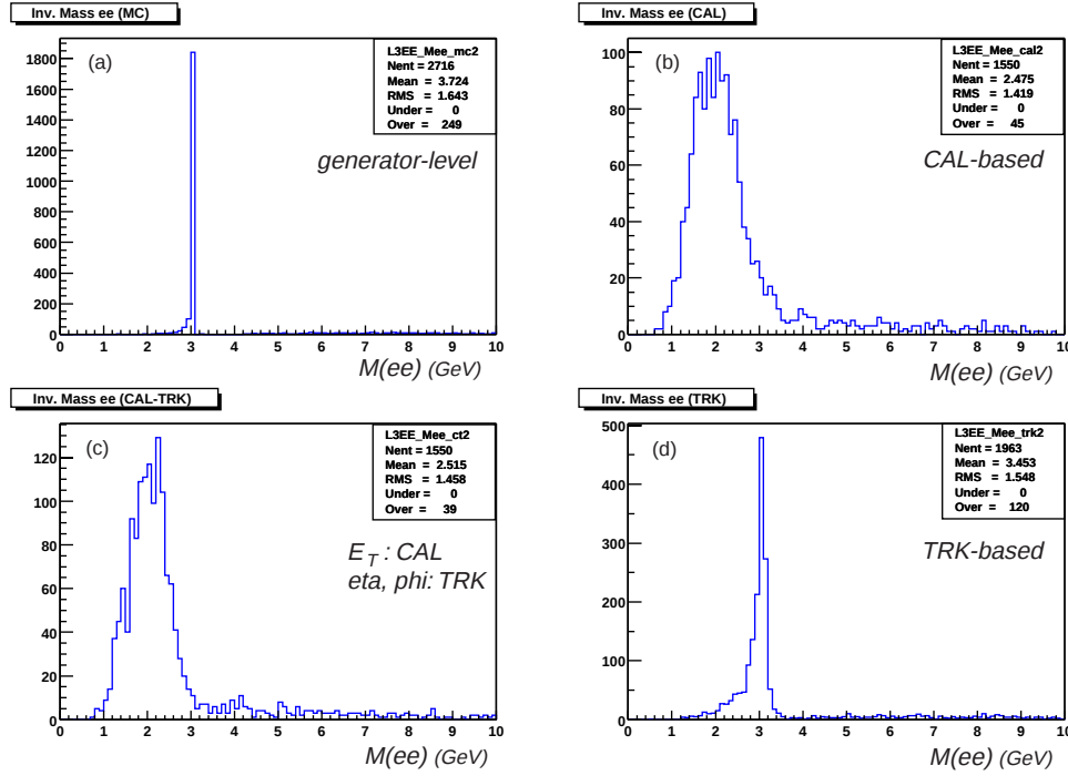
Figure 9.14: Invariant mass resolutions for e^\pm pairs from J/\psi decays. Shown are reconstructed mass (using Eq.—9.2) from (a) MC generator-level, (b) calorimeter-based variables, (c) combined calorimeter E_T with track's \Delta\phi and \Delta\eta measurement, and (d) track-based variables.
