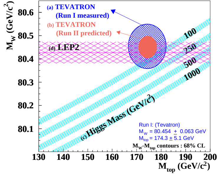
Figure 2.1: Measured Run I Tevatron W boson mass vs. top quark mass, shown by (a) cross-hatched oval, in addition with W mass band from LEP2, CERN (d). The four shaded bands (c) represent expected values for a specific Higgs boson mass in the SM, where the 1\sigma -width in each band is due to \alpha_s(M_Z^2) . The solid oval (b) shows a predicted Run II Tevatron measurement (using Run I central values) and is given for comparisons. Adapted from [17].
