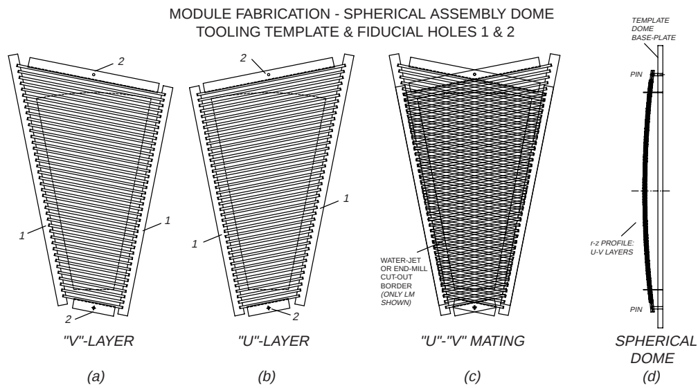
Figure 7.2: Strip-by-Strip layout using lateral alignment bars (1) and alignment stops (2) for module fabrication. Shown are a) v -layer, b) u -layer, and c) mated u - v layer, all assembled on d) the spherical ( r - z view) “template” dome. The fiducial holes in (2) serve to reference the module’s position during water-jet and/or end-mill cutting.
