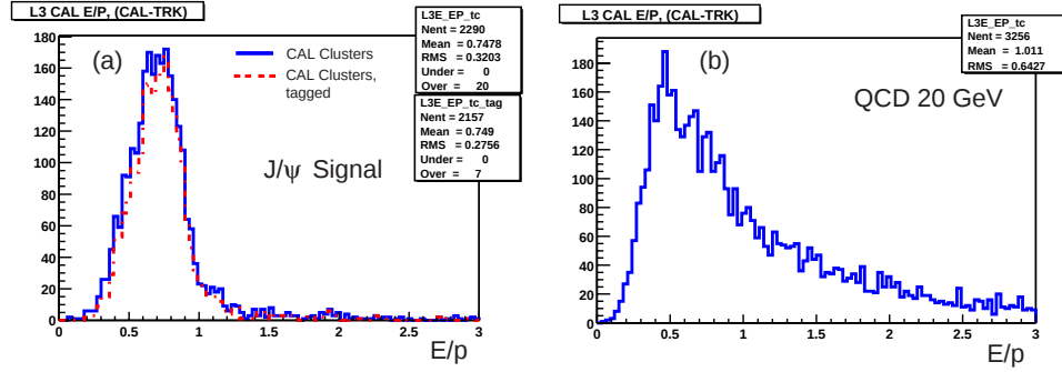
Figure 9.22: Distribution of E/p measured at L3 for a) signal and b) QCD. In (a), the reconstructed clusters (solid-line) are overlapped with tagged-electron tracks (dashed-line).
