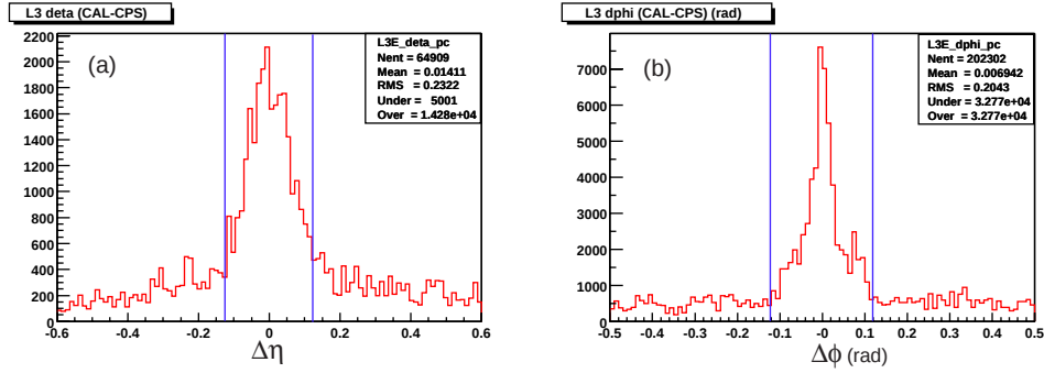
Figure 9.18: Distributions of matching between calorimeter and preshower clusters for electron selection in (a) \eta and (b) \phi for the J/\psi sample.
