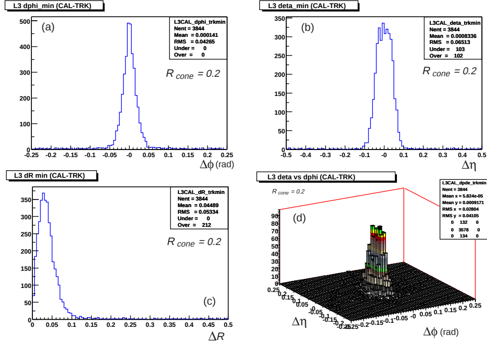
Figure 9.2: Distributions for (a) \Delta\phi , (b) \Delta\eta , and (c) \Delta R for tagged electrons in global tracks and calorimeter clusters in the J/\psi sample. A value of R_{cone} = 0.2 has been used to define L3 calorimeter clusters. The correlation in \Delta\eta with \Delta\phi is also shown in (d).
