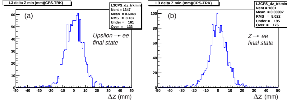
Figure 9.10: Match in z for CPS clusters and tracks for (a) \Upsilon \rightarrow ee and (b) Z \rightarrow ee final states.
