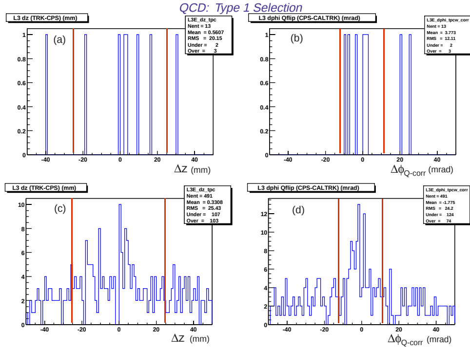
Figure 9.20: Similar distributions as in Fig. 9.19 for Type 1 selections implemented on (a-b) QCD p_T > 2 GeV and (c-d) QCD p_T > 10 GeV samples.
