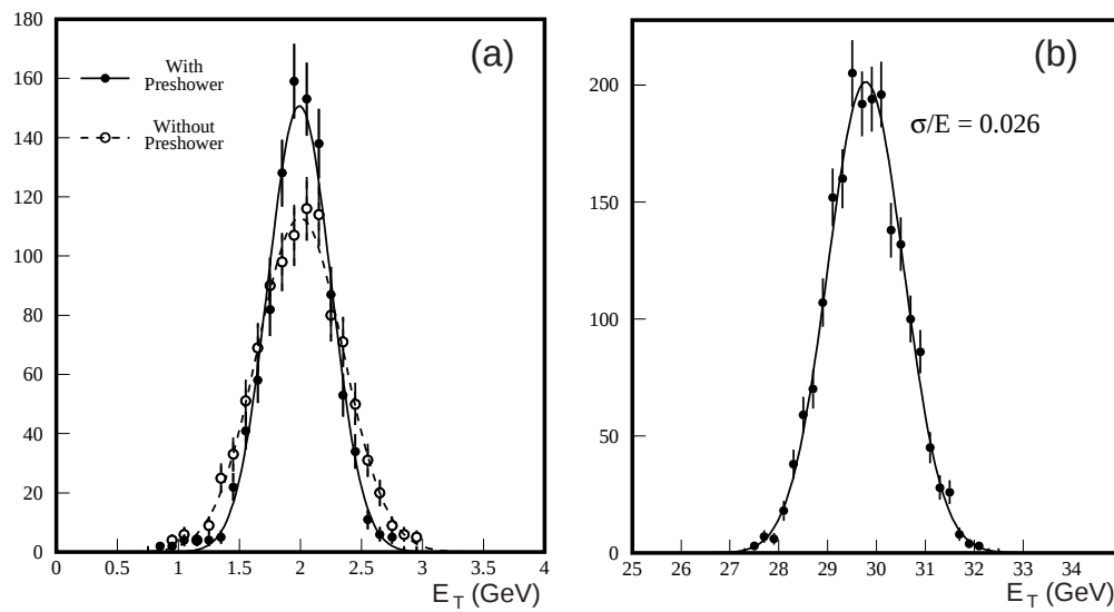
Figure 4.1: Simulation of the Run II DØ calorimeter measuring a) the response to E_T = 2 GeV electrons at \eta = 1 for the cases with (solid-line) and without (dashed-line) a preshower detector. The resolution with calorimetry alone is shown to be about 18% and improves to 13% when preshower information is included. Also shown is b) the response to E_T = 30 GeV electrons with a preshower detector.
