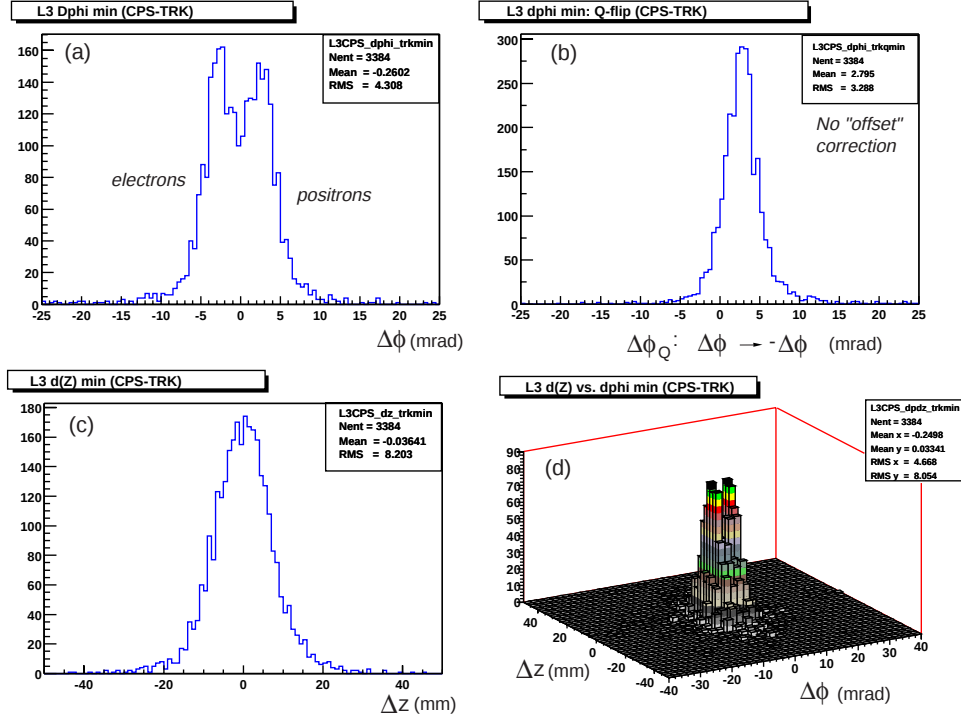
Figure 9.7: Distributions for (a) \Delta\phi and (c) \Delta z for tracks and CPS clusters using tagged electrons in the J/\psi sample. The correlation between these two variables is given in (d). Also shown in (b) is the \Delta\phi_{Q-flip} distribution without offset corrections, described in the text.
