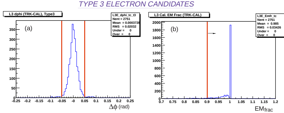
Figure 9.23: Type 3 selection variables and cuts implemented for electron identification in the J/\psi sample: (a) \phi -match between the tracker and calorimeter and (b) EM fraction measured in the calorimeter. Also, shown are the intervals in which selections have been made.
