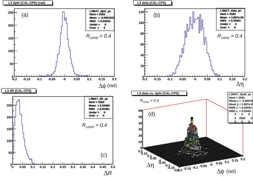
Figure 9.6: Distributions for (a) \Delta\phi , (b) \Delta\eta , and (c) \Delta R for calorimeter and CPS clusters using tagged electrons in the J/\psi sample. Results are for calorimeter clusters with R_{cone} = 0.4 . The correlation in \Delta\eta with \Delta\phi is also shown in (d).
