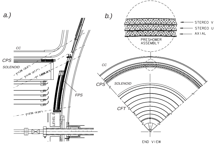
Figure 3.8: Central Preshower detector shown in: a) r - z semi-quarter-view and b) cross-sectional ( r - \phi ) end-view of the D\phi tracking system. The inset in (b) gives a magnified view of the triangular strip nesting and layer configuration.
