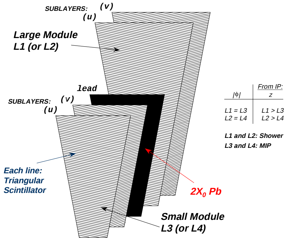
Figure 6.1: FPS module's azimuthal geometry with joint u - v MIP and Shower sublayers, each separated by a lead absorber.
