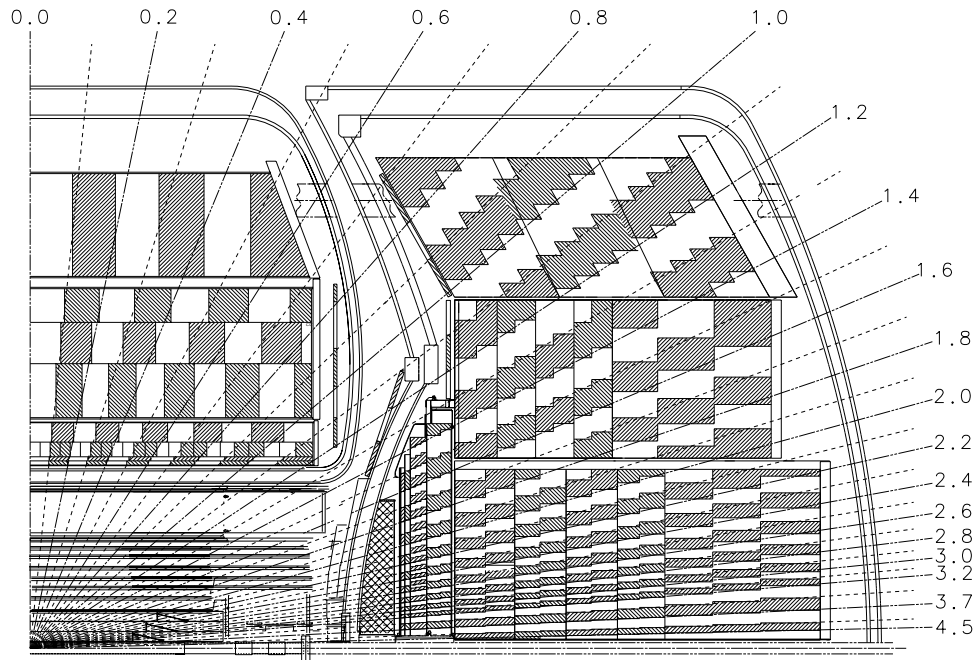
Figure 3.11: Side-view of one quarter of the D\bar{O} calorimeter system, showing segmentation and tower definitions (see text). The lines extending from the center of the detector denote the pseudorapidity coverage of cells and projected "towers".
