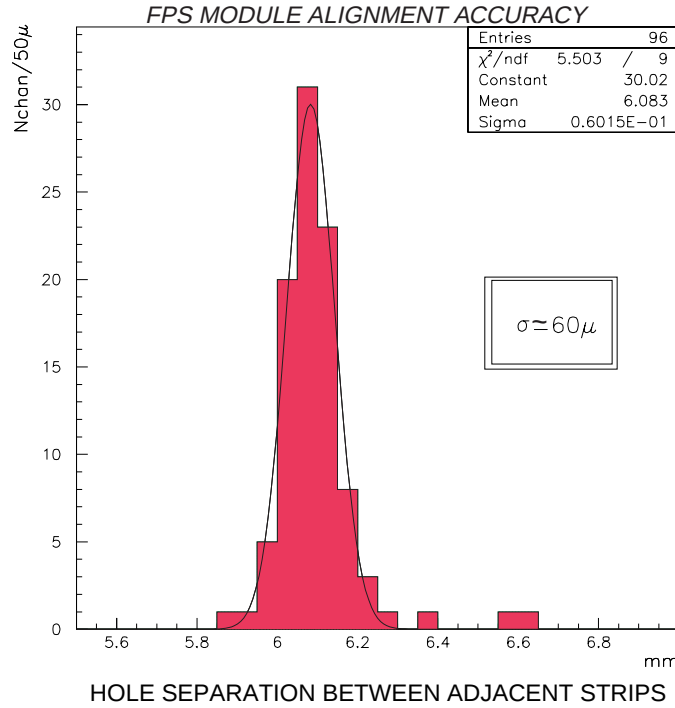
Figure 7.3: Result for channel-to-channel alignment accuracy measured using a CMM for a FPS module. A narrow distribution with an accuracy of about 60 \mu\text{m} is achieved and well within design specifications.
