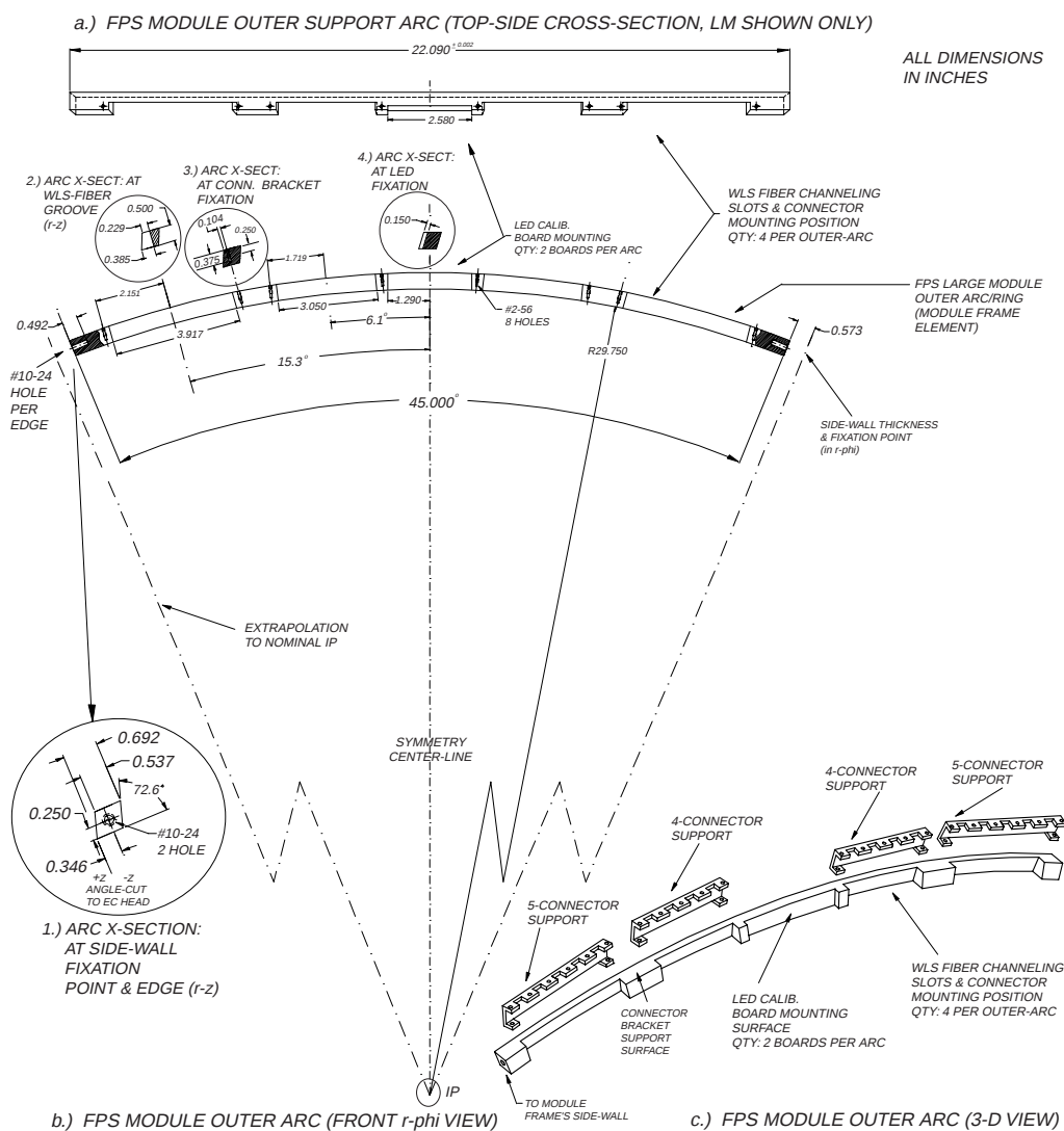
Figure 7.5: Production print of the outer support arc in a large module/frame unit. The arc is precisely machined with angles on both the \pm z -surfaces to conform to the spherical EC head. For completeness, r - z cross-sectional views along the arc are shown in circles #1-4. The geometry for the SM and SpM arcs is designed and constructed similarly.
