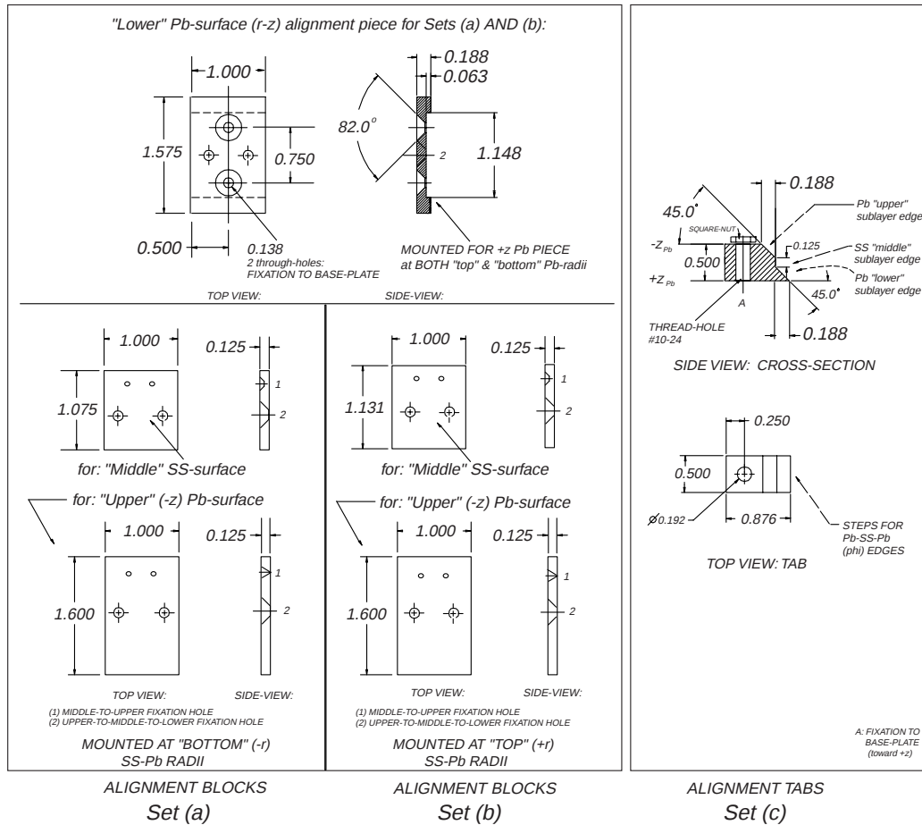
Figure 7.18: Registration hardware for lead-stainless-steel-lead pieces used during bonding. Items (a) and (b) control the r - z alignment of individual Pb-SS-Pb sublayers, whereas (c) defines the \phi -positioning of each piece.
