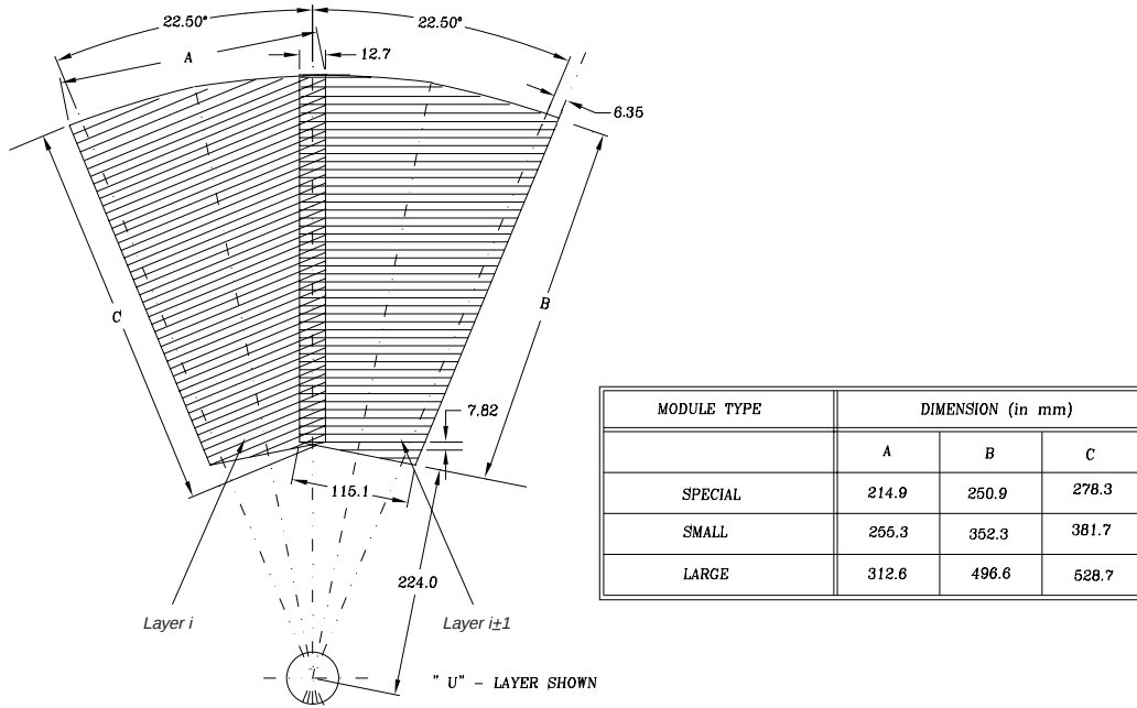
Figure 6.5: Module orientation within two successive FPS layers. Given is the 1/2'' overlap region between two adjacent \phi -modules as well as dimensions of the active area of each module type (see text for description).
