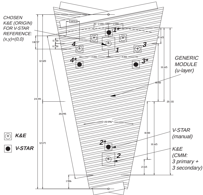
Figure 8.6: Generic FPS module illustrating the six (1-6) CMM installed K&E targets and four (1*-4*) manually placed V-star targets. K&E target #1 defines the origin and reference to which all other V-star mapping positions are made.
