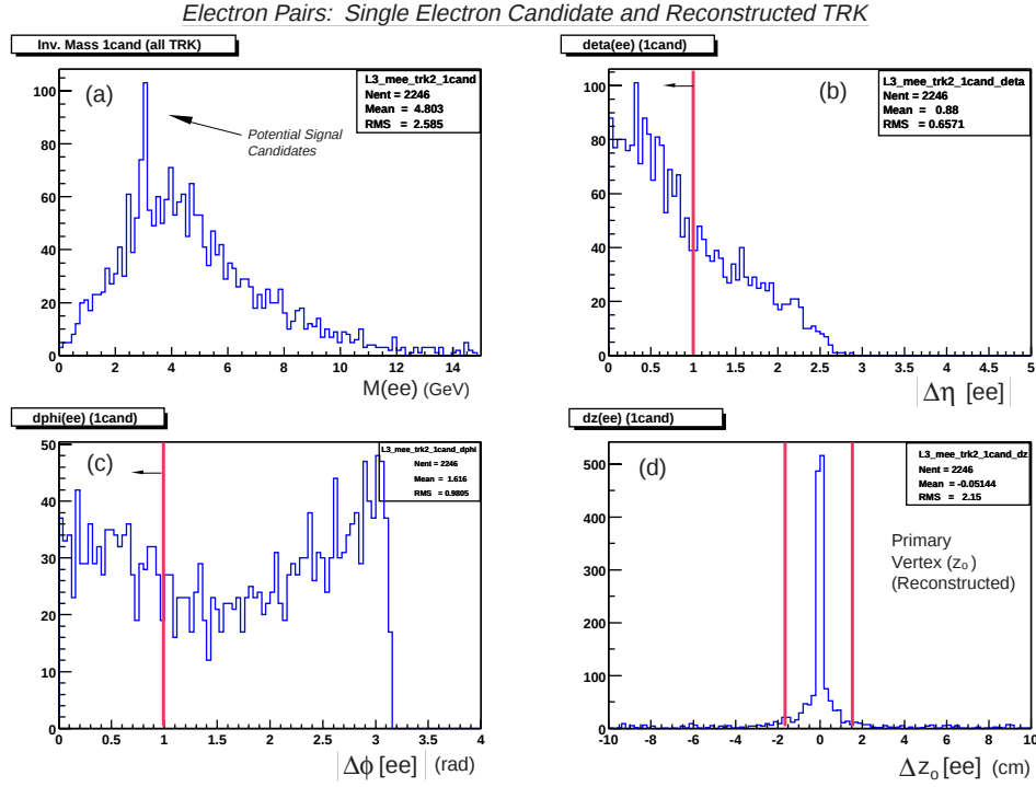
Figure 9.29: (a) Invariant mass distribution as for single electron candidates in the J/\psi signal sample paired with L3 reconstructed tracks. Also shown are corresponding (b) \Delta\eta , (c) \Delta\phi , and (d) \Delta z_0 distribution for all pairs. Results for R_{cone} = 0.2 are shown.
