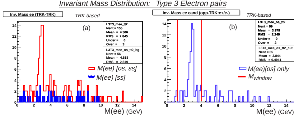
Figure 9.28: Similar invariant mass distribution as Figs. 9.26 and 9.27 for Type 3 pairs. See text for further discussion.
