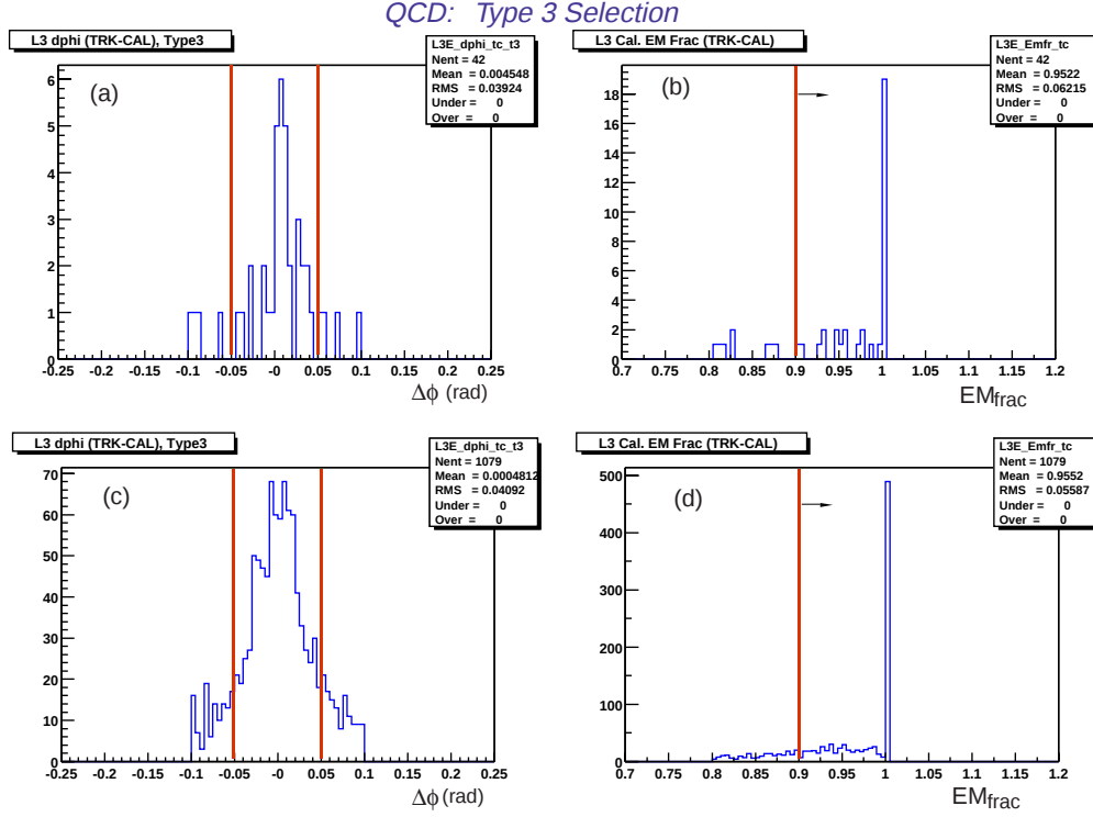
Figure 9.24: Similar distributions as in Fig. 9.23 for Type 3 selections implemented on (a-b) QCD p_T > 2 GeV and (c-d) QCD p_T > 10 GeV samples.
