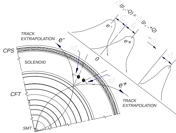
Figure 9.8: Schematic of the bimodal distribution in \Delta\phi observed in the match between the tracker and CPS. See text for further discussion.
