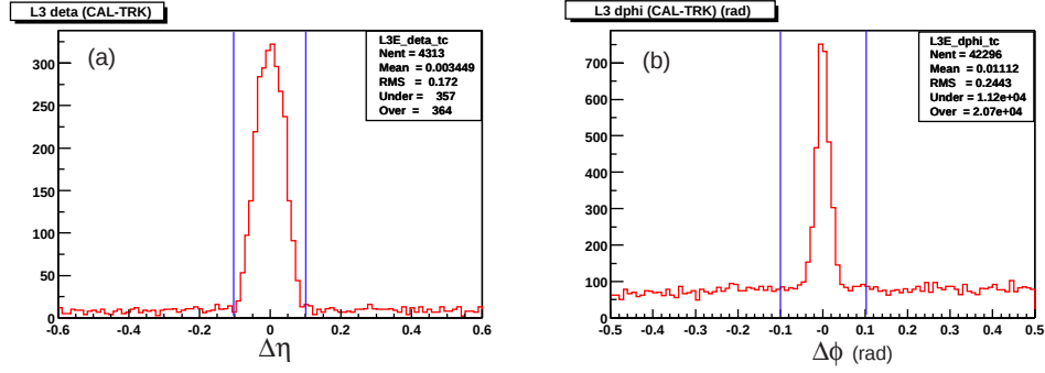
Figure 9.17: Distributions of matching between calorimeter clusters and global tracks for electron selection in (a) \eta and (b) \phi for the J/\psi sample.
