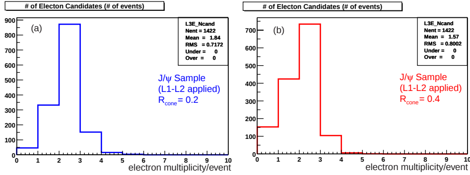
Figure 9.25: Number of candidates per events for J/\psi sample using calorimeter cluster cone sizes of (a) 0.2 and (b) 0.4. In either case, only those events with two or more electrons are used for the invariant mass calculation. Note the improvement in the number of events with two electrons for \Delta R=0.2 .
