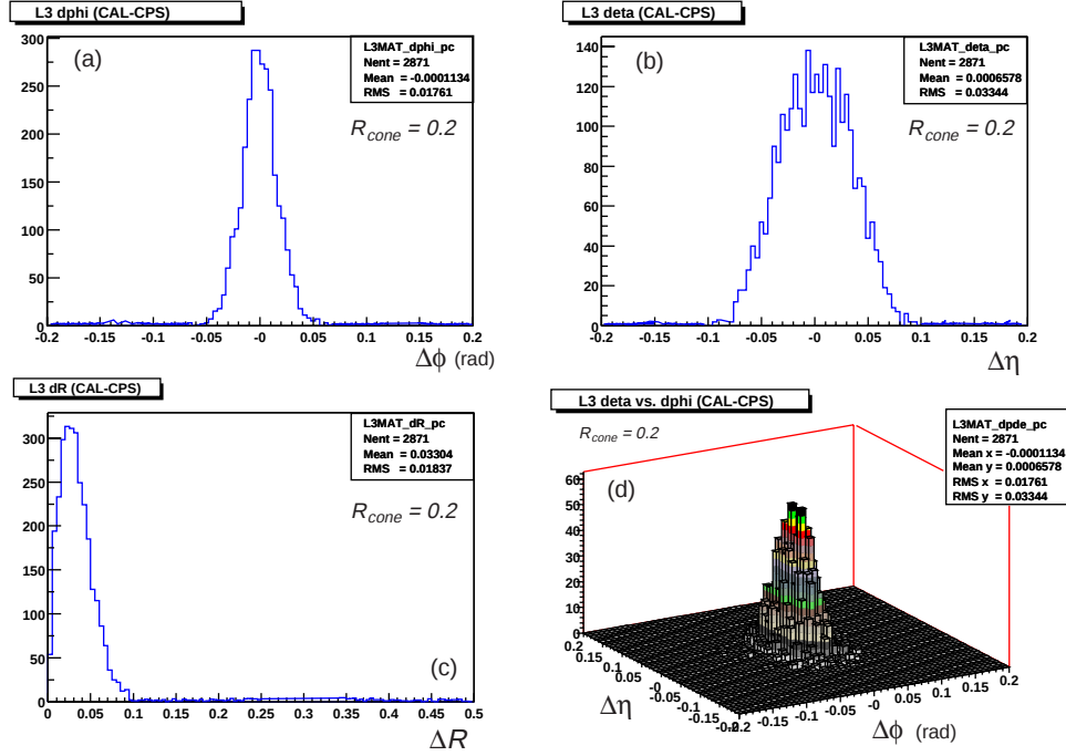
Figure 9.5: Distributions for (a) \Delta\phi , (b) \Delta\eta , and (c) \Delta R for calorimeter and CPS clusters using tagged electrons in the J/\psi sample. Results are for calorimeter clusters with R_{cone} = 0.2 . The correlation in \Delta\eta with \Delta\phi is also shown in (d).
