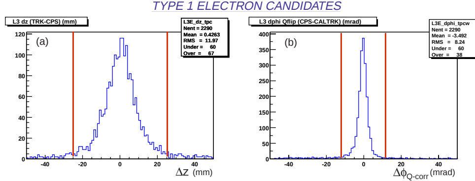
Figure 9.19: Type 1 selection variables and cuts implemented for electron identification on J/\psi sample: track-preshower match in (a) z and in (b) \phi after correcting for magnetic field effects at the CPS radius. Also, shown are the intervals in which selections have been made.
