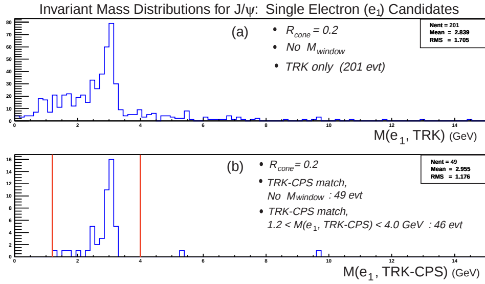
Figure 9.31: Invariant mass distribution for single electron candidates in the J/\psi signal sample paired with L3 reconstructed tracks requiring (a) \eta , \phi , and common vertex conditions. Also given is the corresponding distribution requiring (b) a track-preshower match. The mass window in (b) is shown by the vertical bars.
