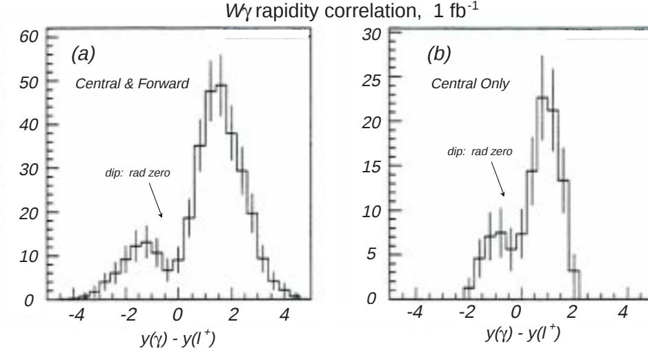
Figure 4.2: Simulations of the photon-lepton rapidity difference distribution for W\gamma production for 1 \text{ fb}^{-1} , using a) central and endcap photons and electrons, and b) central photons and electrons only. Adapted from [58].
