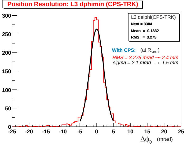
Figure 9.9: \Delta\phi distribution for CPS clusters and tracks after correcting for the offset resulting from the “Q-flip”. The distribution has been fitted to a Gaussian to determine an order of magnitude of the resolution in \phi .
