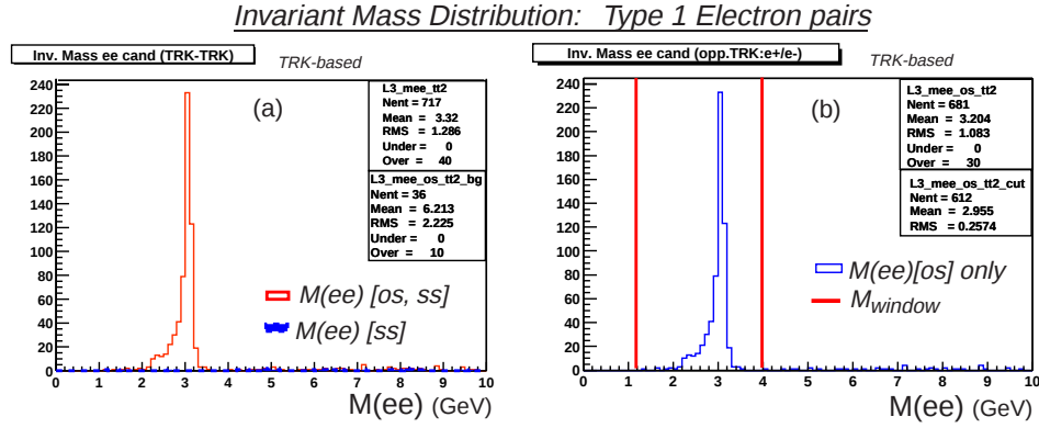
Figure 9.26: Invariant mass distribution for Type 1 pairs using R_{cone}=0.2 . Given is the track-based results for (a) opposite- (os) and same- (ss) sign pairs (open-histogram), and same-sign pairs (shaded-histogram). The distribution in (b) shows results for only os pairs with the mass window shown by the vertical lines. See text for further discussion.
