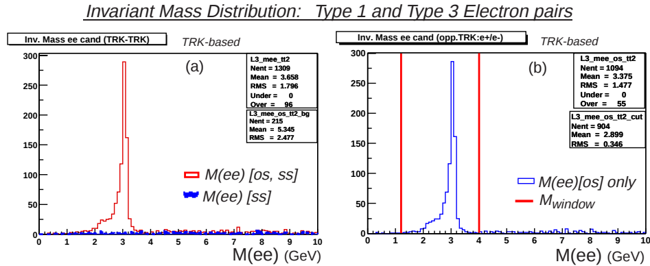
Figure 9.27: Similar invariant mass distribution as Fig. 9.26 for pairs where at least one electron is of Type 1 while the other is either Type 1 or 3. See text for further discussion.
