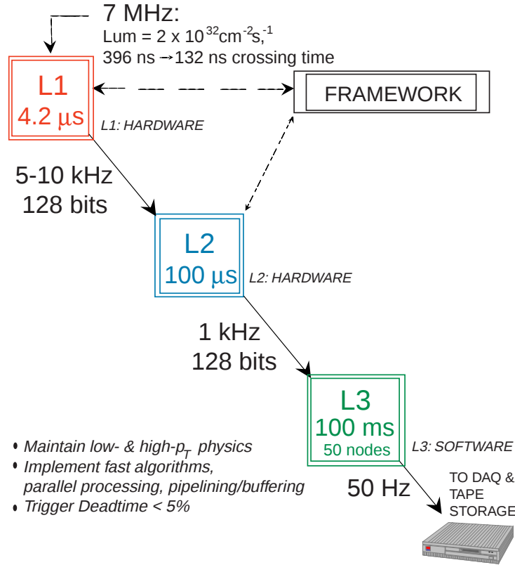
Figure 3.17: Summary of the three-level DØ Trigger System for Run II with the decision time and bandwidth allocated to each level.
