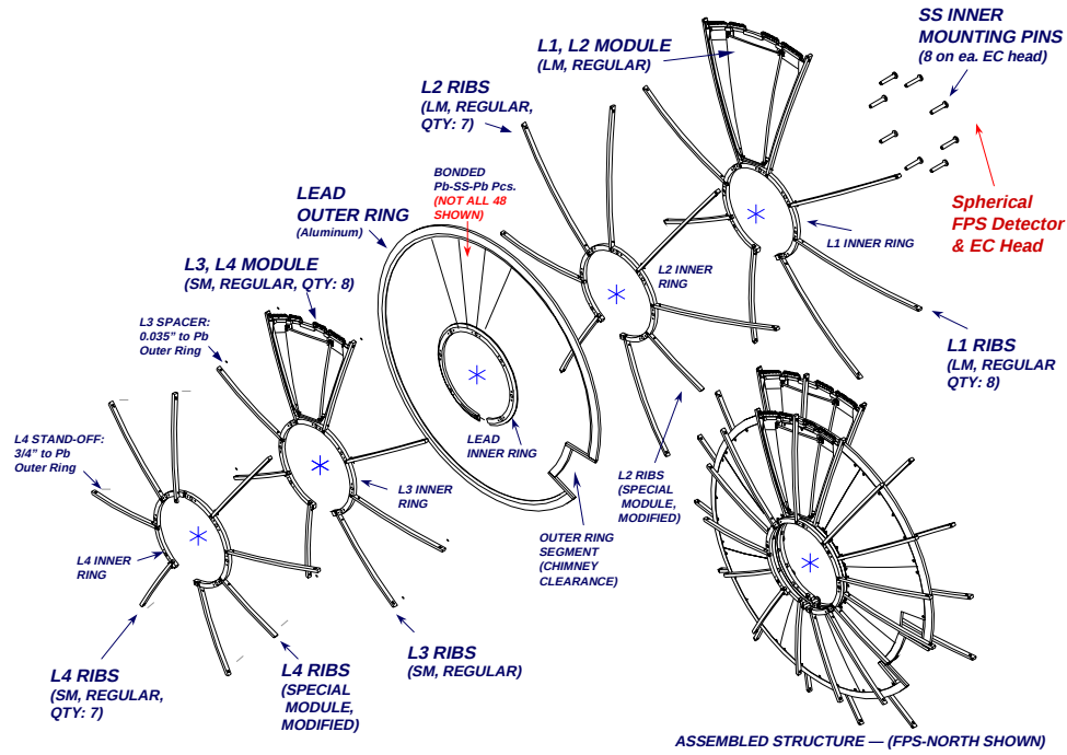
Figure 7.4: Three-dimensional view of the layered FPS support structure assembly. For brevity, all modules and lead pieces are not shown.
