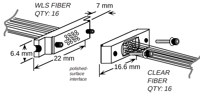
Figure 7.21: 3-D view of detector-side (mating) FPS optical connector assembly and alignment.
