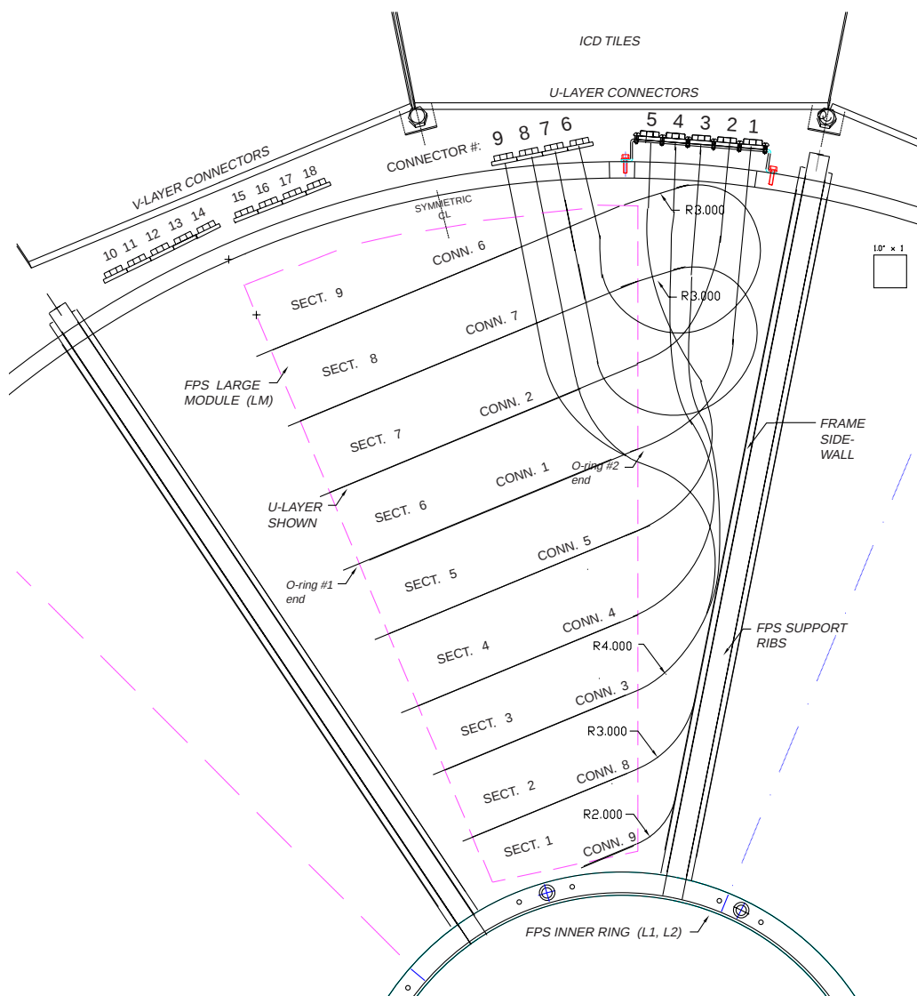
Figure 7.27: An r - \phi view of a large module in L1 or L2 of the FPS, showing the WLS fiber/scintillation strip layout and connector-by-connector mapped routing. Individually labeled connectors are shown at the top and map to sections of 16 contiguous strips on a module's u - or v -sublayer. Cabling for the u -layer is only shown — the v -layer follows in a mirror-symmetric manner.
