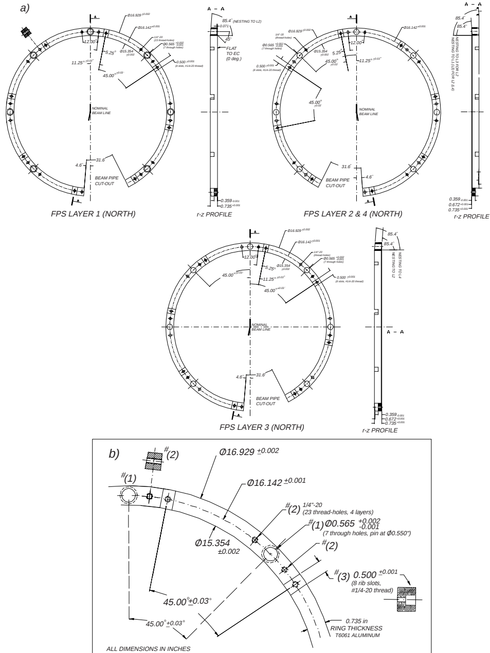
Figure 7.10: Inner support rings for Layers 1–4 (FPS-North). (a) gives each layer’s ring and its respective r – z profile. The rings for L1 and L3 are geometrically similar and only differ in the nesting configuration in the r – z plane. (b) gives a limited, expanded r – \phi view of the different sets of holes used for assembly and mounting, outlined in the text. Rings for FPS-South are a symmetric, mirror-image of the north half.
