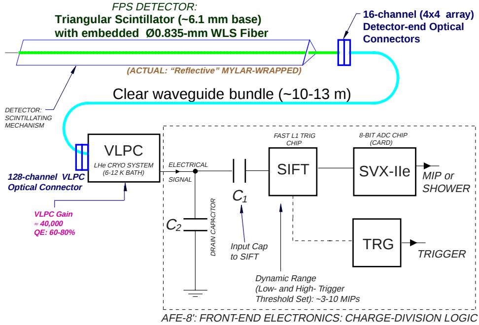
Figure 5.7: Schematic of the FPS readout system.
