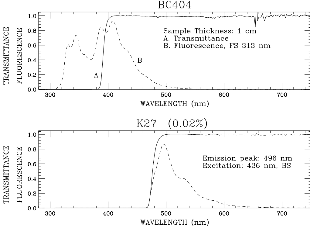
Figure 5.3: Fluorescence spectrum of BC-404 (top) and K27 (bottom). For BC-404, the two peaks near 350 (400) nm are from pT (DPS). The light transmission curve is also given. The light output from BC-404 is a convolution of the emission and transmission curves. For K27, the emission peak includes the effects of self-absorption and is at \sim 500 nm. Adapted from [54].
