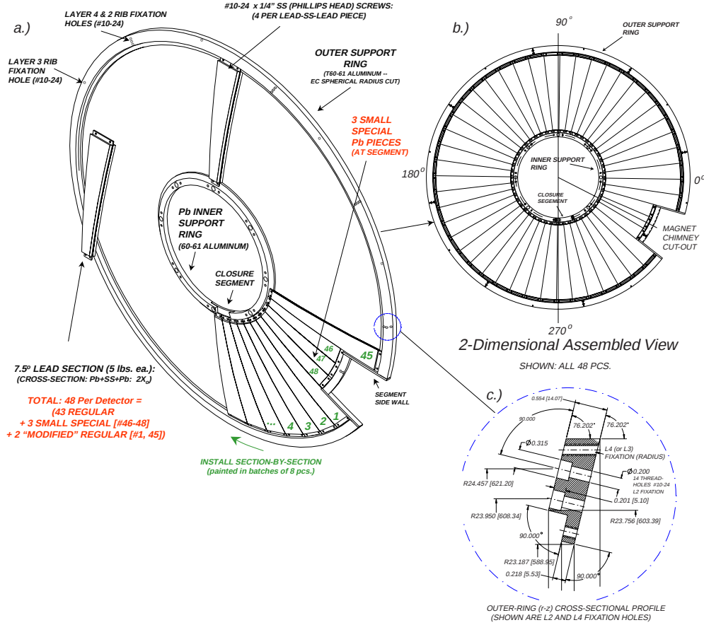
Figure 7.20: Lead layer support assembly showing bonded pieces mounted between inner- and outer-support rings. A 2-D projection of the completed layer (b) and a close-up of the outer-ring's cross-sectional profile (c), which follows the L2 rib's spherical profile are given.
