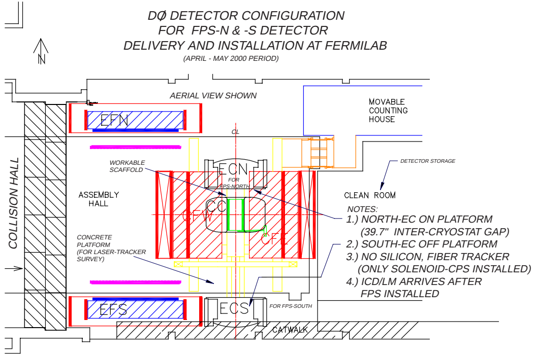
Figure 8.5: Configuration of the DØ Detector during the FPS installation period at Fermilab. See notes in figure and text for a description of the scenario available for preshower assembly and installation.
