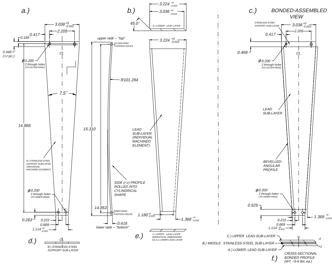
Figure 7.16: Lead absorber design using 7.5° wedge-like elements: (a) and (b) shows the front r\text{-}\phi view of the stainless-steel support unit and lead sub-layer, respectively, as individual elements, while the assembled view is given in (c). A cross-sectional profile of each component is given in (d), (e), and (f), respectively.
