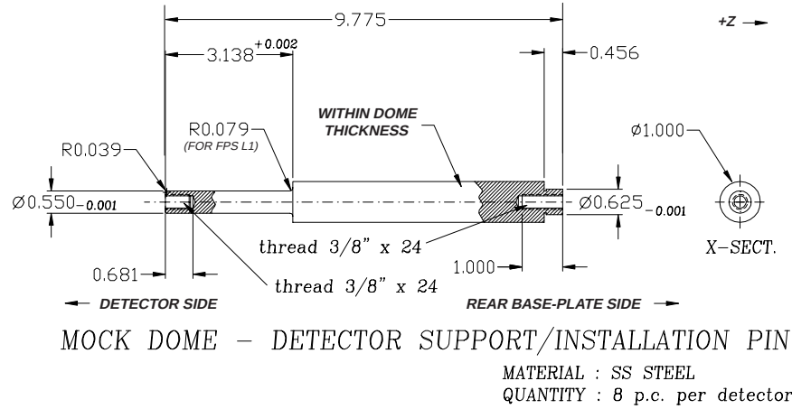
Figure 7.8: Detector inner support pins mounted within the wooden dome/base plate assembly. The pins support the FPS inner ring structure outlined in Sec. 7.2.3.
