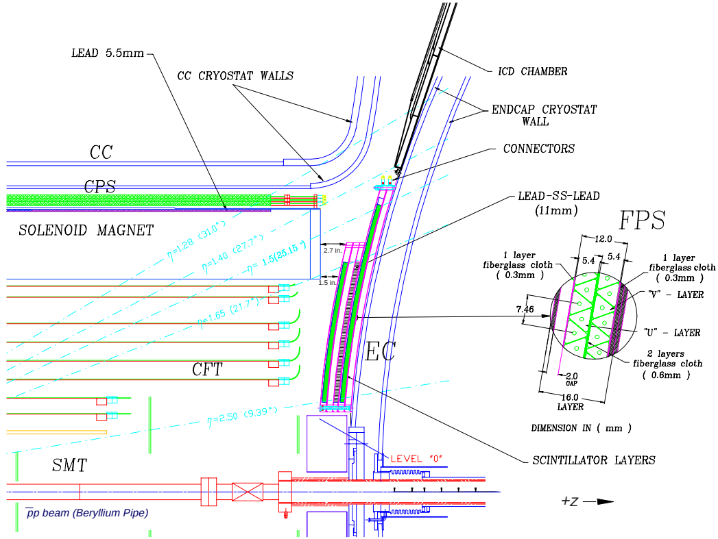
Figure 6.3: Cross-sectional r - z view of the FPS detector at DØ. Given within the inset is a module's triangular strip nesting configuration.
