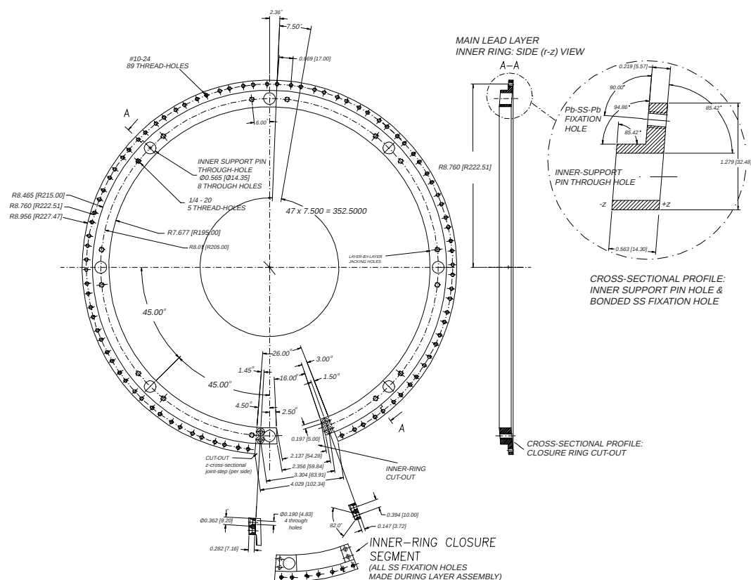
Figure 7.19: Precision-machined lead layer's inner support ring with closure segment. Shown are the eight through-holes that mate to supporting inner pins welded on EC wall as well as a cross-section (insert) illustrating the ring's r - z surface. In order to properly nest and anchor a cylindrically-shaped Pb-SS-Pb element, an angular profile is needed on the surface. Note: all fixation holes on the closure segment are made in situ during actual lead layer assembly.
