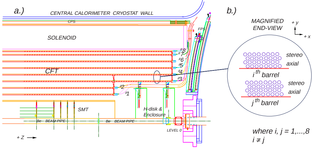
Figure 3.6: Quarter r - z view of CFT detector as installed at D\phi . Shown is a) the nested eight barrel configuration of the device, A magnified r - \phi end-view of the two ribbon doublet layers per barrel is also given in (b).
