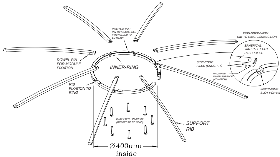
Figure 7.11: View of FPS supporting unit for independently constructed modular frames. Shown is an inner ring with machined slots to attach the support rib array. Modules for all subsequent active layers are supported in a similar manner.
