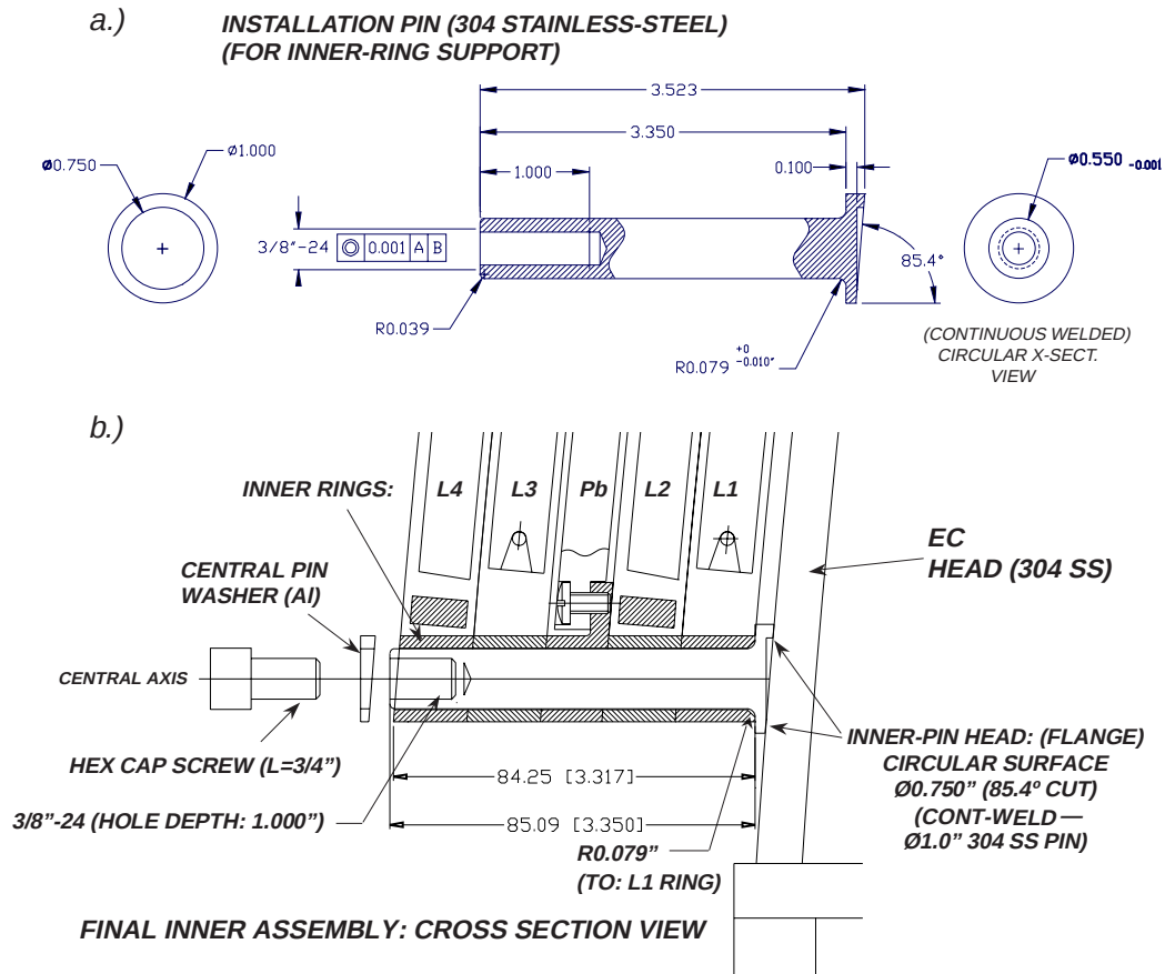
Figure 8.2: a) Stainless-steel FPS inner-support pin with dimensions and b) cross-sectional view of nested FPS layers and inner pin assembly. Eight such pins are aligned and welded on each cryostat head to support the detector.
