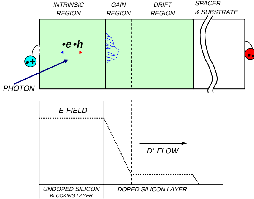
Figure 5.8: Cross-sectional illustration of VLPC operation (top) and corresponding electric field profile (bottom).
