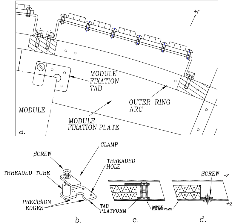
Figure 7.14: (a) An r - \phi view of the outer edge of a layer, showing the means of module fixation within individual supporting frames using aluminum fixation tabs. Each module is held in place in an identical manner at each of its four corners. Also shown are b) and c) details of the fixation tab attached to the surface of a corner fixation plate with pan-head screws in (d). The threaded tube stand-off is held to the tab's platform using a flat-head screw on the +z surface.
