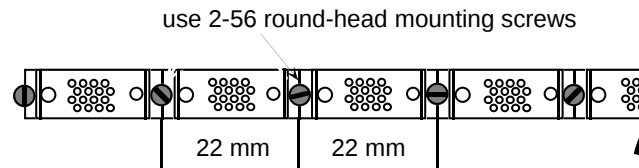
Figure 7.24: \phi - z view of the single row connector mounting configuration in each FPS module.
