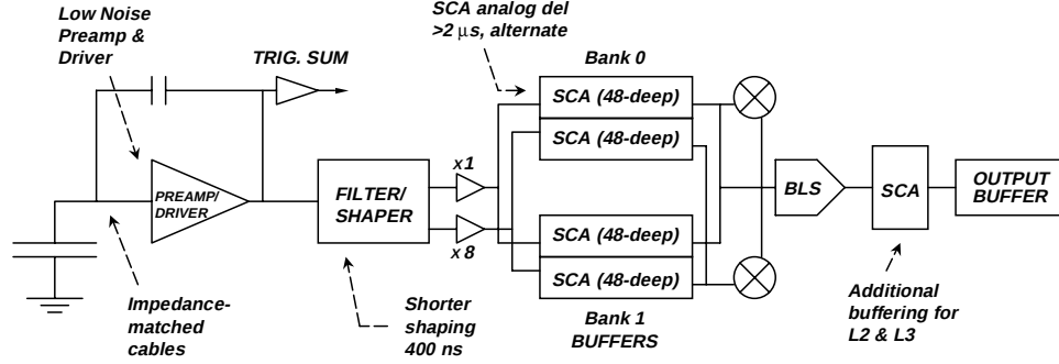
Figure 3.13: Schematic of the primary elements for the DØ calorimeter electronics.
