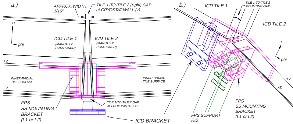
Figure 8.9: 3-D frame view in (r, z, \phi) illustrating two ICD tiles nested on the EC wall. Shown are: a) a view from the innermost z -surface of two panels and b) a similar forward angular view. The brackets supporting the ICD are designed to securely fit within the gap existing between tiles.
