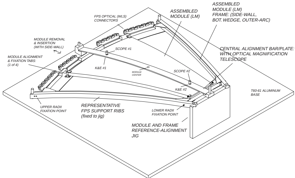
Figure 7.13: Three-dimensional view of alignment jig used to assemble and align module frames and each element. Details are given in the text.
