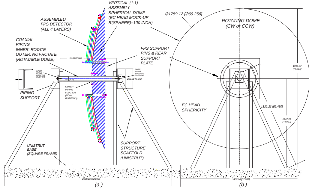
Figure 7.9: Vertical mounting of the mocked-EC head for final testing of the assembly procedures prior to installation at DØ. Shown are: a) r - z view and b) r - \phi view. To facilitate module insertion and removal, the dome is made to rotate about a central axis.
