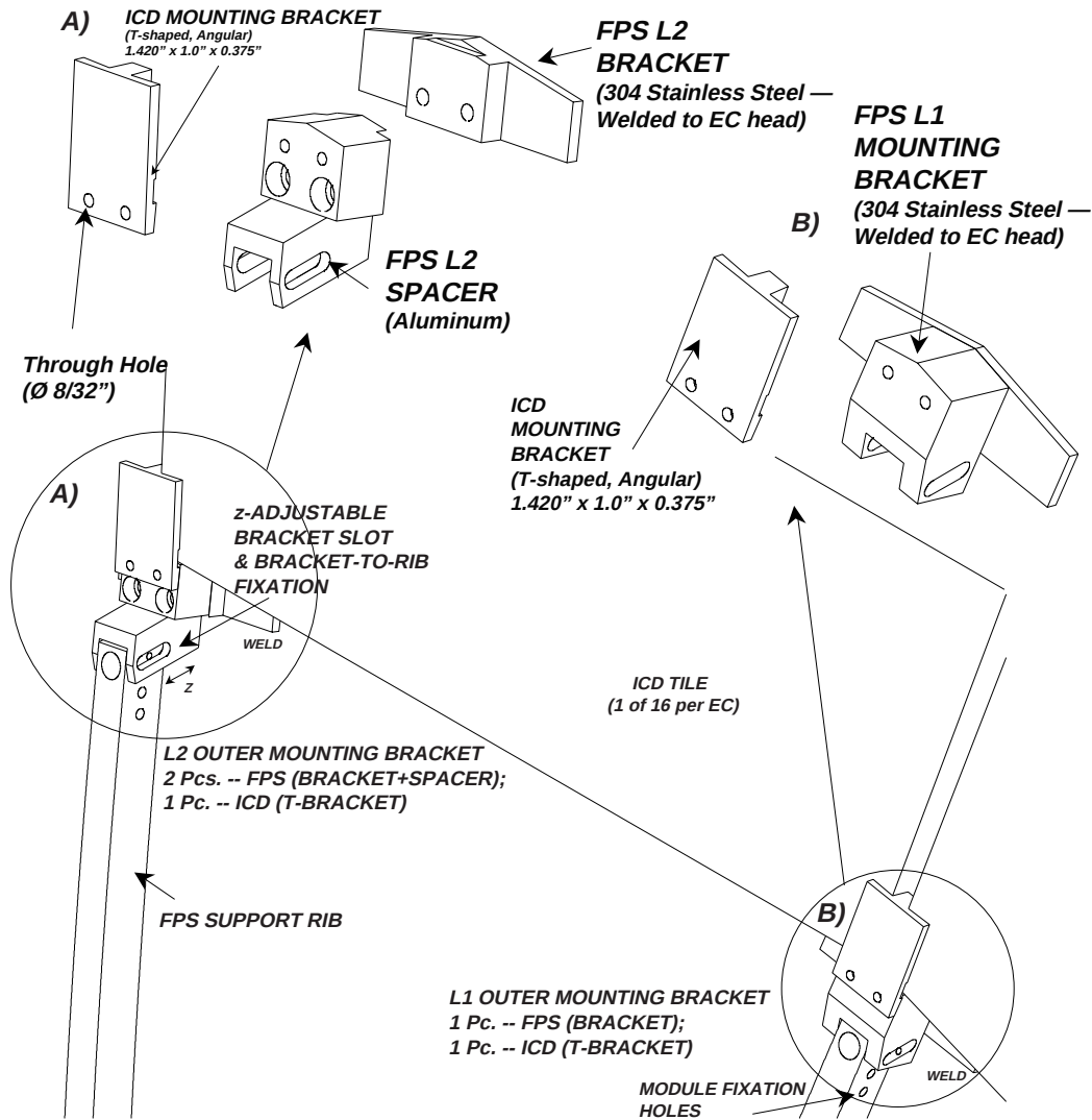
Figure 8.3: Welded stainless-steel brackets supporting the FPS support rib and detector structure at its outer radial periphery on the EC head. Shown are a) FPS L2's (two-piece) bracket and spacer as well as b) L1's (one-piece) bracket. At both L1 and L2, an equivalent T-shaped aluminum bracket (a) and (b) allows for a coupled ICD and FPS support.
