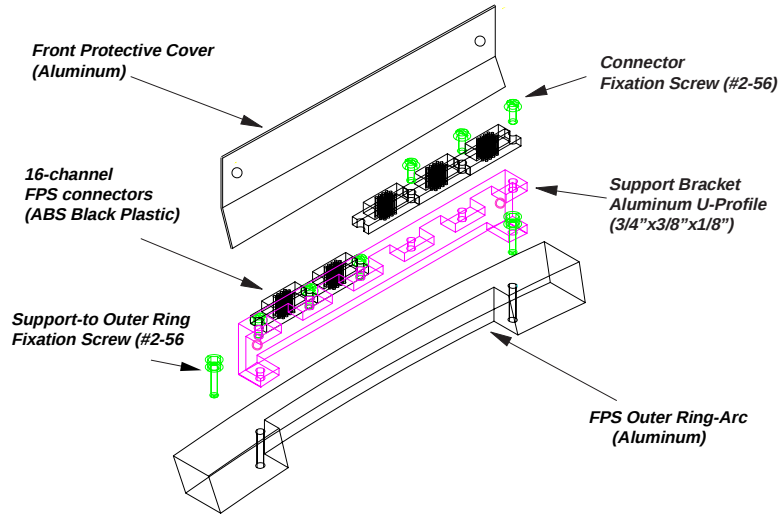
Figure 7.6: Section of FPS outer arc supporting optical connectors and required brackets, all protected by a 1/16"-thick aluminum covering plate.
