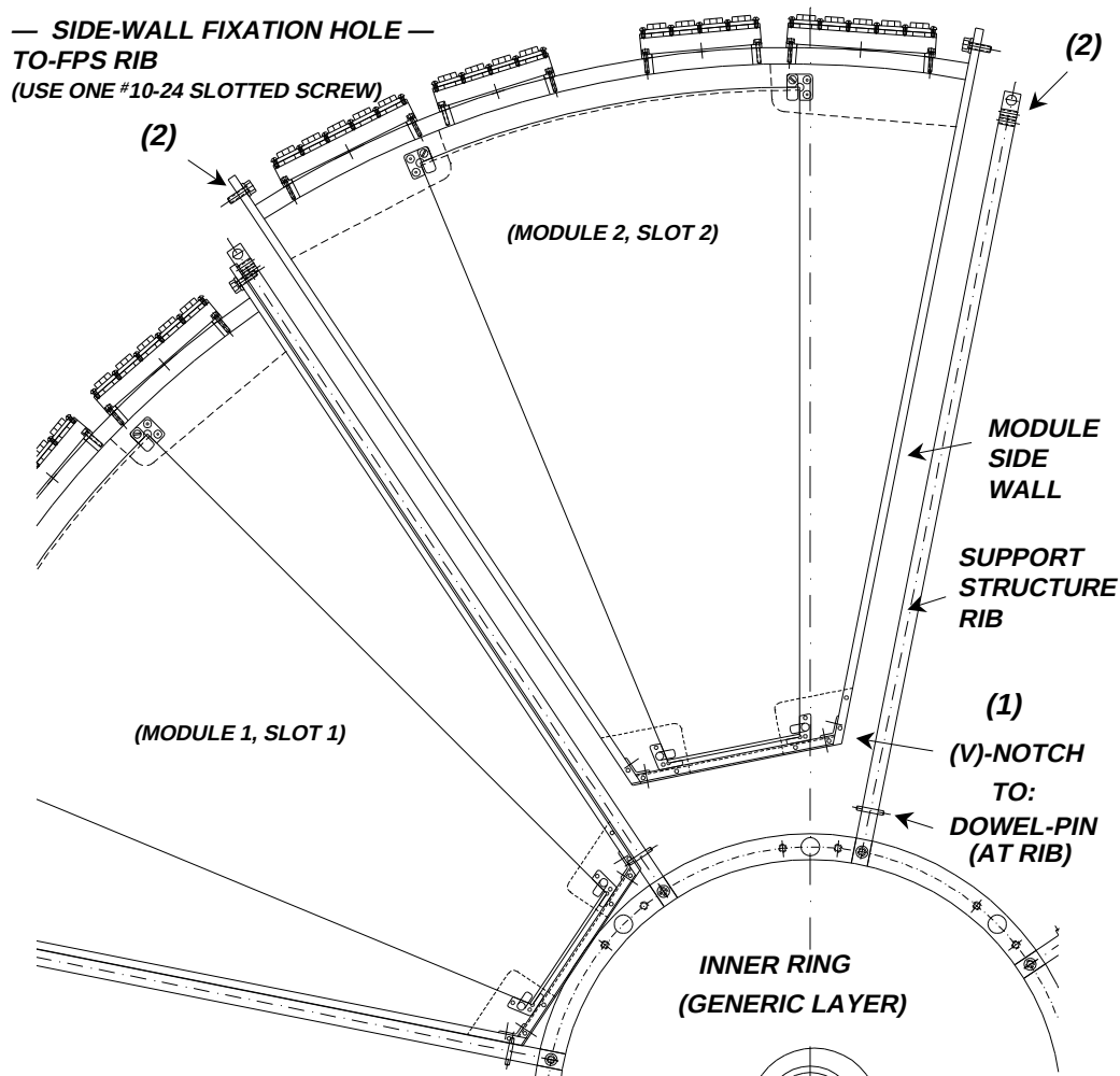
Figure 7.12: Module insertion process into FPS support structure. The lower radius of the module is inserted first until its v-notch rests on dowel pins attached to each rib (1), and the full unit is pitched about z for holes at (2) to be aligned and bolted.
