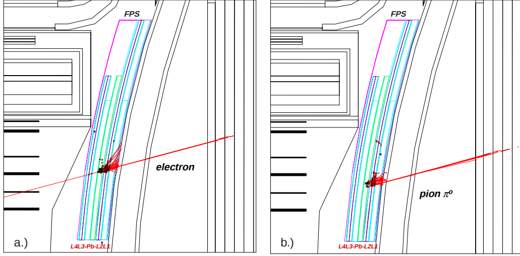
Figure 6.2: Typical GEANT simulated signature of 50 GeV a) electrons and b) neutral pions traversing the FPS detector.
