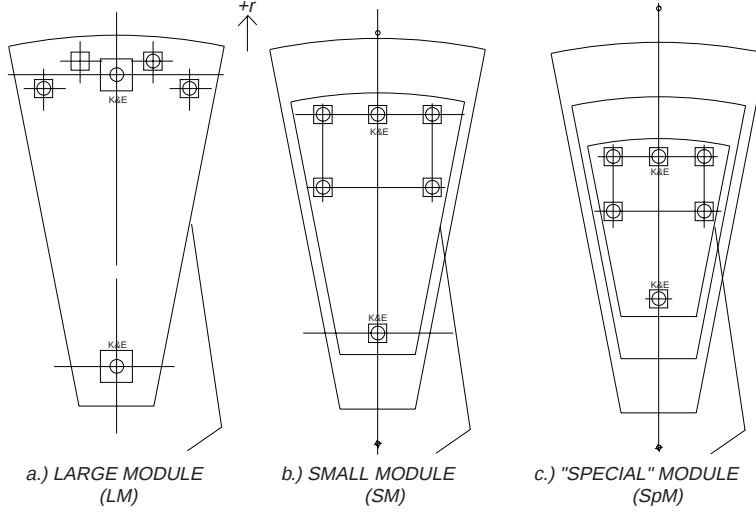
Figure 6.7: The three different types of representative FPS modules: a) Large Module (LM), b) Small Module (SM), and c) “Special” Module (SpM).
