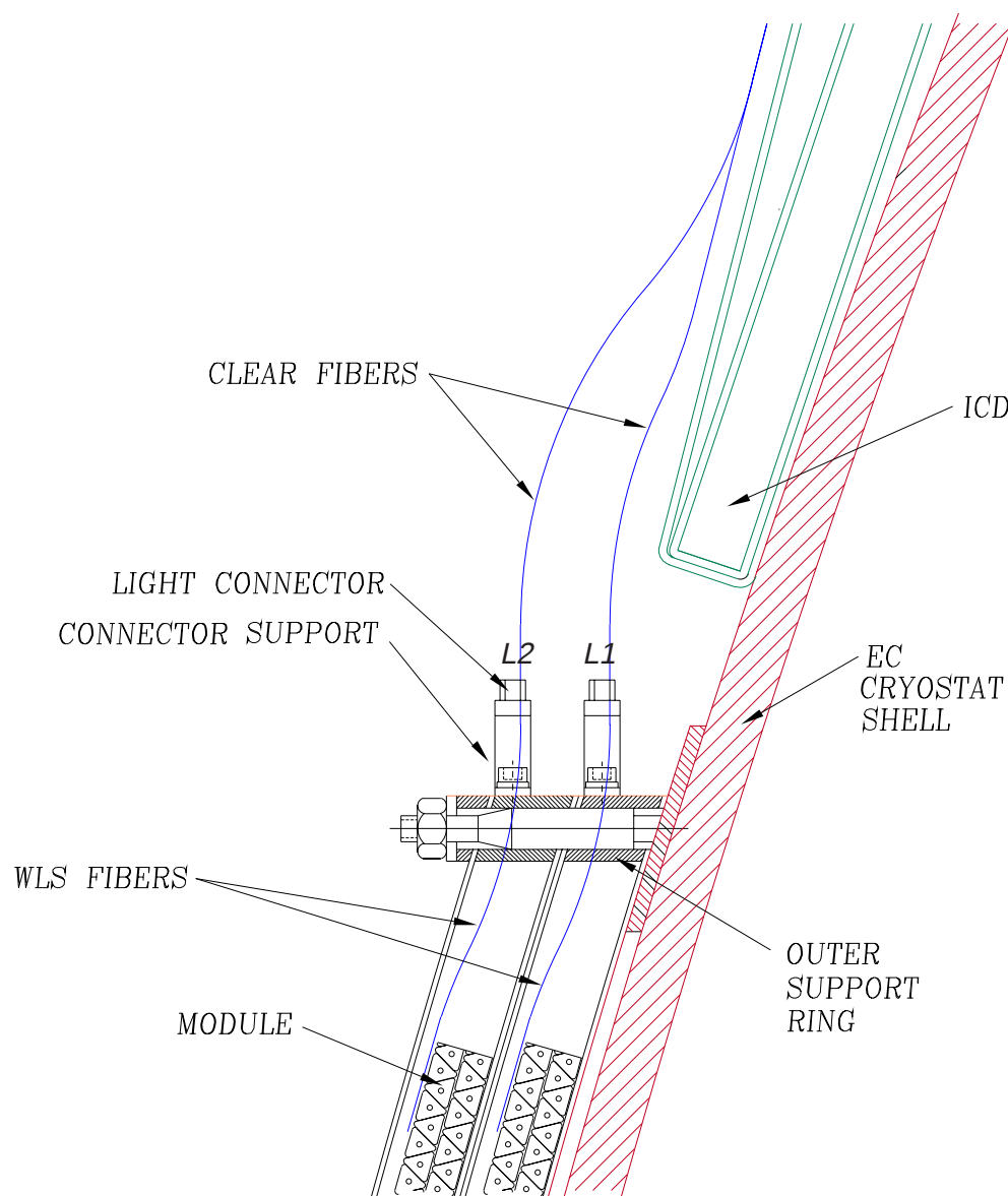
Figure 7.25: r - z view of FPS connectors at the outer periphery of Layers 1 and 2. An angular pitch to these connectors is made for waveguides to clear the existing ICD tiles at this radius.
