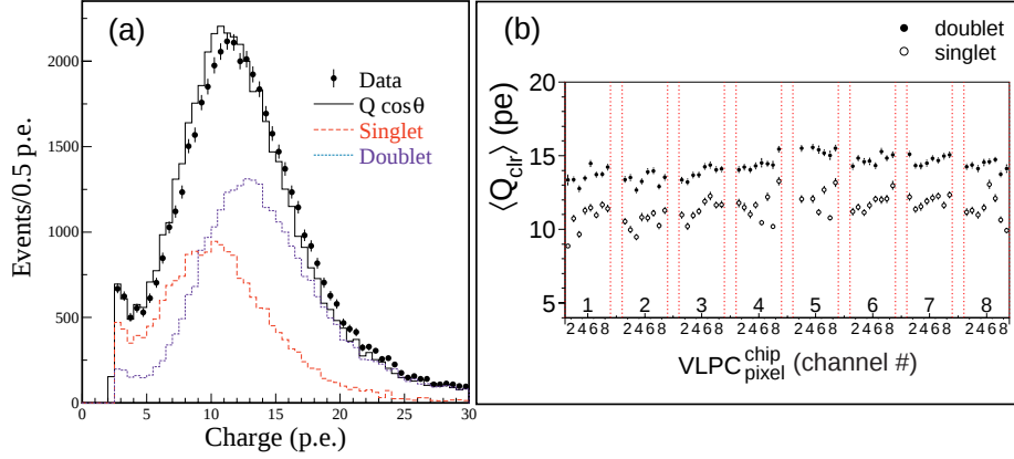
Figure 5.10: Measurement of preshower light-yield for MIPs (a) in a cosmic ray system setup. Shown are data corrected for \cos \theta (solid line) as well as singlet (dashed) and doublet (dotted) extrapolations. Charge uniformity, mean charge vs. channel number, is given in (b). Distributions represent results using final scintillator strips, WLS fibers, 11.0 m clear lightguides, and VLPCs.
