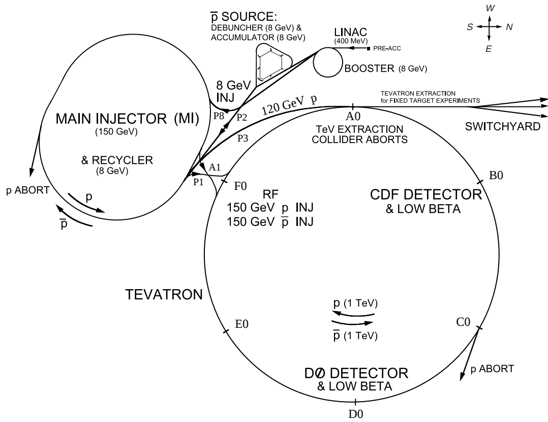
Figure 3.1: Schematic of the Run II Fermilab accelerator complex. Adapted from [20].
