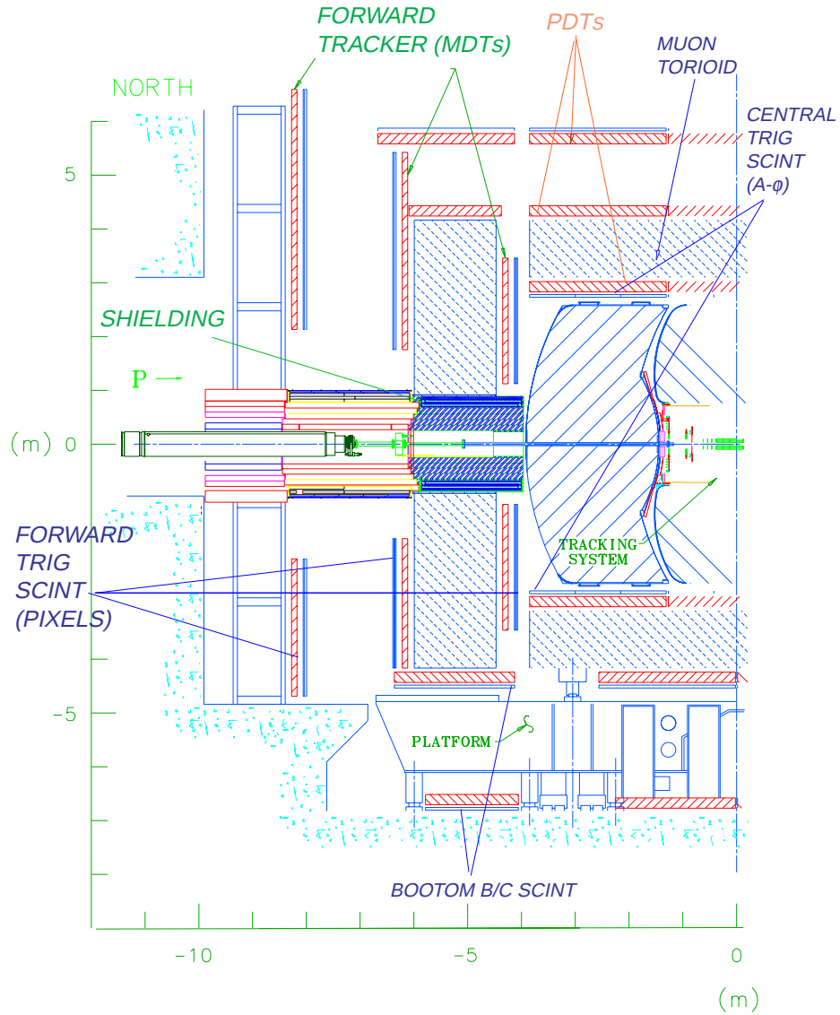
Figure 3.14: r - z half-view of the Muon System. Components of both the Forward and Central systems are shown.
