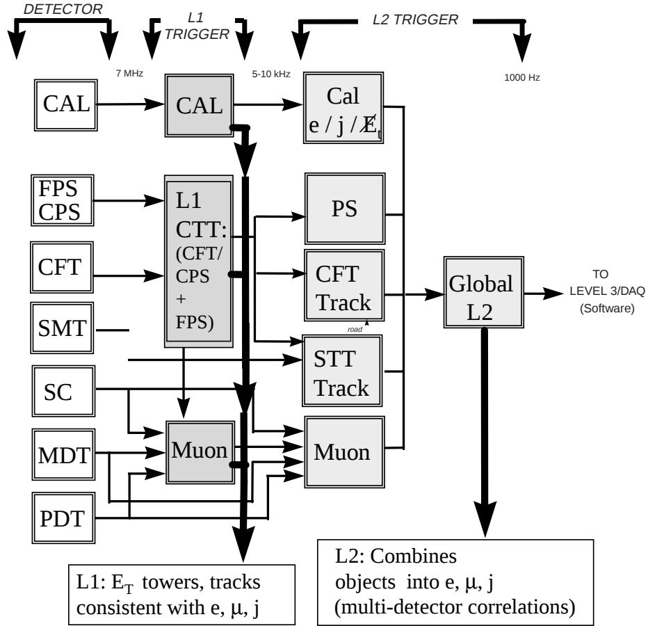
Figure 3.18: L1 and L2 trigger data pathway. The arrow indicates the direction of data flow. Multiple arrows from a particular subsystem are present for parallel processing of detector information and thus, to permit fast trigger decisions and sophisticated physics filters.
