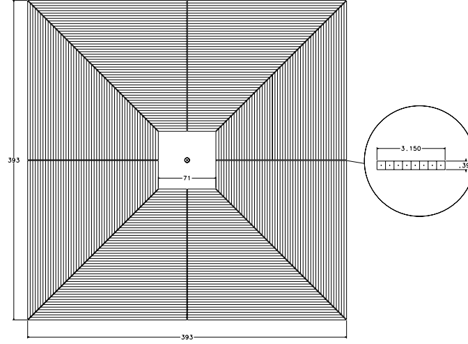
Figure 3.15: Illustrative view of one r - \phi plane in the muon mini-drift tube. The insert shows the cross section of a single Iarocci tube, which consists of eight 1 \times 1 cm 2 cells.
