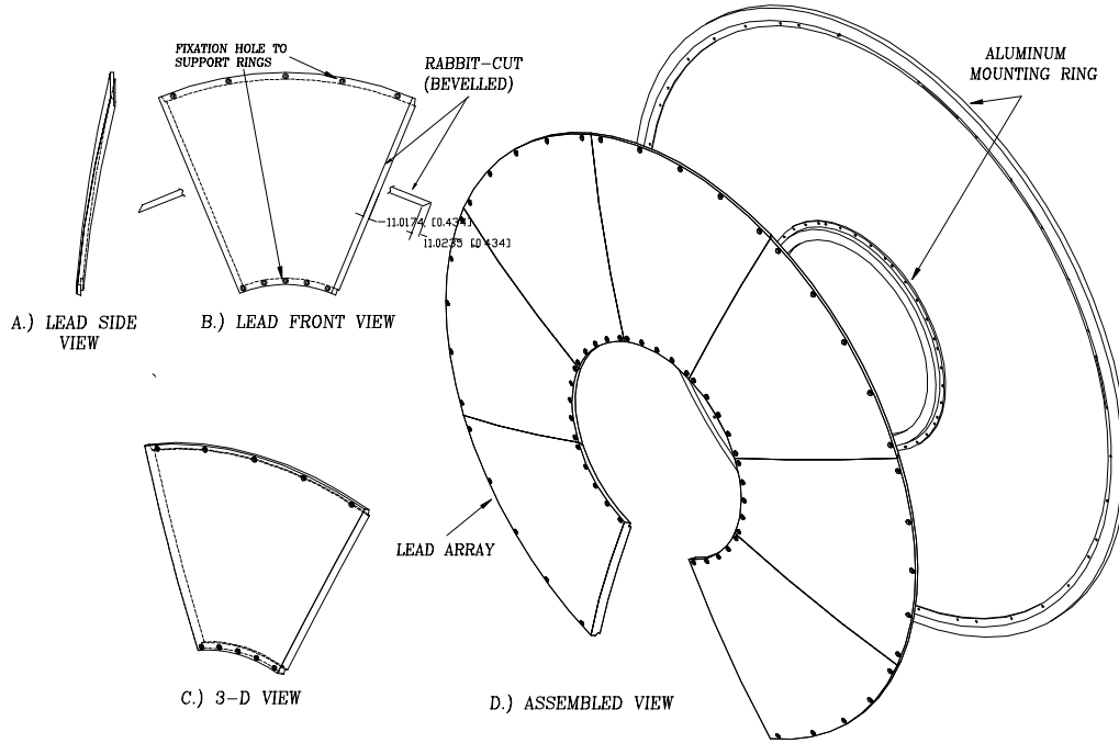
Figure 7.15: Lead absorber layer design with eight 45^\circ wedge-like elements: (a), (b), and (c) showing the side, front, and three-dimensional views, respectively, including the beveled “rabbit-cut” on the \phi -edges of each absorber. This ensures (d) nesting with adjacent pieces, and thus, full coverage.
