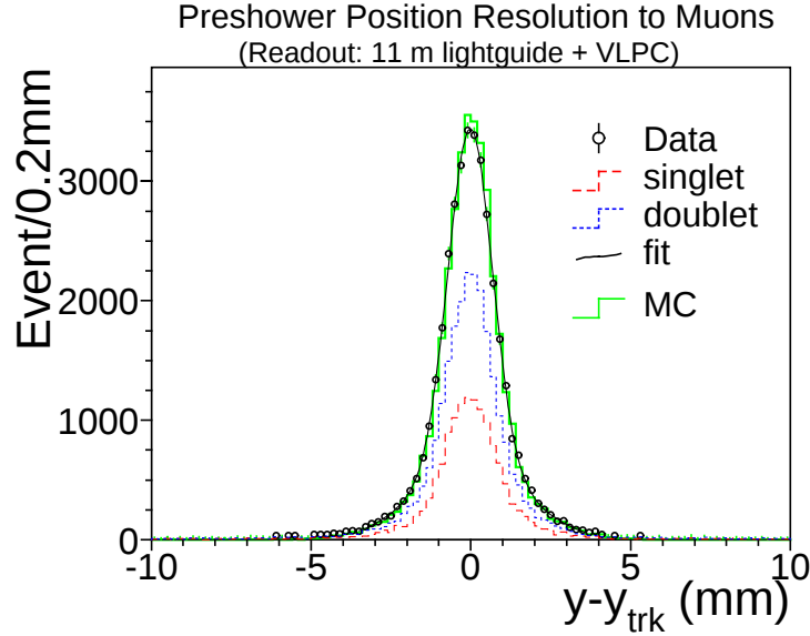
Figure 5.6: Residuals for preshower cluster position relative to a PDT track used to measure the spatial resolution for MIPs in a module readout by 11.0 m lightguide and VLPCs. Shown are distributions for both singlet (dashed) and doublet (dotted) tracks (see text for definitions) as well as the data (circles) fitted to double-Gaussian (solid). MC simulations are shown in histograms.
