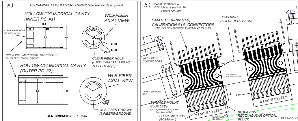
Figure 7.28: LED calibration and monitoring system. Shown are: a) a hollow-cylindrical cavity grouping sixteen WLS fibers and b) the surface-mounted LED pulser boards supplying the signal. Cavity 1 and 2 in (a) are mated and aligned together, being fixed with five-minute epoxy between their outer and inner cylindrical walls, respectively.
