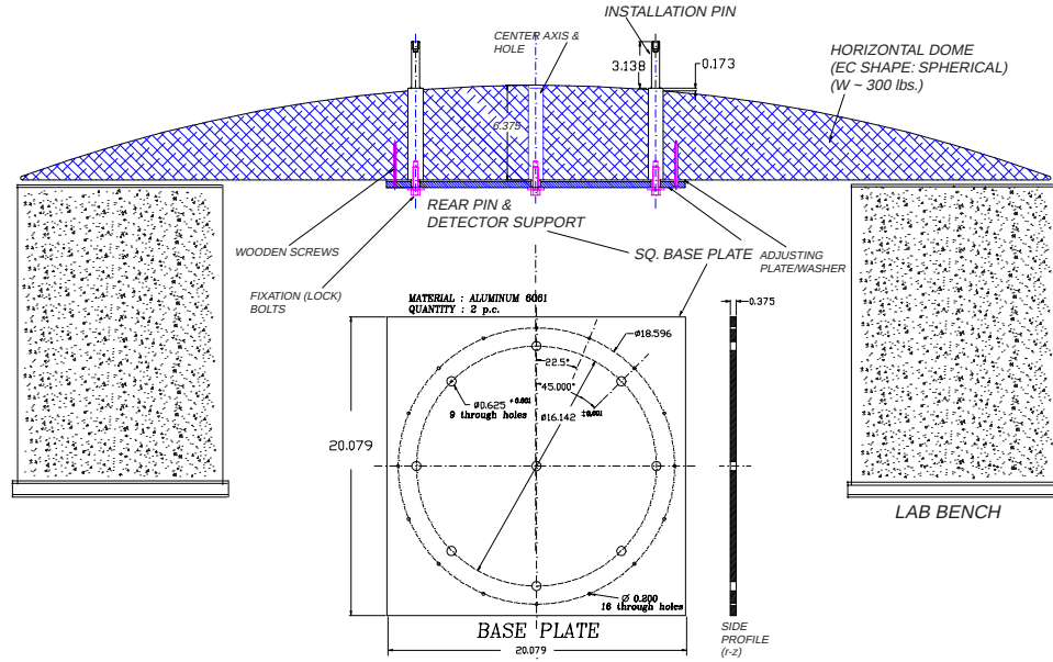
Figure 7.7: One-to-one assembly of DØ EC head for detector assembly during FPS construction. The eight stainless steel support pins mounted on the dome are supported by the adjustable rear base-plate aligned on the dome.
