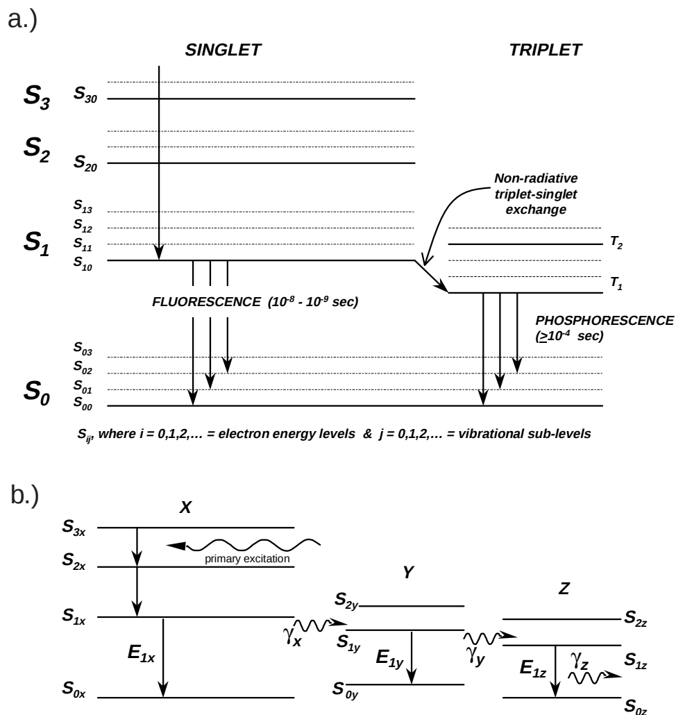
Figure 5.1: Representation of energy levels indicating the fluorescence mechanism in a scintillator. Shown are: a) the \pi electron energy levels participating in scintillation light and b) the energy transfer process in a scintillator from a solvent (X) with two fluors (Y & Z). Adapted from [62].
