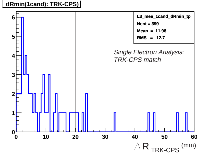
Figure 9.30: \Delta R matching distribution for L3 tracks and preshower clusters needed for single electron candidate and L3 track pairing. Value for the cut has been chosen to help suppress QCD backgrounds during invariant mass reconstruction.
