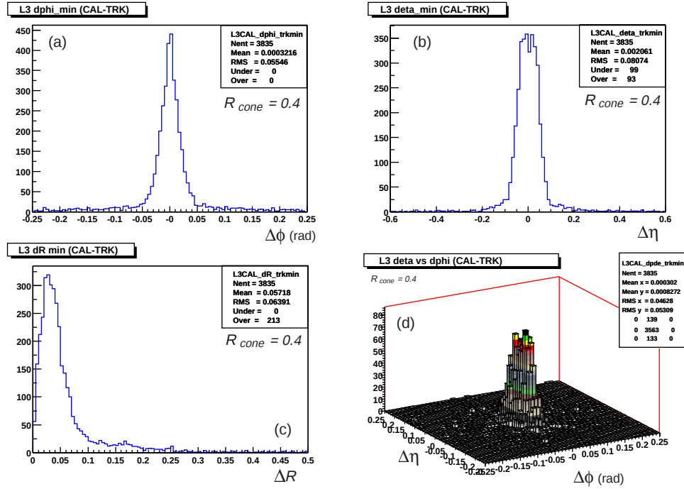
Figure 9.3: Distributions for (a) \Delta\phi , (b) \Delta\eta , and (c) \Delta R for tagged electrons in global tracks and calorimeter clusters in the J/\psi sample for R_{cone} = 0.4 . The correlation in \Delta\eta with \Delta\phi is also shown in (d).
