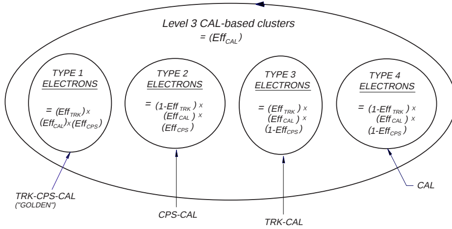
Figure 9.16: Schematic of the Level 3 algorithm for electron identification and selection. The sum of the efficiencies for the electron categories Type 1 through 4 yield the total calorimeter efficiency, Eff_{CAL} .
