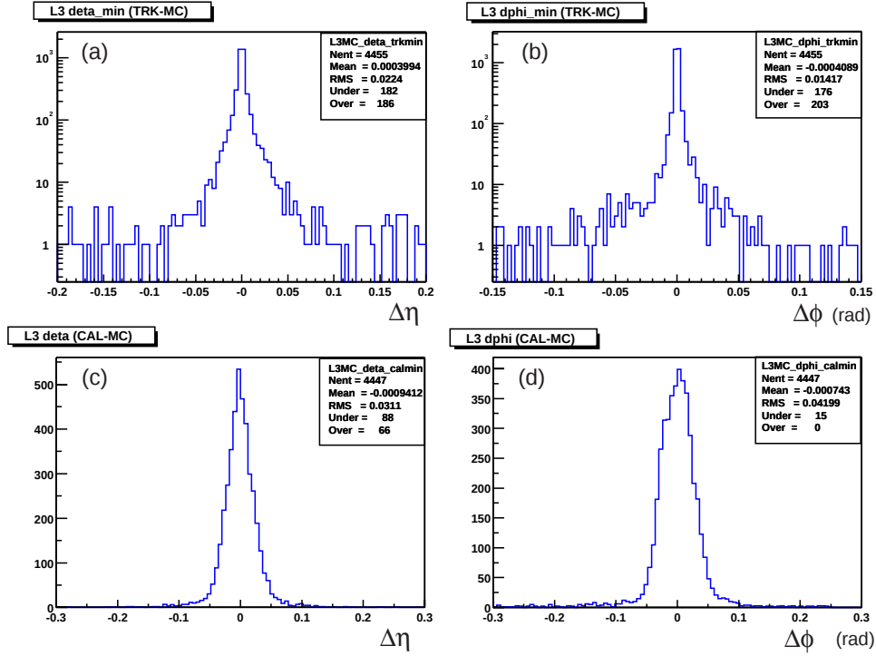
Figure 9.1: Matching resolutions in \eta and \phi for MC electrons with (a-b) global tracking ( i.e. , CFT and SMT) and (c-d) calorimeter, respectively.
