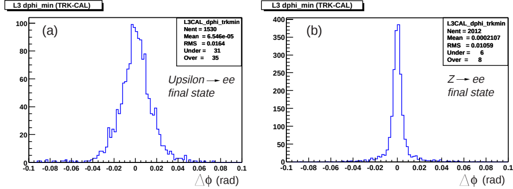
Figure 9.4: \Delta\phi distribution for electrons matched in the global tracker and calorimeter for (a) \Upsilon \rightarrow ee and (b) Z \rightarrow ee final states.
