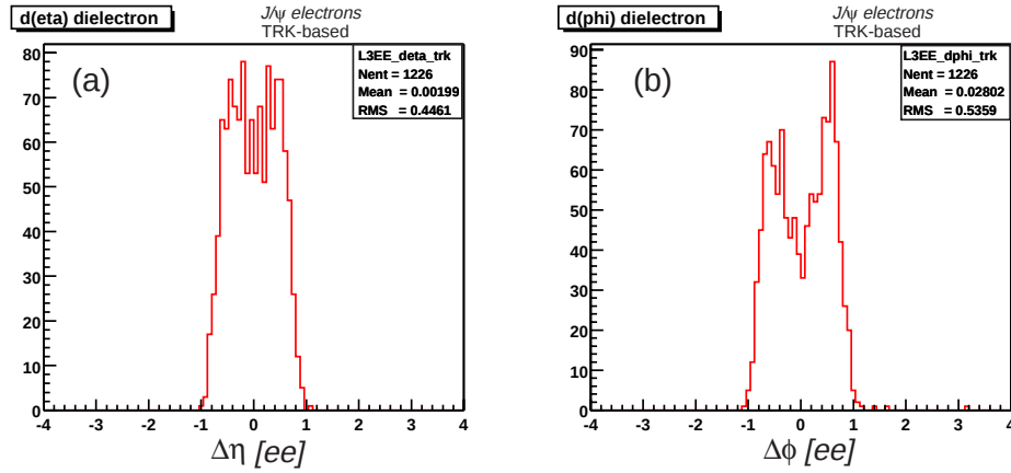
Figure 9.11: Separation of electron pairs from the J/\psi in (a) \eta and (b) \phi .
