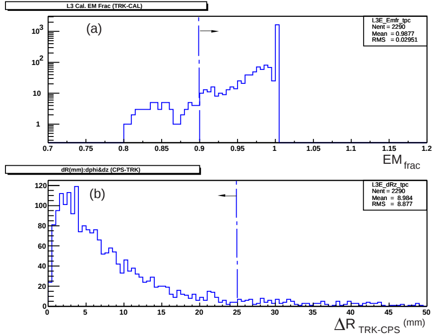
Figure 9.21: Miscellaneous selection variables studied for Type 1 electrons from the J/\psi : (a) calorimeter EM_{frac} and (b) \Delta R match between a track and preshower cluster. See text for complete discussion.
