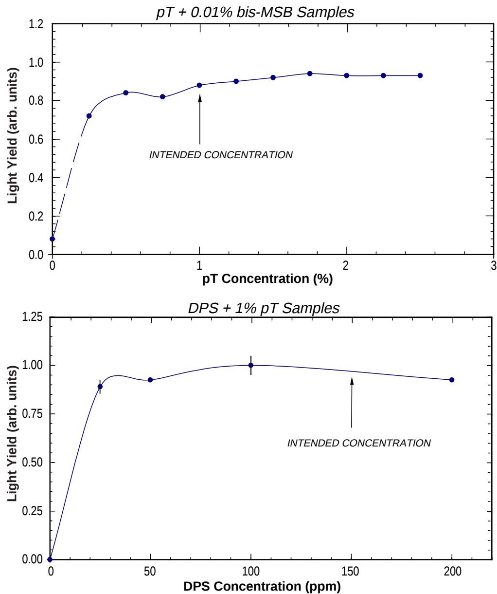
Figure 5.4: Chosen concentrations of scintillating fluors, pT (top) and DPS (bottom) for extruded scintillating strips. The concentration mixtures are determined on the basis of approximating BC-404 scintillator as well as aiming to minimize light re-absorption. Adapted from [67].
