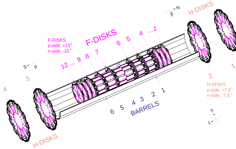
Figure 3.3: Three-dimensional view of the DØ silicon microstrip tracker.
