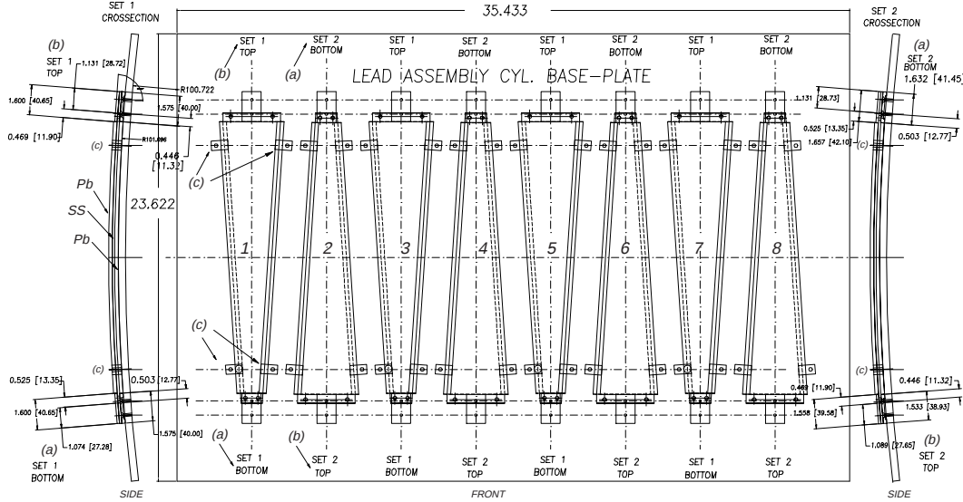
Figure 7.17: Lead base-plate and tooling hardware used for Pb-SS-Pb bonding and production. See text and Fig. 7.18 for description of tooling items (a), (b), and (c).
