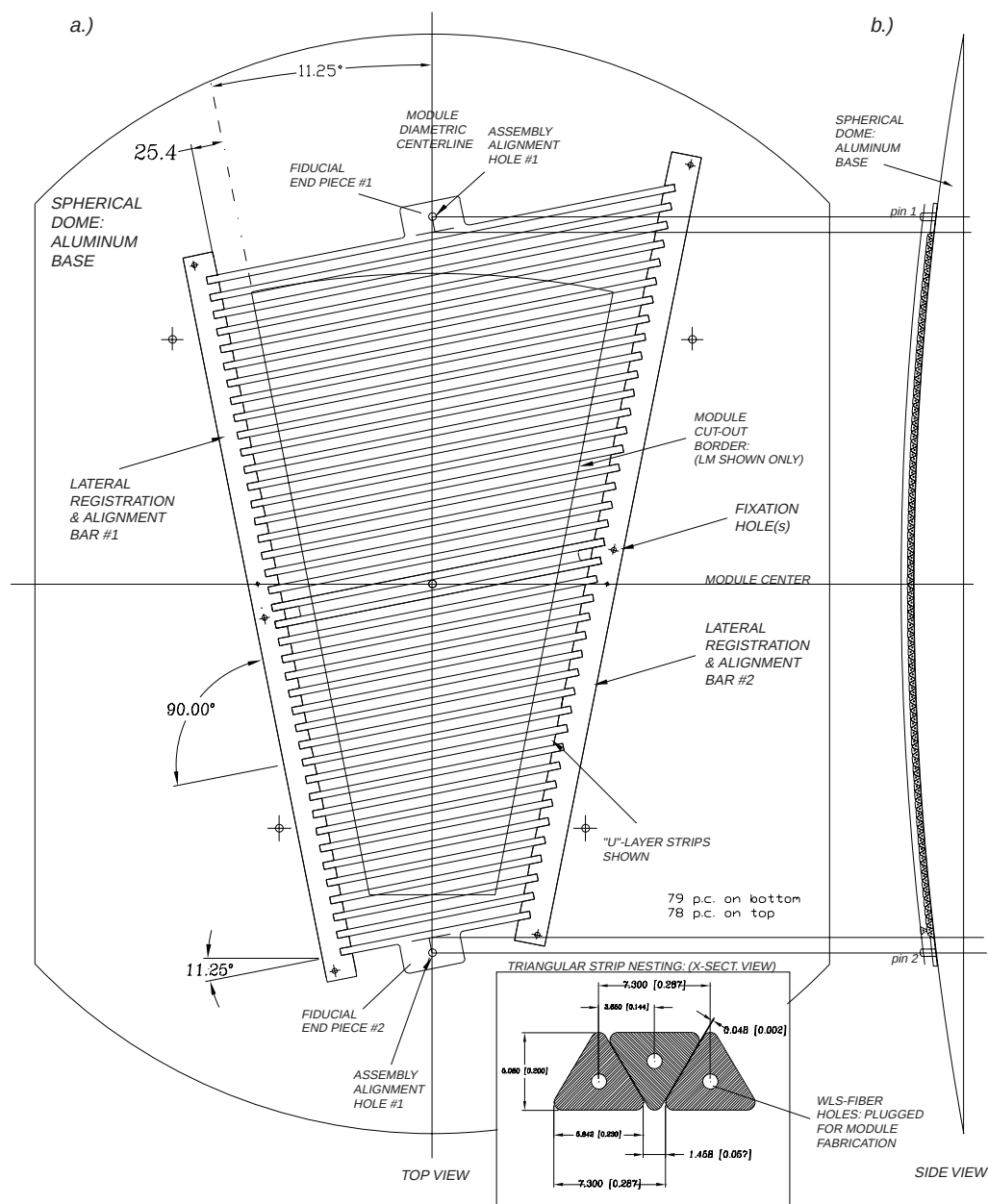
Figure 7.1: Schematic of module fabrication: strip-by-strip layout, registration and alignment on the spherical template dome is shown. Given are a) top r - \phi modular view including the “nested” triangular strip cross-section and b) side r - z profile of assembly.
