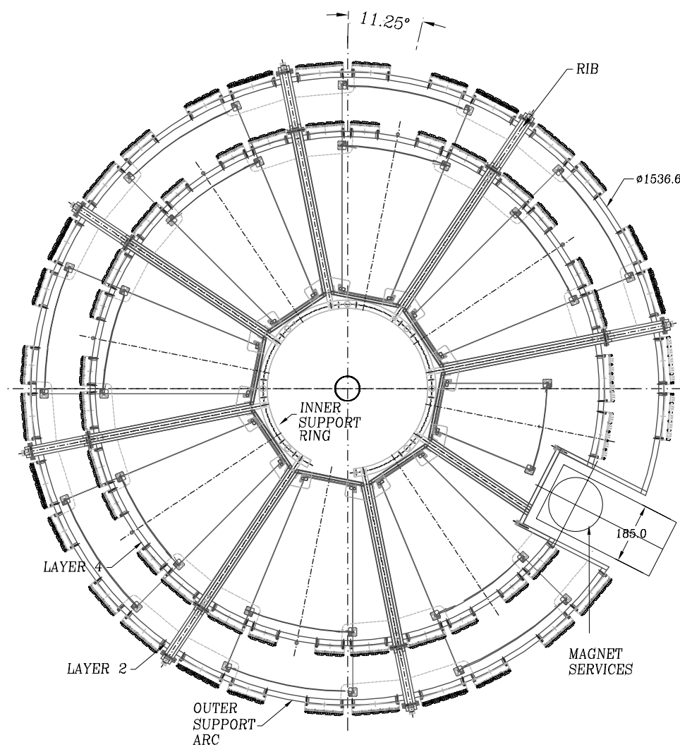
Figure 6.6: r - \phi view of the North-FPS detector. For brevity, only (nested) Layers 2 and 4 are shown; Layers 1 and 3 are rotated by 22.5^\circ in \phi with respect to these layers. Also, the South-FPS is not given here, as it is a symmetric, mirror-image of the north detector.
