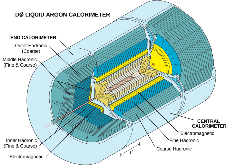
Figure 3.9: Cutaway view of the DØ calorimeter.
