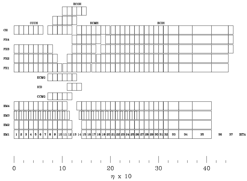
Figure 3.12: Calorimeter channel configuration in terms of depth and \eta .
