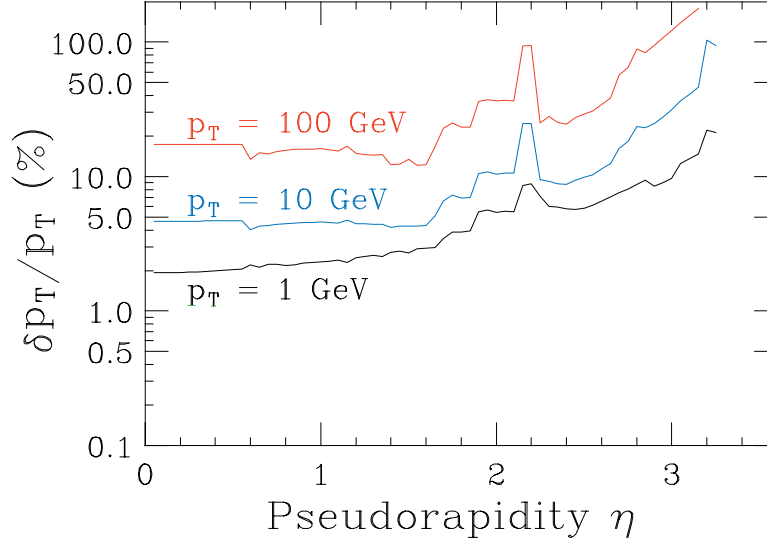
Figure 3.5: Simulation results for the momentum resolution with the Fiber Tracker as a function of pseudorapidity ( \eta ) for three different p_T values.
