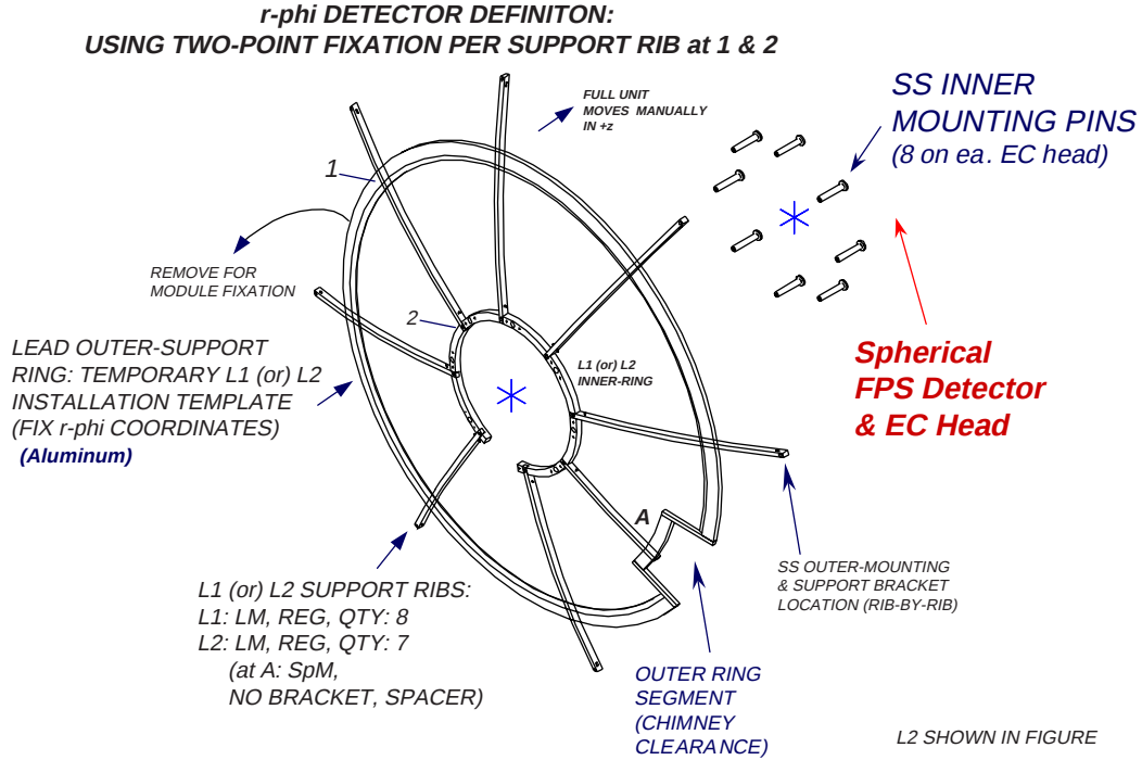
Figure 8.4: Lead layer's precision outer support-ring provides a convenient technique to establish the detector's r - \phi coordinates on the cryostat head, prior to welding and module insertion.
