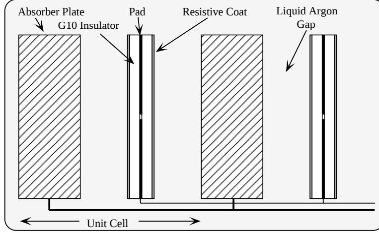
Figure 3.10: Schematic view of a representative calorimeter unit cell. The gap structure, grounded absorber plates, and signal boards are shown.
