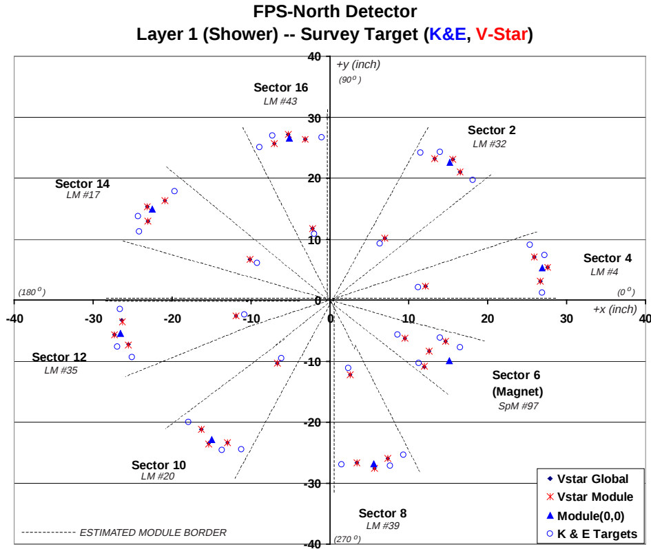
Figure 8.7: Graphical representation of survey target location for the eight modules installed in Layer 1 of FPS-North on the cryostat head. Shown are the actual V-star measurements (asterisk) extrapolated with the mapped K&E (open circle). As described in the text, the location of any V-star target is measured with respect to an arbitrarily chosen K&E (closed triangle), which is taken as the origin (0,0) for the module.
