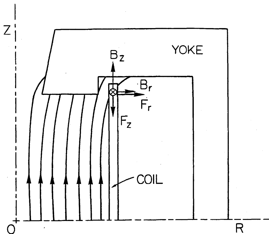
Fig. D(1). Simplified iron geometry - one quadrant
