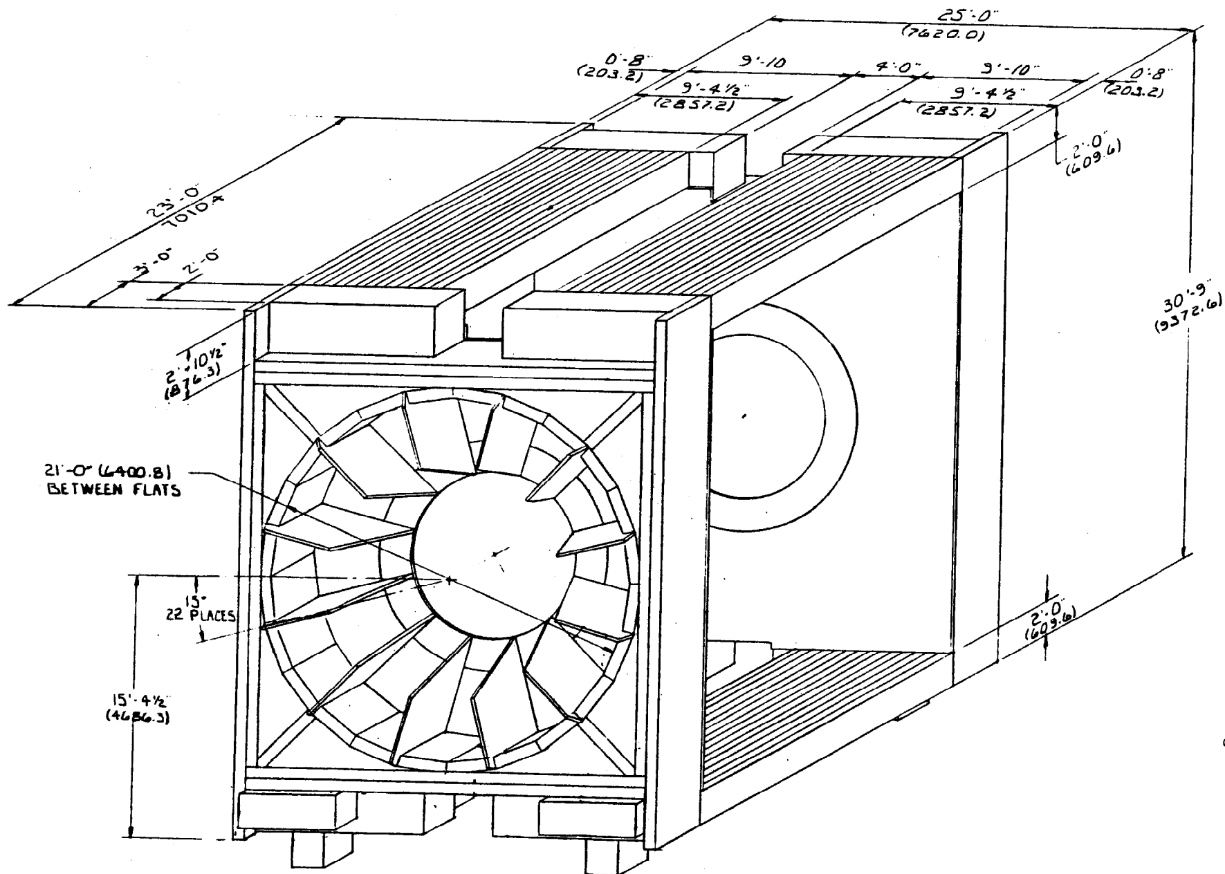
Fig. II(1). Isometric view of bare yoke
