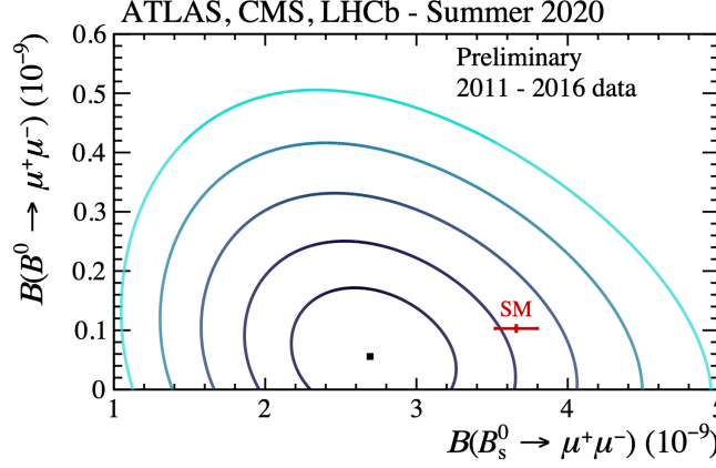
Figure 2.6: Average of the branching fractions of the B^0 \rightarrow \mu^+ \mu^- and B_s^0 \rightarrow \mu^+ \mu^- decays measured by the LHCb, CMS and ATLAS experiments. The contours correspond to different likelihood levels. From darkest to lightest shade, the values of -2\Delta\ln\mathcal{L} of 2.3, 6.2, 11.8, 19.2 and 30.2 are drawn. The SM prediction is represented by the red point [67].
