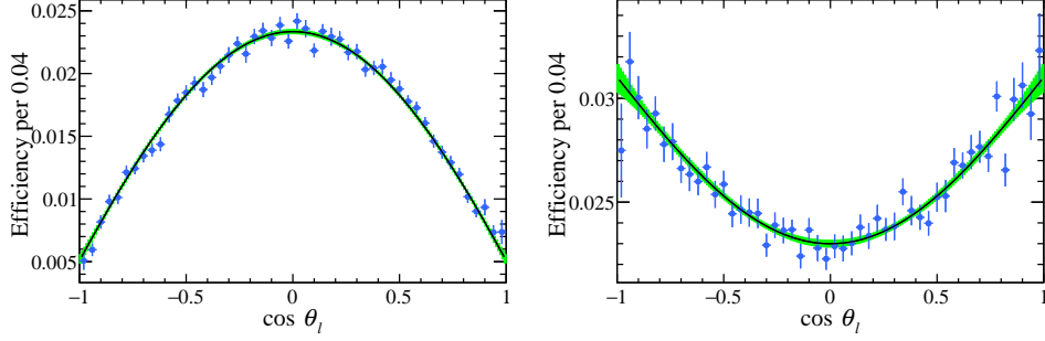
Figure 4.11: Efficiency averaged over the different data-taking periods for the B^+ \rightarrow \pi^+ \mu^+ \mu^- (left) for 1.1–6.0 GeV/ c^4 and (right) 15.0–22.0 GeV/ c^4 . The model is described by the sum of Legendre polynomials up-to and including order four.
