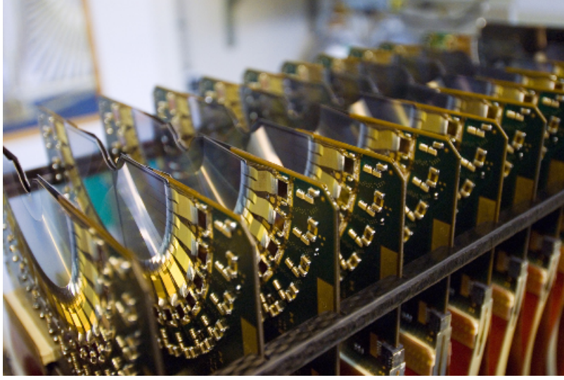
Figure 3.8: Close-up photograph of the VELO halves [114].
