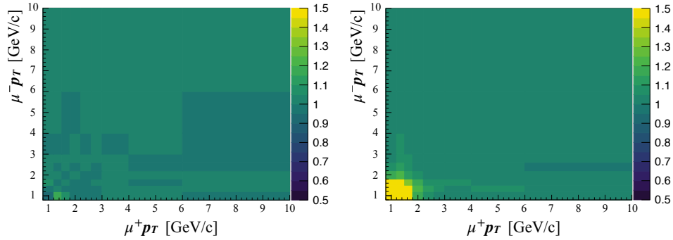
Figure 4.6: Ratio between L0Muon efficiency in data and simulation obtained with the TIS TOS method for (left) 2012 and (right) 2016 data with magnet polarity Up.
