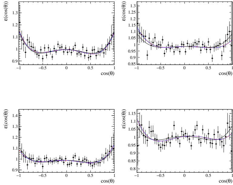
Figure A.1: Efficiency distribution for the B^+ \rightarrow J/\psi(\mu^+\mu^-)K^+ samples fitted with an ordinary polynomial (blue), a sum of Legendre polynomials (dotted red) and a symmetric sum of Legendre polynomials (black). From left to right: down and up magnet polarities, from top to bottom, 2011 and 2012 data-taking years. .
