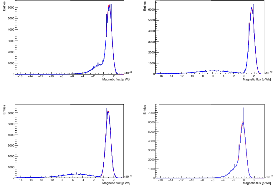
Figure 5.37: Magnetic flux measured by the oscilloscope of signal from four vertically adjacent MCP-PMT pixels, fit with the function described in equation 5.18. Each plot presents the pedestal peak at values \sim 2 pWb, which is followed but the photoelectron peaks as the flux decreases. Due to a binning effect, the oscilloscope introduces artefacts periodically in the datasets. To first approximation these do not affect the fit.
