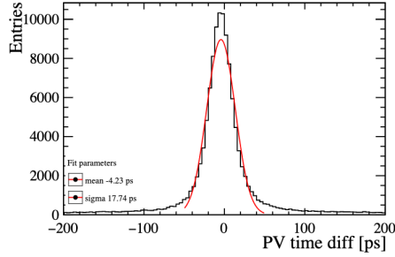
Figure 5.19: Plot of the PV t_0 resolution from reconstruction for a large sample of simulated b\bar{b} events using the reconstruction algorithm described in section 5.6.1. The distribution is fitted with a Gaussian function to extract the time resolution.
