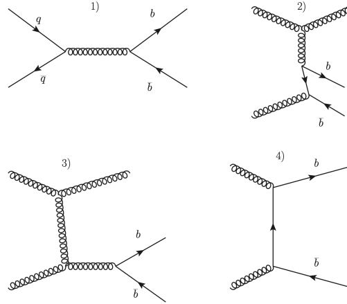
Figure 3.4: Allowed b\bar{b} production mechanisms. Channel 1 corresponds to quark-antiquark annihilation, channel 2 is flavour excitation, Feynman diagram 3 illustrates gluon splitting, and mechanism 4 is gluon-gluon fusion. Figure taken from [108].
