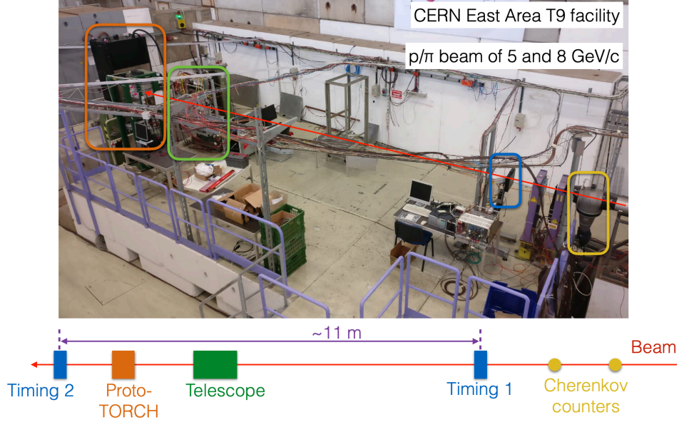
Figure 5.25: Photo of the latest Proto-TORCH test beam set up. Proto-torch is highlighted by the orange box, the Cherenkov counters by the yellow box. Only one of the timing stations is in the shot, highlighted by the blue box. The second timing station is off camera to the left.
