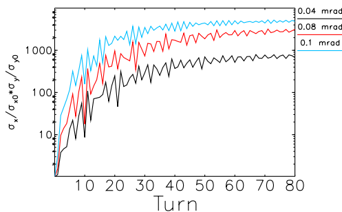
Figure 5: Normalized transverse beam size as a function of the number of turns for different values of kicks in both planes (1000 particles, \varepsilon_x = 17.4 pm rad, \varepsilon_y = 4 pm rad).
