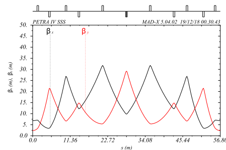
Figure 1: Beta functions of the short straight section SSS.
