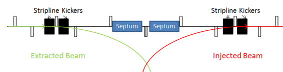
Figure 2: Schematic of the PETRA IV injection and extraction.
