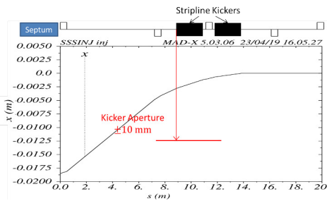
Figure 3: The horizontal trajectory of the injected beam.
