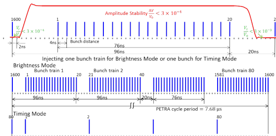
Figure 4: Injection fill pattern scheme for PETRA IV on-axis injection.
