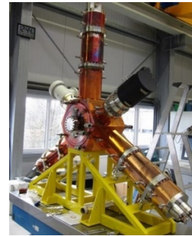
Figure 1: EU HOM-damped cavity.
