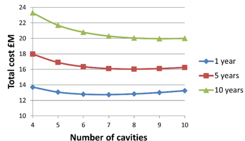
Figure 3: Cost of multiple HOM-damped cavities.
