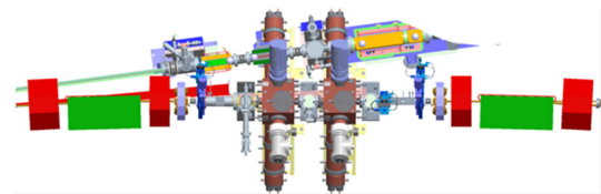
Figure 2: Two cavities in a mid-section straight.
