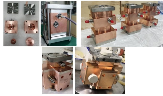
Figure 2: The picture of these three type cavities. Top-left: CBPM-100 ns; Top-right: CBPM-200 ns; Bottom: CBPM-300 ns.
