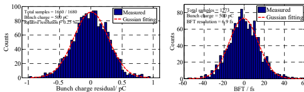
Figure 6: (left) Bunch charge resolution and (right) beam arrival time resolution based on the two adjacent reference cavities.
