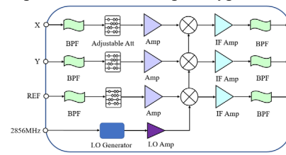
Figure 3: Schematic diagram of the RF front-end.
