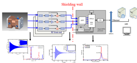
Figure 1: System architecture of the CBPM system.
