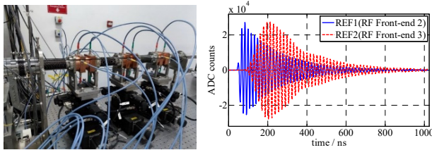
Figure 5: (left) The BPM test array installed at the SXFEL; (right) Waveform of the two adjacent reference cavities.
