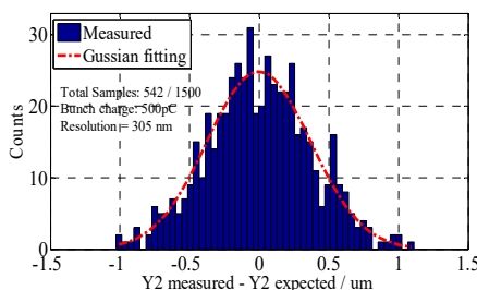
Figure 7: Histogram of the differential of the Y measured and the Y expected.
