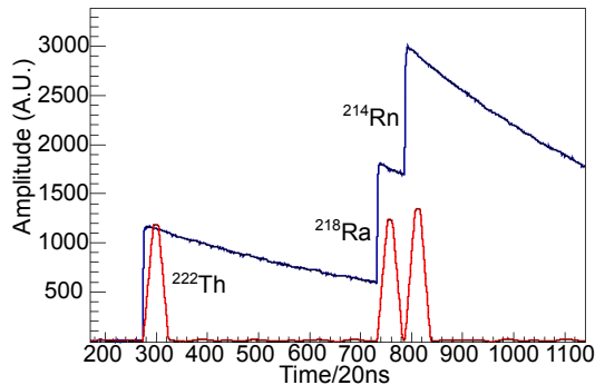
Fig. 2. (Colour on-line) An example trace (black/blue) of the triple pile-up signal ^{222}\text{Th} (1.56 ms) \rightarrow ^{218}\text{Ra} (9.17 \mu\text{s} ) \rightarrow ^{214}\text{Rn} (1.09 \mu\text{s} ) with the energy resolved using the trapezoidal filter shown in grey/red, and the times given as the measured values in the shown trace.
