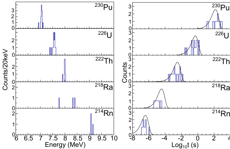
Fig. 4. Left: The \alpha -decay energies of the decay chain originating from ^{230}\text{Pu} measured at SHIP. Right: \alpha -decay half-life distributions of each member of the chain. The solid curves indicate the calculated time distributions for which the mean values are taken from literature.
