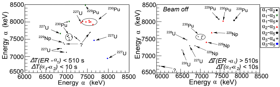
Fig. 3. Left: \alpha - \alpha matrix in a time range 510 s following an EVR implantation and a time difference \Delta T(\alpha_1-\alpha_2) less than 10 s apart (beam pause and beam on). The measured decays depending upon the position in the chain they belong to ( e.g. \alpha_2-\alpha_3 ) is indicated with different symbols given in the legend, and the chain they originate from is labelled. Right: The same as left but more than 510 s following implantation and in the beam pause period only showing longer lived decays.
