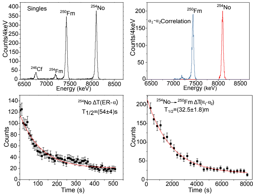
Fig. 1. (Colour on-line) Top left: ^{254}\text{No} \alpha -decay spectrum measured at SHIP in 2016 with the DSSD. Bottom left: ^{254}\text{No} half-life measured between EVR implantation and \alpha decay within 10 \times T_{1/2} of the literature value of T_{1/2}^{\text{lit}} = (51.2 \pm 0.4) \text{ s} . Right top: \alpha - \alpha spectrum of ^{250}\text{Fm} correlated to decays of ^{254}\text{No} (red) within 6 \times T_{1/2} of ^{250}\text{Fm} . Right bottom: \alpha -decay half-life of ^{250}\text{Fm} . Events were searched for in the same pixel in the beam off period.
