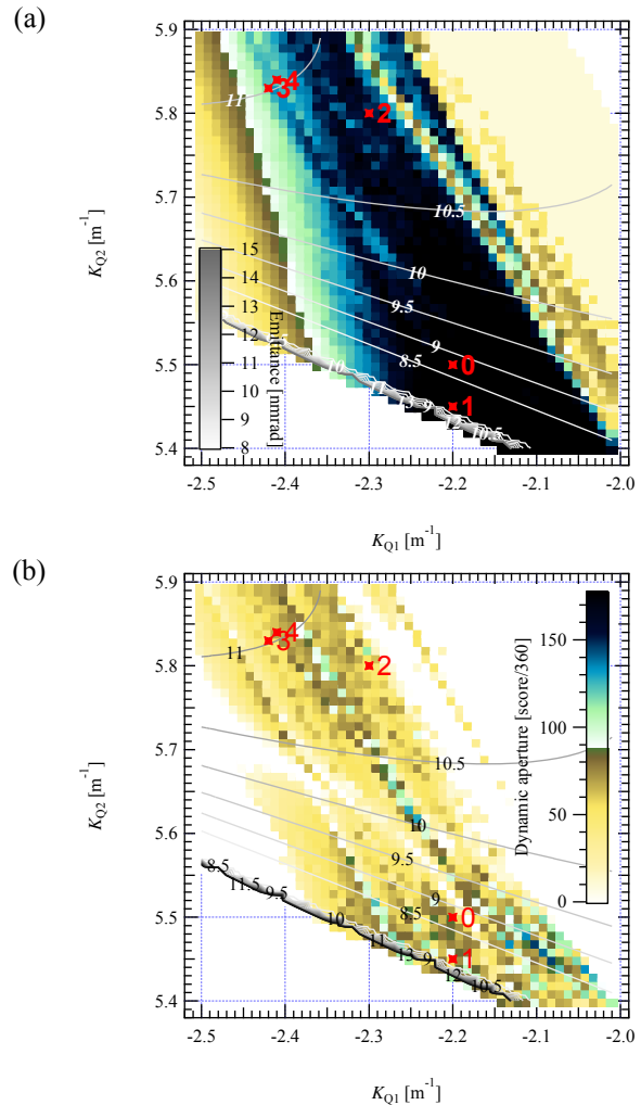
Figure 5: Result of K-survey. (a): dynamic aperture at the centre of long straight section without alignment errors, (b): with alignment errors. Contour lines in each graph show natural emittance.
