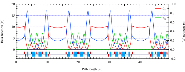
Figure 6: Beta functions and dispersion function in 1/3 turns of ring at operating point #1.
