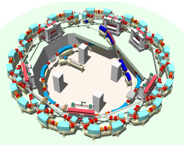
Figure 7: The bird eye view of the (11, 3)-AMATELAS with multi-bend lattice for HiSOR-II.
