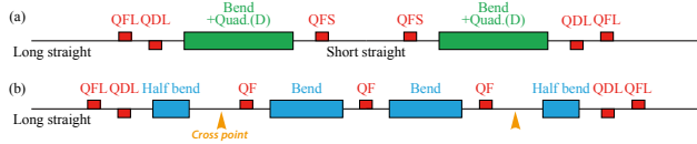
Figure 3: Multi-bend type cells compared with double-bend lattice. (a) is original double-bend lattice. (b) shows multi-bend lattice for (11,3)-AMATELAS.
