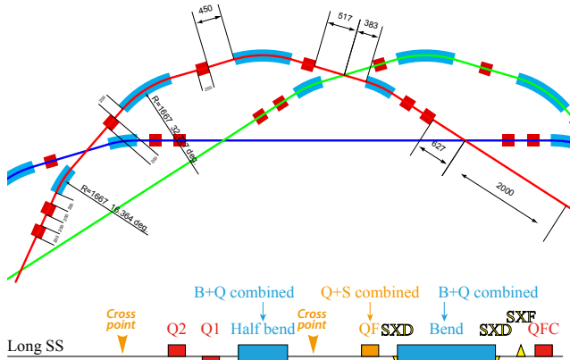
Figure 4: Geometry of unit cell of HiSOR-II and lattice of half of unit cell.
