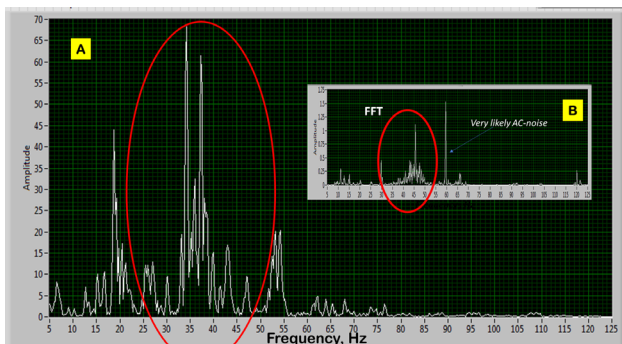
Figure 11: Two spectrums of the cavity vibrations. (A) Cavity response on the external (to Top Plate) hits. (B) Spectrum of the cavity microphonics.
