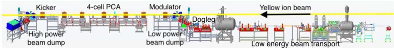
Figure 4: PCA-based CeC system installed at BNL RHIC. The electron beam is generated in a 1.25 MV superconducting radio frequency (SRF) photo-electron gun, accelerated to 14.56 MeV, and merged to co-propagate with the 26.5 GeV/u ion beam circulating in RHIC's yellow ring.
