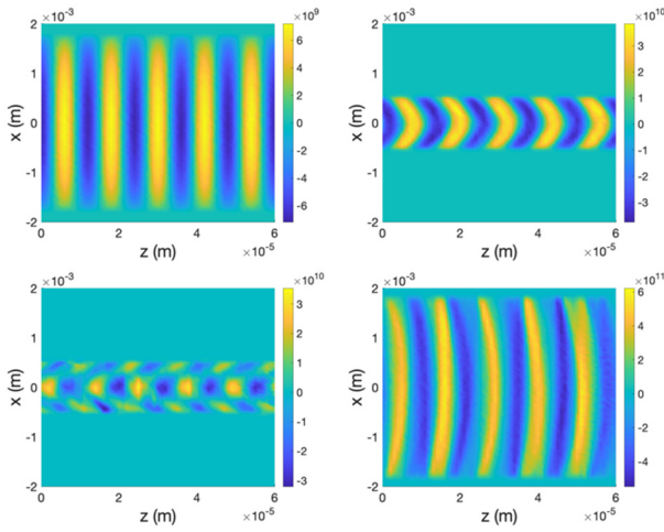
Figure 3: 2D plot of density modulation at 25 THz at the entrance of PCA (top left), slightly before the waist of second cell (top right), slightly after the waist of second cell (bottom left) and at the exit of PCA (bottom right).
