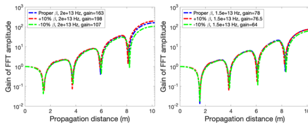
Figure 8: Dependence of PCA amplification on initial \beta function for electron beam peak current 75A and normalized KV emittance 7 mm mrad (left) and 10 mm mrad (right).
