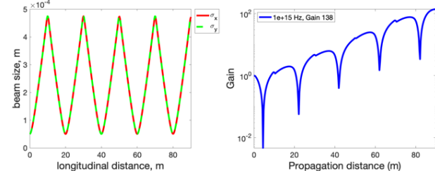
Figure 9: Evolution of transverse RMS beam size (left) and amplification of initial density modulation at 1 PHz (right) in the PCA designed for future EIC.
