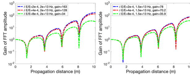
Figure 7: Dependence of PCA amplification on energy spread for electron beam peak current 75A and normalized KV emittance 7 mm mrad (left) and 10 mm mrad (right).
