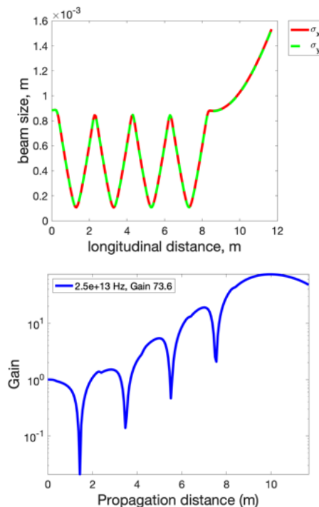
Figure 2: Evolution of transverse RMS beam size (top) and growth of initial density modulation at 25 THz (bottom) in a 4-cell periodic PCA followed by a drift.
