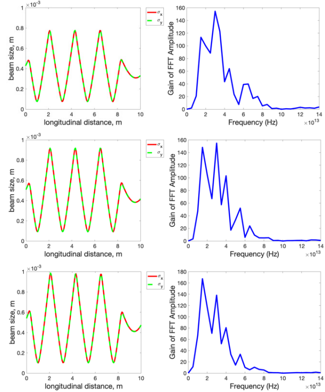
Figure 5: Evolution of transverse RMS beam size (left) and amplification spectrum (right) in a 4-cell realistic PCA for electron beam peak current 50A (top), 75A (middle) and 100A (bottom).
