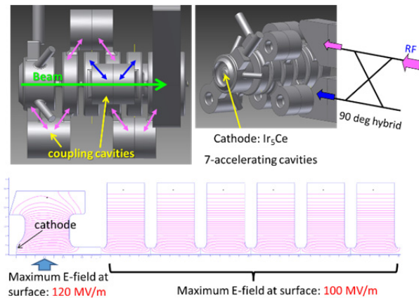
Figure 2: Quasi travelling-wave side-couple RF gun.
