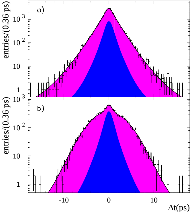
FIG. 10: Same as Fig. 9 with logarithmic scale.
