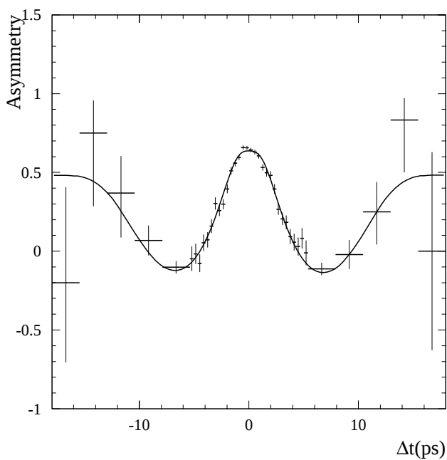
FIG. 12: Asymmetry between unmixed and mixed events as a function of \Delta t , for events in the background \mathcal{M}_\nu^2 region. Points with error bars represent the data, and the curve is a projection of the fit result.
