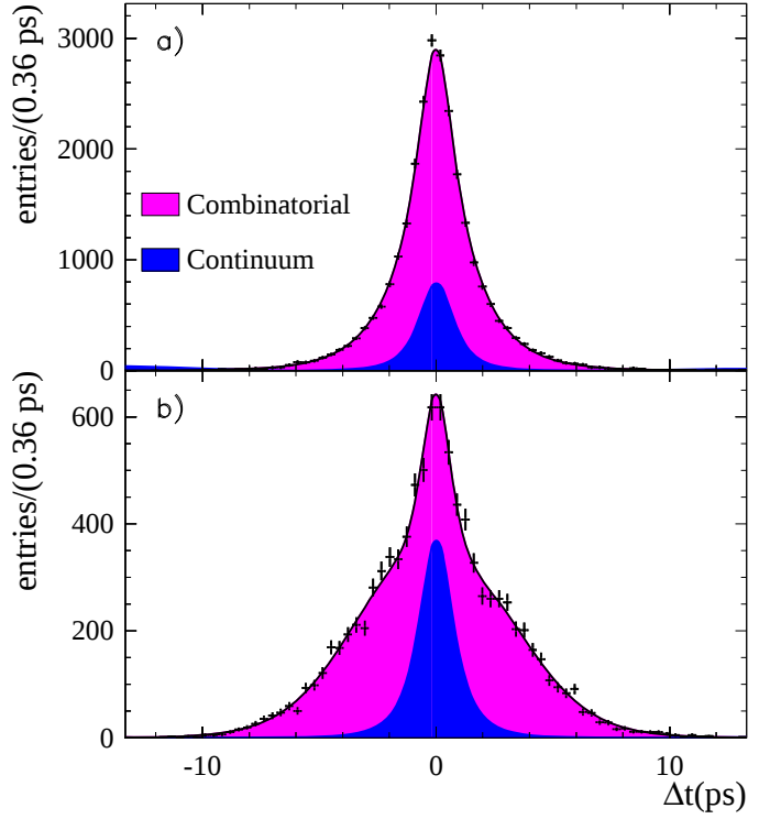
FIG. 9: Distribution of \Delta t for unmixed (a) and mixed (b) events in the background \mathcal{M}_v^2 region. The points show the data, the curve is the projection of the fit result, and the shaded areas are the contributions from continuum and B\bar{B} combinatorial background.
