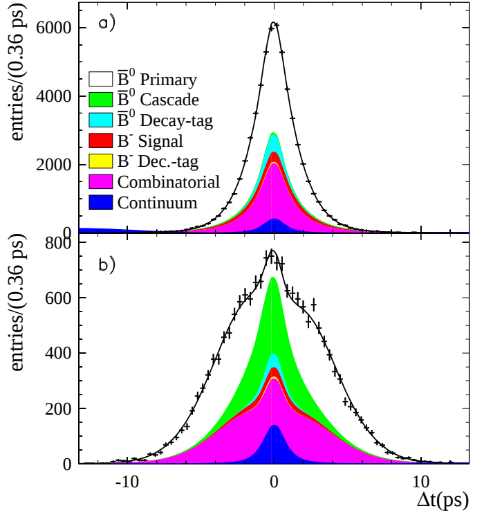
FIG. 7: Distribution of \Delta t for unmixed (a) and mixed (b) events in the signal \mathcal{M}_\nu^2 region. The points show the data, the curve is the projection of the fit result, and the shaded areas from bottom to top are the contributions from continuum background, B \bar{B} combinatorial background, peaking B^- background with decay-side tag, peaking B^- background with primary tag, signal with decay-side tag, signal with cascade tag, and signal with primary tag.
