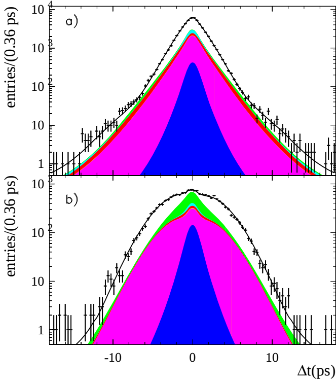
FIG. 8: Same as Fig. 7 with logarithmic scale.
