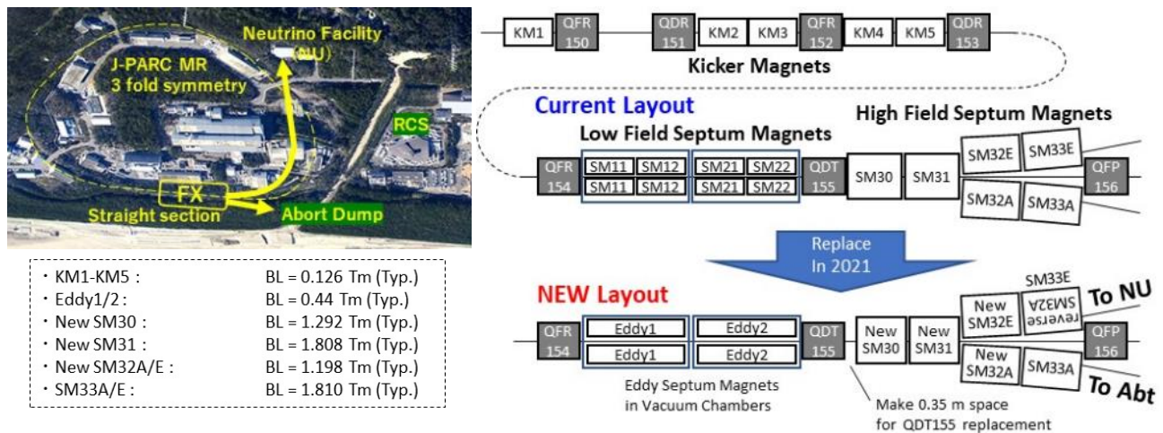
Figure 1: The outline of layout and replacement.
