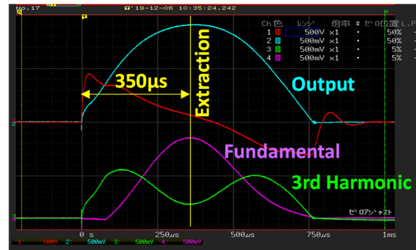
Figure 5: Pulse operation of the eddy SM.
