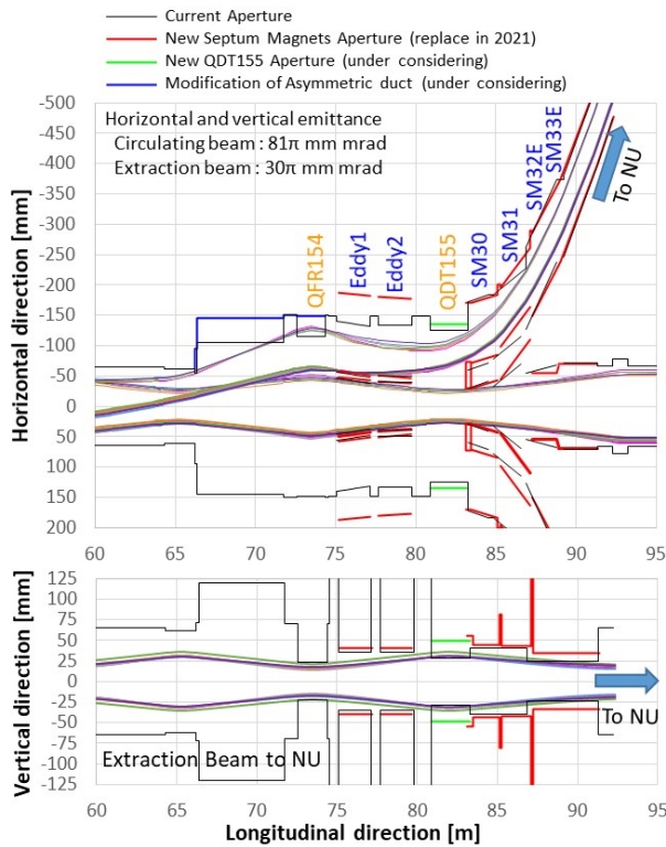
Figure 3: New Aperture plans and beam envelopes.
