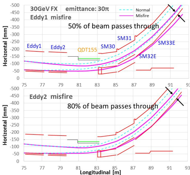
Figure 4: Simulation of the eddy SM failure.
