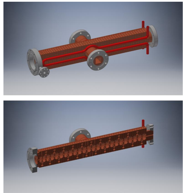
Figure 1: X-band RF cavity.
