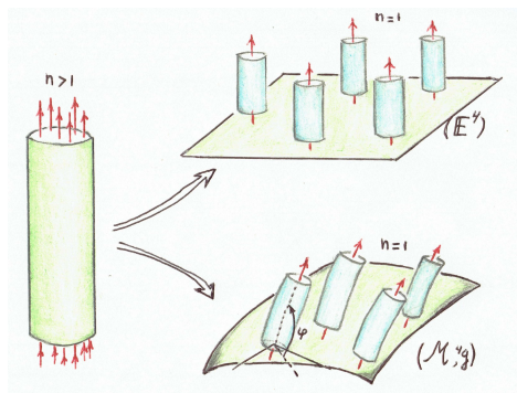
Fig. 1. Excitation and decay of a high multiplicity vortex into correlated vortices of unit flux n = 1 . Top: the Abrikosov lattice in Euclidean space. Bottom: correlated vortices with preferred azimuthal angle \varphi in curved spacetime after the symmetry breaking.
