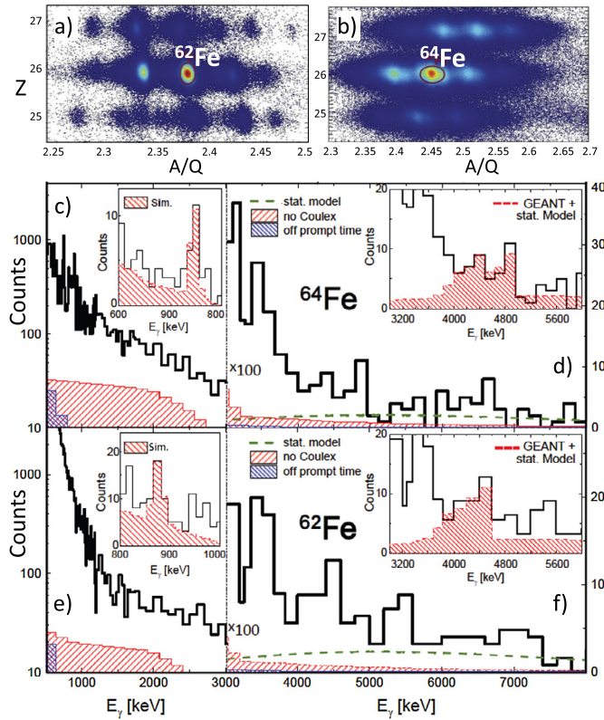
Fig. 1. Top panels a) and b) show the particle identification plots obtained when the fragment separator was set for the optimal transmission of the ^{62}\text{Fe} (left) and ^{64}\text{Fe} (right) secondary beams. The circles indicate the isotopes of interest. Panels c) to f) show the low energy part (left) and high energy part (right) of the measured \gamma spectra. The shaded areas in these figures display the spectral shapes obtained with gates corresponding to events outside the Coulomb excitation conditions (red area) or out of the prompt time of flight peak (blue area). The dotted lines (green) in panels d) and f) give the calculated statistical contribution to the spectra. The insets in the panels c) and e) display the known transitions from the first 2^+ states, as obtained with full tracking together with the Monte Carlo simulations of the expected peak. In the insets of panels d) and f) the counts forming peak structures at around 4.5 MeV are compared with simulations taking into account the detection conditions. An increase of the bin size with energy has been chosen to take account for the efficiency loss in the detection of high energy \gamma rays.
