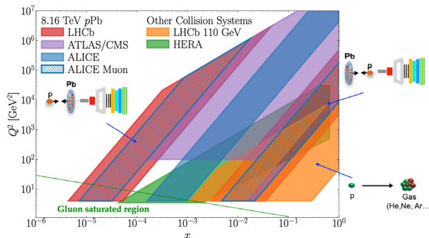
Figure 1. The LHCb acceptance in the Q^2 / Bjorken- x plane compared to other experiments.
