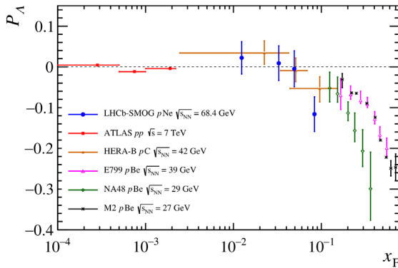
Figure 3. Comparison of the magnitude of the \Lambda hyperon polarization as a function of x_F obtained in the experiments performed up to the time of writing.
