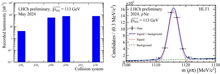
Figure 4. The left plot shows the integrated luminosity recorded during May 2024, corresponding to around two hours of injections per gas. The right plot shows the invariant mass distribution for \Lambda \rightarrow p\pi^- decay candidates.
