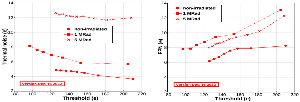
Figure 4. Thermal noise (left) and FPN (right) as a function of the pixel discriminator threshold and of the integrated ionising radiation dose, for the AC-pixel with “p-stop” epitaxial layer, operated with -3 V back-bias and 10 V top-bias voltages.
