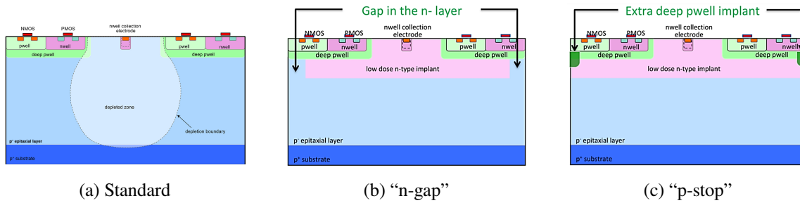
Figure 3. Three different sensing node, viz. epitaxy doping profile, options used in MIMOSIS-1. Reprinted from [6], Copyright 2017, with permission from Elsevier.
