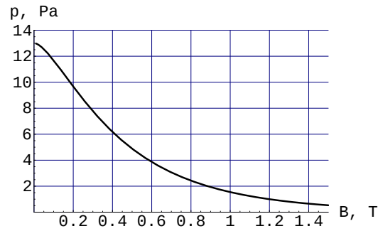
Fig. 4. Casimir pressure for scalar field as a function of magnetic field B , corresponding to distance a = 100 nm. The diagram is made in SI units for massless field.
