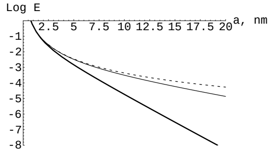
Fig. 2. Casimir energy for scalar field as a function of distance a , for massless field m = 0 and L = 1 m. Bold curve corresponds to magnetic field B = 100 T whereas the thin one corresponds to B = 10 T. The dashed curve corresponds to function -\pi^2 \hbar c a^{-3} / 720 (standard function of distance a for B = 0 ). Values of energy are shown in logarithmic scale.
