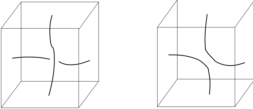
Figure 10.1: A toroidal topology can be represented as a cube, where opposite faces are identified. The left panel shows two closed strings winding around different compact directions. These strings will generically intersect each other if they are propagating in 3-dimensional space. After the intersection, the strings regroup as displayed in the right panel. Effectively, this process corresponds to an unwinding from the compact direction.
