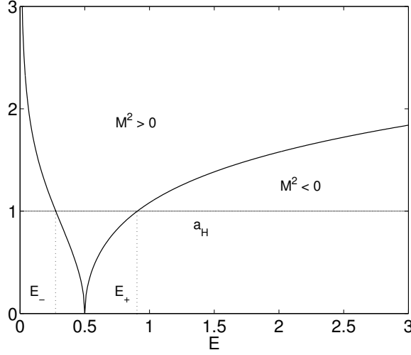
Figure 5.5: The curve represents a_c , the zero of M^2(\tau) , as a function of the energy E as given in Eq. 5.65. Below the curve the effective mass squared is negative, above it is positive. For E < E_- and E > E_+ the M^2(\tau) already becomes negative outside the horizon, whereas for energies within the interval E_-, E_+ the M^2(\tau) < 0 region is hidden within the horizon. The parameters chosen are q = 1 , r_H = 1 , and L = 1 .
