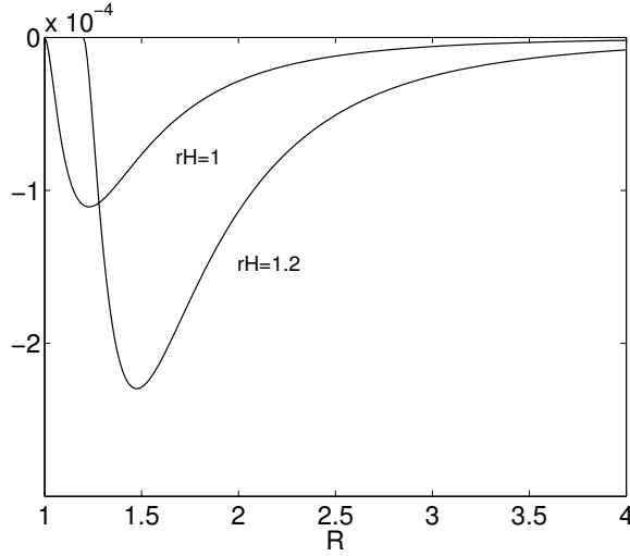
Figure 5.1: V_{\text{eff}}^t(E, q, R) for E = 0, q = 1, L = 4 and different values of r_H . For R \rightarrow \infty the potential goes to zero according to our normalization. When r_H = 0 , the potential is exactly flat.
