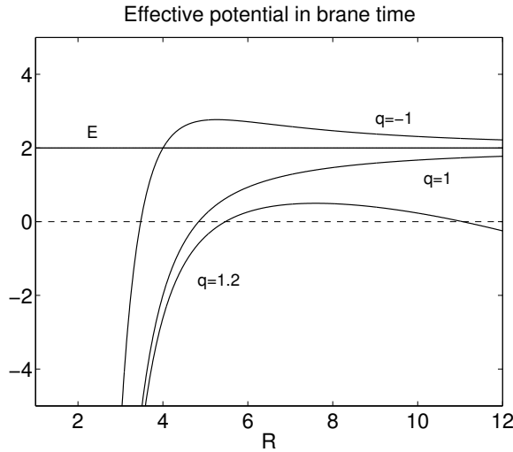
Figure 5.3: V_{\text{eff}}^\tau(E, q, R) for the same parameters as in Fig. 5.2. A BPS brane has zero kinetic energy at infinity corresponding to a vanishing cosmological constant on the brane. Otherwise, the cosmological constant is \propto q^2 - 1 . A BPS anti-brane is allowed to move only in a restricted range of R : after having reached a maximal scale factor, the universe starts contracting. Any inwardly moving brane falls into the black-hole in a finite \tau .
