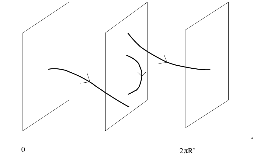
Figure 3.1: The horizontal axis corresponds to the T-dual coordinate x'^d . An open string with winding number zero starts and ends on the same Dp-brane, whereas an open string with single winding can be represented by identifying the hyperplanes on the left and on the right. Note that those are not Dp-branes; they just symbolize the periodic identification.
