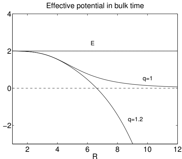
Figure 5.2: V_{\text{eff}}^t(E, q, R) for E = 2 , r_H = 1 , L = 4 . For a BPS-brane ( q = 1 ), V_{\text{eff}}^t \rightarrow 0 as R \rightarrow \infty according to our normalization. This should be contrasted with a non BPS brane e.g. with q = 1.2 . Note that V_{\text{eff}}^t(E, q, R = r_H) = E . Any inwardly moving (contracting) brane takes an infinite amount of t -time to reach the horizon.
