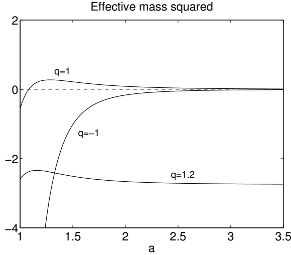
Figure 5.4: The dimensionless quantity M^2 L^2 (on the vertical axis) is plotted as a function of a for E = 1, L = 1, r_H = 1 . Here, the effective mass squared is positive in a certain range only for the BPS-brane. Note that the negative M^2 L^2 region is not hidden behind the horizon.
