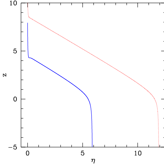
Figure 7.2: The time evolution of the dimensionless Hubble parameter z for the two trajectories shown in Fig. 1.
