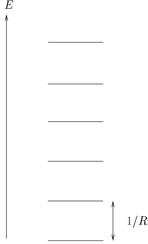
Figure 2.1: Infinite tower of Kaluza-Klein mass states.
