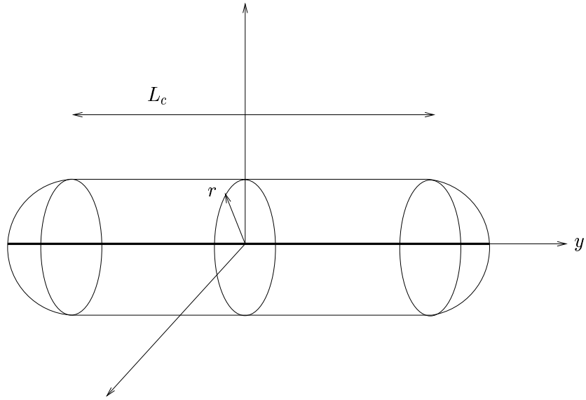
Figure 2.2: A uniform mass density (represented by the solid line) along the extra-dimension y is enclosed by a cylinder of length L_c with two hemispheres as endcaps. Here, r is a distance ‘along’ our 3-dimensional universe.
