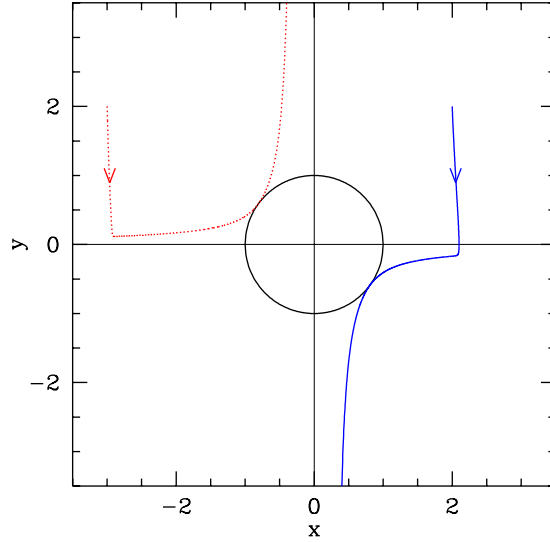
Figure 7.1: Two trajectories in the phase space (x, y) which represent typical solutions of the system (7.40)-(7.41) for K = 1 . The trajectory on the left (dotted, red), starting with an initial condition x_{\text{in}} = -3, y_{\text{in}} = 2 , winds towards the circle x^2 + y^2 = \sqrt{K} , which corresponds to the condition z = H = 0 . After reaching the circle, the solution moves away showing that it is not an attractor. The trajectory on the right (solid) with initial conditions x_{\text{in}} = 2, y_{\text{in}} = 2 shows a similar behavior. It takes much longer to pass the region around the kinks than to trace out the remaining parts of the trajectories.
