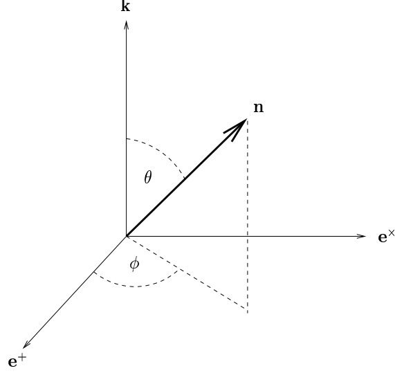
Figure 8.1: The direction of observation, \mathbf{n} , and the set of orthogonal basis vectors (\mathbf{k}, \mathbf{e}^+, \mathbf{e}^\times) over which the amplitudes \hat{v}_i(\eta, \mathbf{k}) and \hat{\sigma}'_i(\eta, \mathbf{k}) are decomposed.
