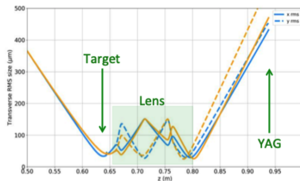
Figure 3: Transverse beam spot size (solid- x, dashed -y) for BNL UED transport with target and quintuplet lens identified in graph. The detector is a YAG scintillator. Blue lines are ideal, and yellow lines include space charge effects.
