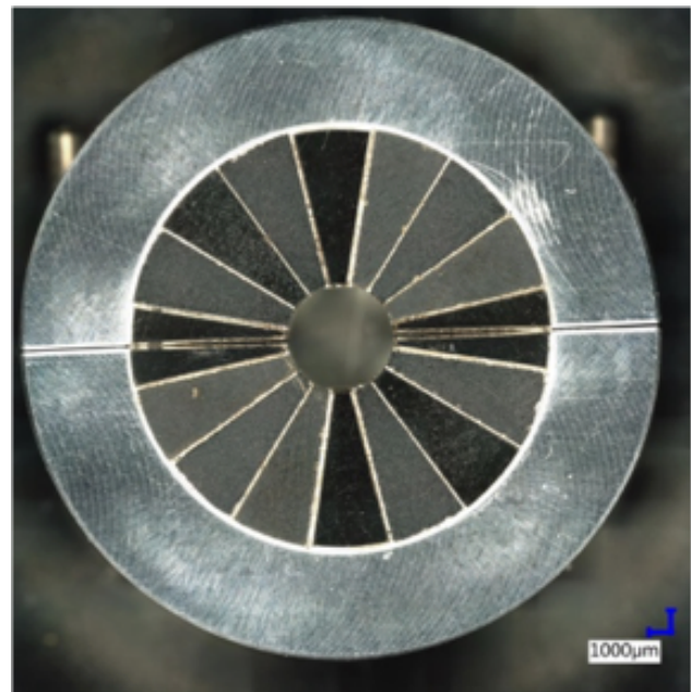
Figure 6: High resolution photograph of hybrid-PMQ with steel wedges for split design. Aperture is 4 mm.
