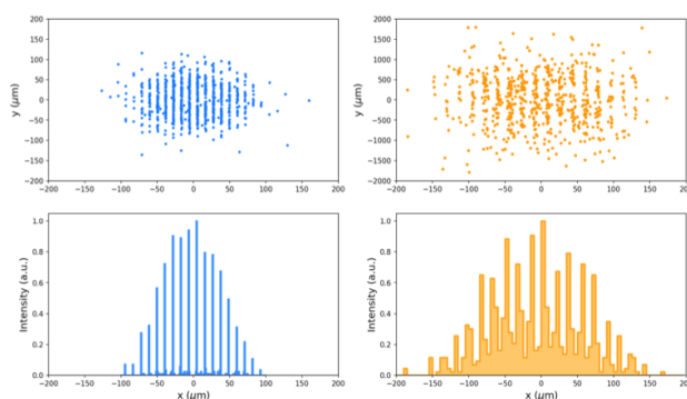
Figure 4: Top row: Simulation of 1-D imaging target with 1\text{ }\mu\text{m} slitted array at interaction point (left column), and imaged distribution at screen (right column). Bottom row: histograms of respective beam distributions.
