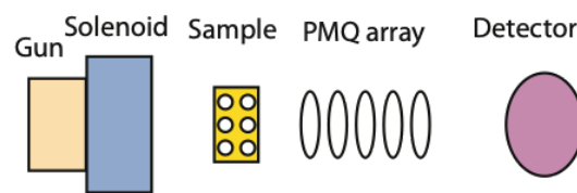
Figure 1: Sketch of experimental configuration to test characteristics of quintuplet lens within existing beamline layout.
