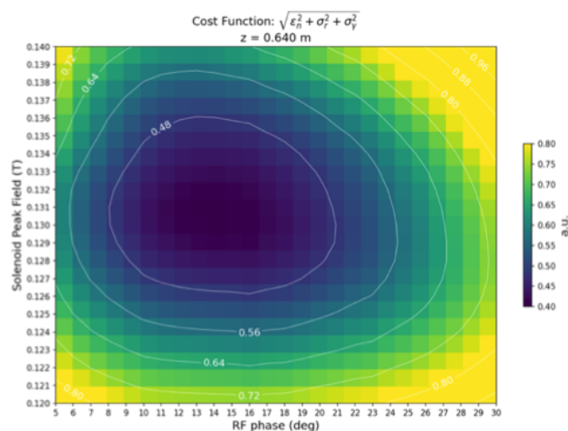
Figure 2: Simulation of cost function to optimize beam emittance and energy spread at interaction point using BNL UED parameters.
