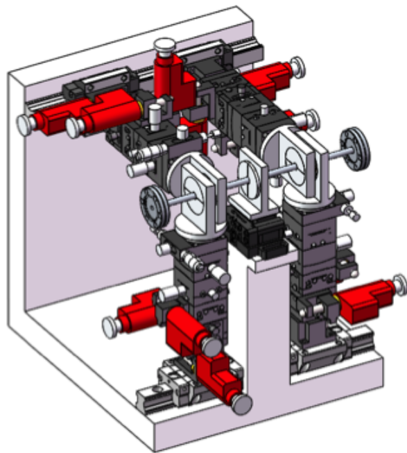
Figure 5: Model of complete assembly using multiple rotation and translation stages to accommodate multiple degrees of freedom for PMQ quintuplet.
