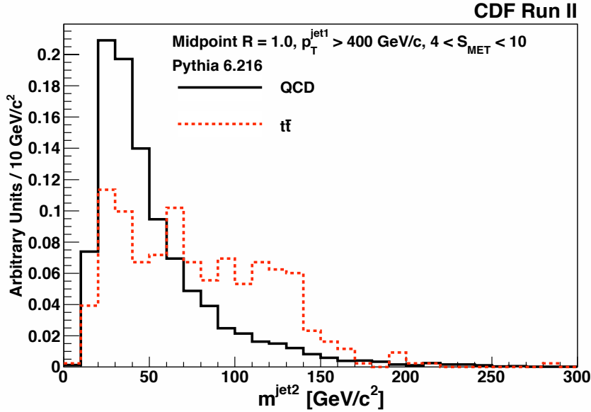
Figure 4: The m^{\text{jet}2} distribution for t\bar{t} and QCD MC events when we require that the event have a leading jet with p_T > 400 GeV/c 2 and |\eta| < 0.7 using R = 1.0 Midpoint cones and S_{MET} \in (4, 10) .
