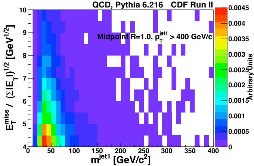
Figure 6: The S_{MET} versus m^{jet1} distribution for QCD MC events with at least one jet with p_T > 400 GeV/ c^2 and |\eta| < 0.7 using R = 1.0 Midpoint cones, where we have required S_{MET} \in (4, 10) .
