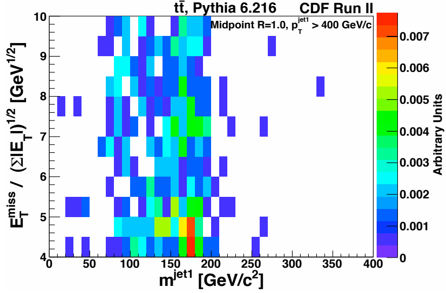
Figure 5: The S_{MET} versus m^{jet1} distribution for t\bar{t} MC events with at least one jet with p_T > 400 GeV/ c^2 and |\eta| < 0.7 using R = 1.0 Midpoint cones, where we have required S_{MET} \in (4, 10) .
