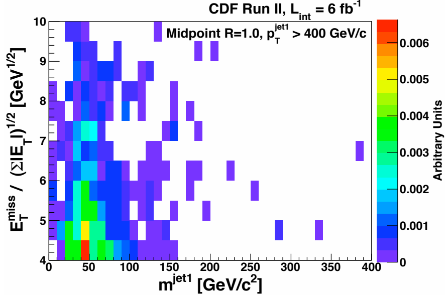
Figure 7: The S_{MET} versus m^{\text{jet1}} distribution for all data events with at least one jet with p_T > 400 \text{ GeV}/c^2 and |\eta| < 0.7 using R = 1.0 Midpoint cones, where we have required S_{MET} \in (4, 10) .
