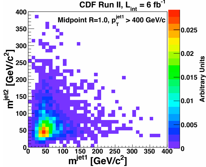
Figure 3: The m^{jet2} versus m^{jet1} distribution for all data events with at least one jet with p_T > 400 GeV/c 2 and |\eta| < 0.7 using R = 1.0 Midpoint cones. The MI corrections have been performed and all events are required to have S_{MET} < 4 .
