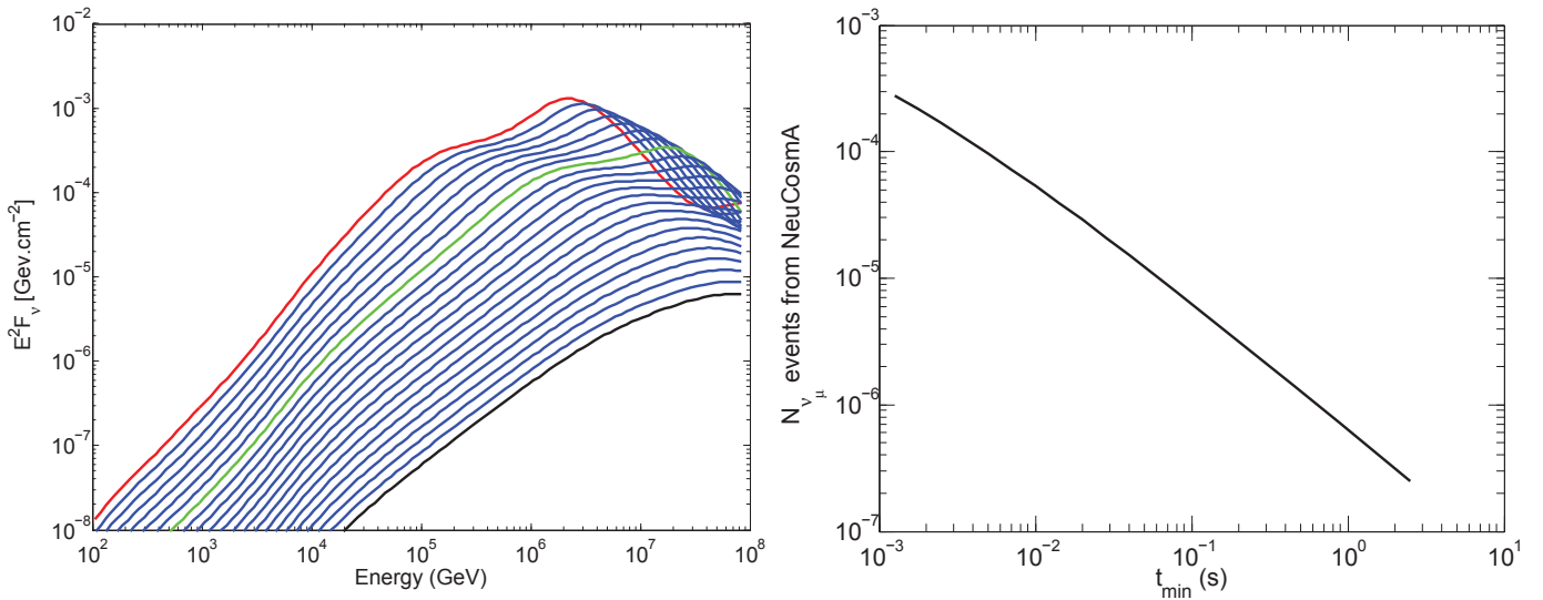
Figure 8.15.: ( Left ) NeuCosmA spectra ( \nu_\mu + \bar{\nu}_\mu ) for a standard GRB with t_{min} \in [0.001(\text{black}) \rightarrow 1(\text{red})] s. Spectra in red, black and green corresponds to the best, the worst and the standard neutrino prediction, respectively. ( Right ) Evolution of the expected number of neutrinos as a function of t_{min} for a standard GRB.
