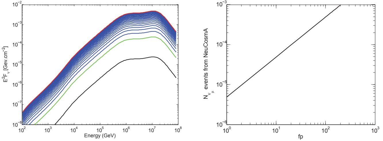
Figure 8.14.: ( Left ) NeuCosmA spectra ( \nu_\mu + \bar{\nu}_\mu ) for a standard GRB with f_p \in [1(\text{black}) \rightarrow 200(\text{red})] . Spectra in red, black and green corresponds to the best, the worst and the standard neutrino prediction, respectively. ( Right ) Evolution of the expected number of neutrinos as a function of f_p for a standard GRB.
