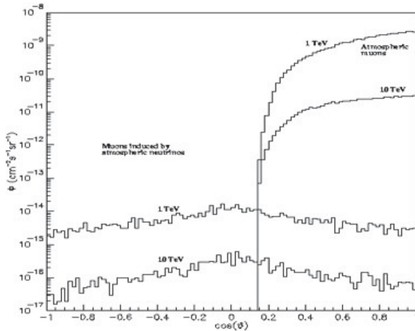
Figure 3.10.: ( Top ) Illustration of the different physical background components (atmospheric neutrinos/muons) in the neutrino astronomy without any selection cuts applied. ( Bottom ) Simulated angular flux of events in the ANTARES detector. Atmospheric muons are only seen above the horizon, whereas muons induced by neutrinos produced in atmospheric interactions are distributed nearly isotropically. The flux is seen to drop precipitously with energy for both distributions. The figure and the caption are extracted from (Hoffman 2009).
