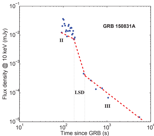
Figure 5.12.: The afterglow x-ray light curve of GRB 150831A detected by the Swift -XRT instrument (blue dots). The late steep decay phase (noted as ”LSD”), with \alpha_{LSDP} = -7.06 , is difficult to interpret as it appears for only 2 GRB x-ray afterglows.
