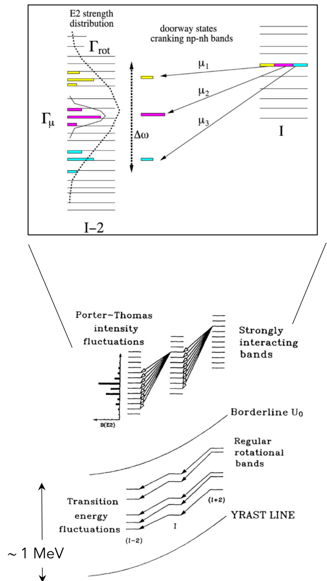
Fig. 13 Bottom: Schematic representation of the \gamma -decay pattern in the excitation energy-angular momentum phase space. The region of discrete, regular rotational bands (ordered motion) and the regime of strongly interacting bands (at the onset of chaos) are indicated. Top: Detailed illustration of the fragmentation of the rotational E2 strength from a state at spin I to a number of final states at spin (I-2) , owing to the complex nature of the nuclear states already at few hundreds keV excitation energy above the yrast line. The FWHM of the distribution at (I-2) is called rotational damping width, \Gamma_{rot} [123]. The \mu_i values are np - np unperturbed “shell model” bands, mixed by the residual interaction over the \Gamma_\mu energy range (i.e., the compound nucleus spreading width) to form a state at spin I . The dispersion \Delta\omega in rotational frequency, from spin I to spin (I-2) originates from the different response to rotation of each unperturbed band. Adapted from [124, 125]
