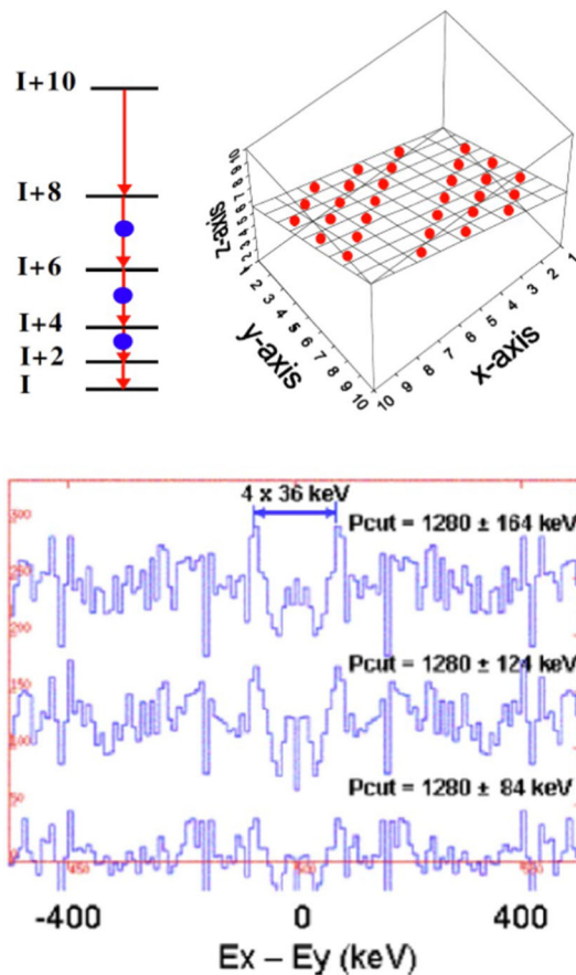
Fig. 12 Top Panel: Schematic representation of the so-called “rotational plane”, obtained from three-dimensional histograms (with the energy correlation condition E_{\gamma_1} + E_{\gamma_2} = 2E_{\gamma_3} \pm \delta ), selecting rotational cascades of at least 3 consecutive transitions. Bottom panel: rotational plane projections (perpendicular to the main diagonal, at the average energy 1280 keV and width \pm 84 , \pm 124 , \pm 164 keV) in ^{128}\text{Xe} , populated by the ^{64}\text{Ni} + ^{64}\text{Ni} \rightarrow ^{128}\text{Ba} fusion evaporation reaction, performed with Euroball at Strasbourg. Ridge structures associated with very large moment of inertia are consistent with hyperdeformed shapes. Figure adapted from Ref. [91], under CC Licence
