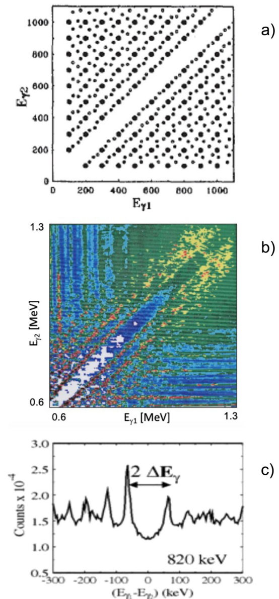
Fig. 15 a Illustration of the emergence of rotational correlations in \gamma – \gamma coincidence matrices from rotating nuclei at high spins. Regular rotational bands (e.g., the yrast and discrete excited bands, see Fig. 13) generate ridge structures running parallel to the E_{\gamma 1} = E_{\gamma 2} diagonal (panel a )), while the fragmented rotational decay from strongly mixed bands, gives rise to a rather uniform distribution filling also the valley region. b \gamma – \gamma spectrum of ^{168}\text{Yb} (0.6–1.3 MeV region, 1 keV/ch), obtained with the Eurogam I array [135]. c projection of the ^{168}\text{Yb} \gamma – \gamma matrix, perpendicular to the E_{\gamma 1} = E_{\gamma 2} diagonal, at the average transition energy 820 \pm 30 keV. The distance between the two most inner ridges depends on the moment of inertia J^{(2)} , being \Delta E_{\gamma} = h^2/2J^{(2)} . For E_{\gamma 1} > E_{\gamma 2} the intensity associated to known discrete rotational bands has been subtracted from the \gamma – \gamma matrix, leading to the asymmetric ridge structure. The remaining ridge intensity corresponds to discrete bands, not yet resolved. Adapted from [116, 118]
