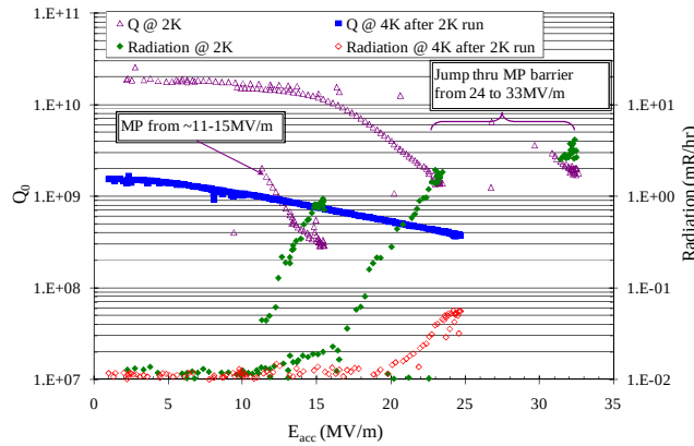
Figure 5: Q_0 vs. E_{acc} from the first cold test of SSR1-02.
