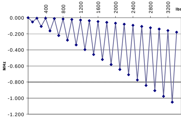
Figure 3: Cycling loads and frequency shifts of the cavity during the operation of inelastic tuning.
