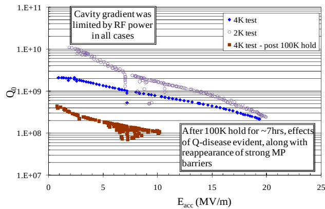
Figure 2: Q_0 vs. E_{acc} at 2.0 K and 4.4 K from the fourth cold test of SSR1-01.
