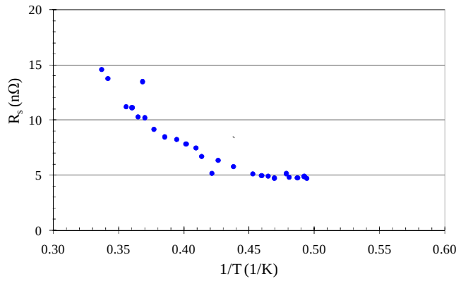
Figure 4: R_s vs. 1/T from the first cold test of SSR1-02.
