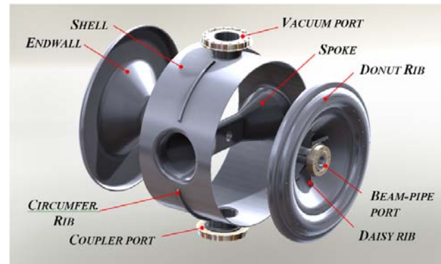
Figure 1: Exploded view of the SSR1 resonator showing the three major sub-assemblies.
