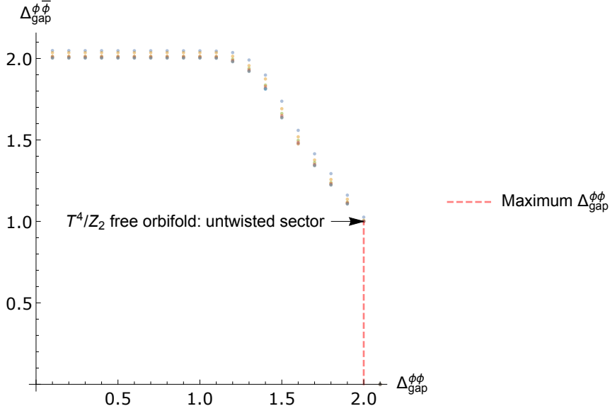
Figure 2.7: The dots indicate upper bounds (\widehat{\Delta}_{gap}^{\phi\phi}, \widehat{\Delta}_{gap}^{\phi\bar{\phi}}) on the gap in the respective OPEs, at derivative orders ranging from 8 to 20. We find that \Delta_{gap}^{\phi\phi} is bounded above by 2, beyond which \Delta_{gap}^{\phi\bar{\phi}} = 0 . The point (2, 1) is realized by an untwisted sector correlator at the T^4/\mathbb{Z}_2 free orbifold point.
