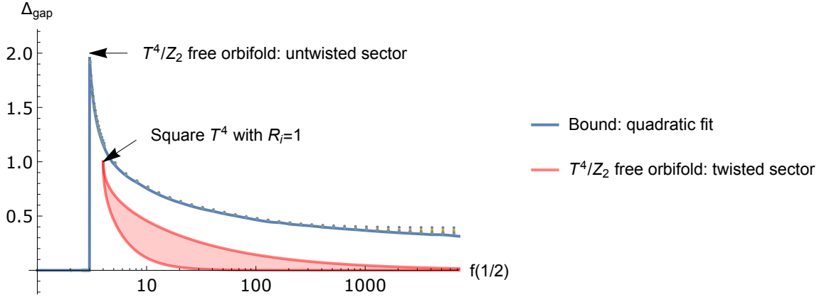
Figure 2.4: The dots indicate the upper bound \widehat{\Delta}_{gap} on the gap versus f(1/2) , the four-point function evaluated at the crossing symmetric point, at derivative orders ranging from 8 to 20. The solid line plots the extrapolation to infinite order using a quadratic fit. The minimal f(1/2) and maximal gap are simultaneously saturated by an untwisted sector correlator at the free orbifold point. The shaded region represents the gap in the OPE of twist fields at a fixed point of T^4/\mathbb{Z}_2 with a rectangular T^4 , where the minimal f(1/2) and maximal gap are achieved by a square T^4 at radii R_i = 1 ( 1/\sqrt{2} times the self-dual radius).
