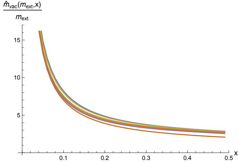
Figure 3.3: The weight \hat{m}_{\overline{\text{vac}}}(m_{\text{ext}}, x) as a function of the cross ratio x for external weights m_{\text{ext}} = \alpha/24 . See (3.26) for a definition. The curves from top to bottom are for \alpha = 1/100, 1/10, 1/2, 1, 2, 12 .
