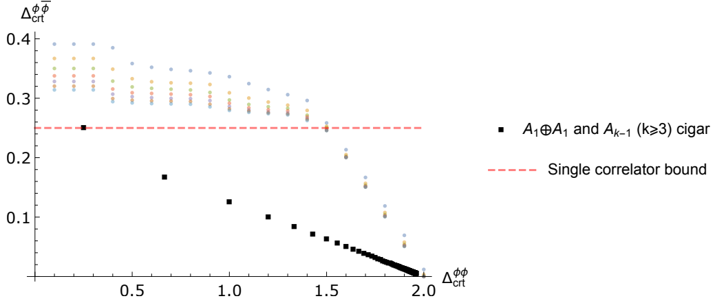
Figure 2.9: The circle dots indicate upper bounds (\widehat{\Delta}_{crt}^{\phi\phi}, \widehat{\Delta}_{crt}^{\phi\bar{\phi}}) on the divergent operator of the lowest scaling dimension in the respective OPEs, at derivative orders ranging from 8 to 20. At infinite order, the bound cannot be worse than the single correlator bound 0.25 indicated by the dashed line. We also find that \Delta_{crt}^{\phi\bar{\phi}} is bounded above by 2, beyond which \Delta_{crt}^{\phi\bar{\phi}} = 0 . The square dots indicate the values for the A_1 \oplus A_1 (at (1/4, 1/4) ) and A_{k-1} ( k \geq 3 ) cigar theories.
