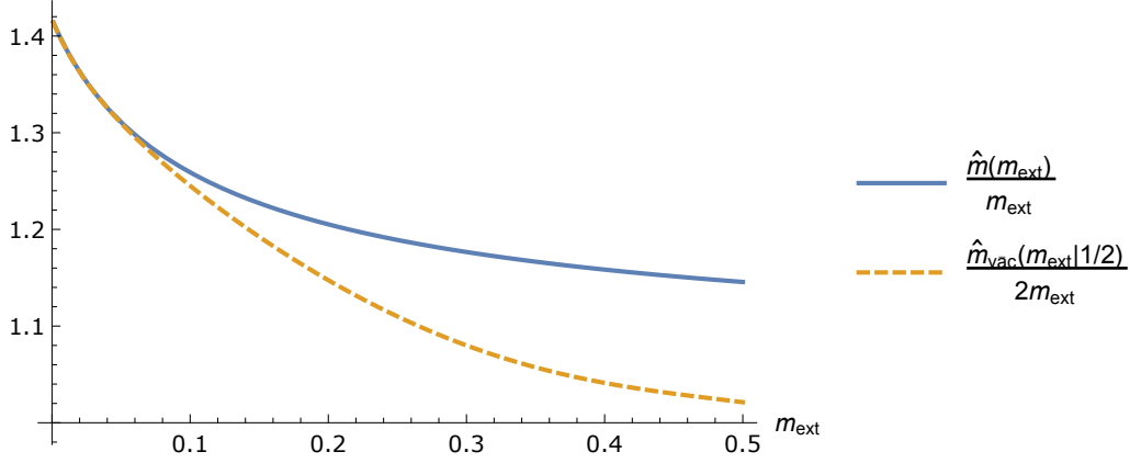
Figure 3.2: The ratios \frac{\hat{m}(m_{\text{ext}})}{m_{\text{ext}}} and \frac{\hat{m}_{\text{vac}}(m_{\text{ext}}|1/2)}{2m_{\text{ext}}} as functions of the external weight m_{\text{ext}} . See (3.22) and (3.26) for definitions.
