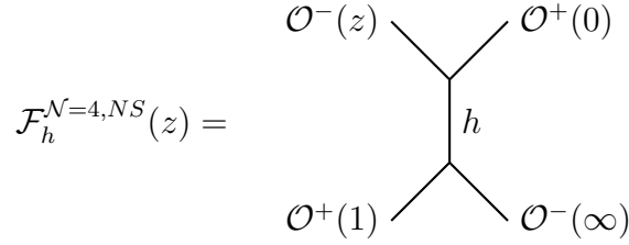
Figure 2.2: The chiral-anti-chiral c = 6 NS \mathcal{N} = 4 superconformal block with external BPS primaries \mathcal{O}^\pm and intermediate non-BPS primary of weight h .
