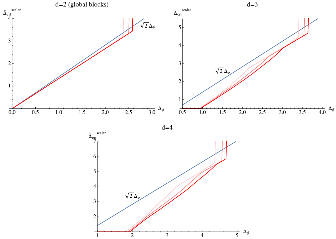
Figure 2.8: Upper bounds on \widehat{\Delta}_{crt}^{scalar} as a function of \Delta_\phi in 2 dimensions (using global conformal blocks), 3 dimensions, and 4 dimensions. The blue line shows the analytic bound \sqrt{2}\Delta_\phi on \widehat{\Delta}_{crt} . The red bounds are computed numerically with derivative order 12, 20, 28, with the darkest line and strongest bound corresponding to derivative order 28. For \Delta_\phi \lesssim 1 in 3d and \Delta_\phi \lesssim 2 in 4d, the red bounds meet at the unitary bounds, thus giving universal OPE bounds in this range of \Delta_\phi .
