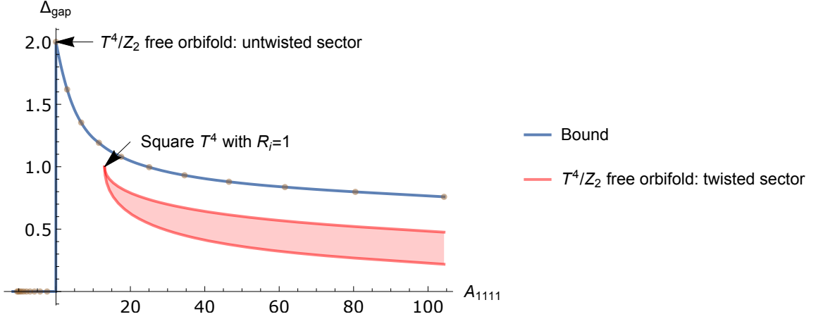
Figure 2.6: The solid line shows the upper bound \widehat{\Delta}_{gap} on the gap versus the integrated four-point function A_{1111} , at 20 derivative order, which we observe to already stabilize with increment of the derivative order in the range of A_{1111} shown here; the dots are the actual data points. The minimal A_{1111} and maximal gap are simultaneously saturated by an untwisted sector correlator at the free orbifold point. The shaded region represents the gap in the OPE of twist fields at a fixed point of T^4/\mathbb{Z}_2 with a rectangular T^4 , where the minimal A_{1111} and maximal gap are achieved by a square T^4 at radii R_i = 1 ( 1/\sqrt{2} times the self-dual radius).
