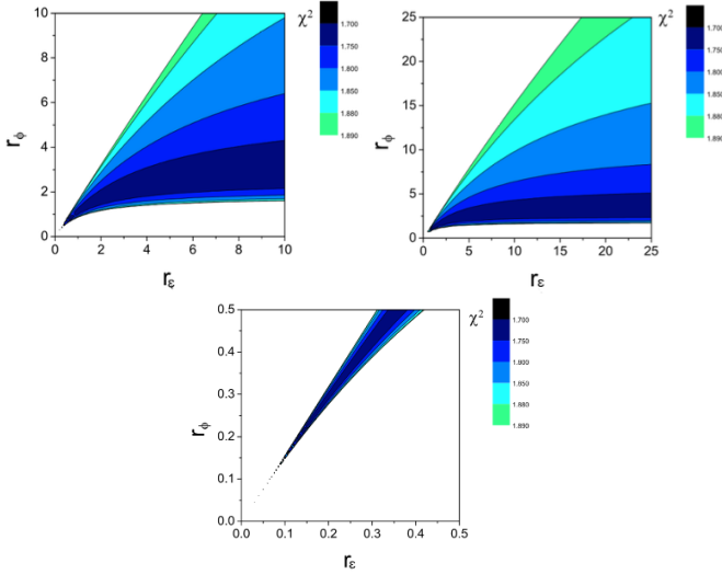
Fig. 1. Reduced \chi^2 in different regions of the parameter space r_\phi – r_\varepsilon (in AU). Regions with darker colors provide a better fit.
