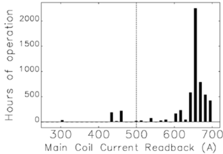
Figure 2: Histogram showing the SCU0 magnet operational current.
