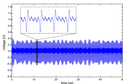
Figure 8: Signal obtained from BPM with 50 \mu s, and it's clearly that main bunch has a larger voltage compared with the satellite bunch.
