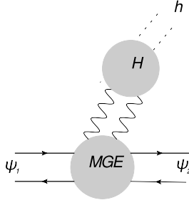
Fig. 1. Hidden-flavor amplitude \psi_1 \rightarrow \psi_2 h in the QCD multipole expansion approach. Here, \psi_1 and \psi_2 are the initial and final charmonium states, h light hadron(s). The two vertices are those of the multipole gluon emission (MGE) and hadronization (H).
